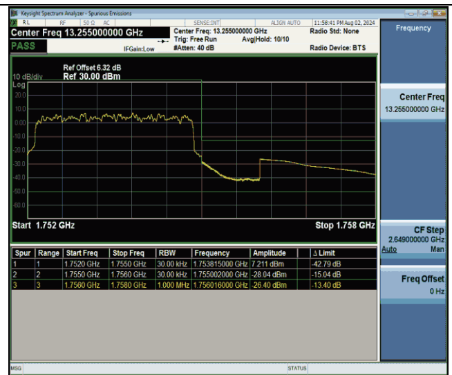
Band4_3MHz_QPSK_20385_15RB#0
