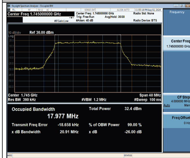
Band4-20MHz-QPSK-20300-100RB#0-PASS
