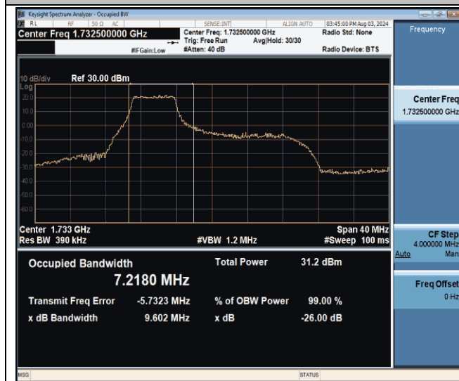
Band4-20MHz-16QAM-20175-27RB#0-PASS
