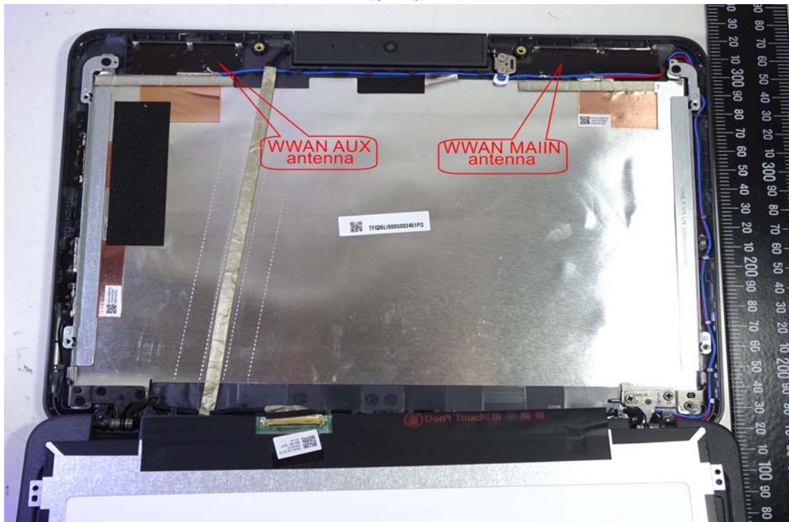
Antenna – 1
