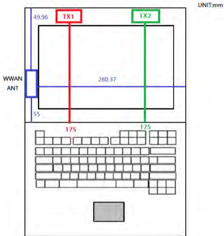
Fig.6 Antenna location
