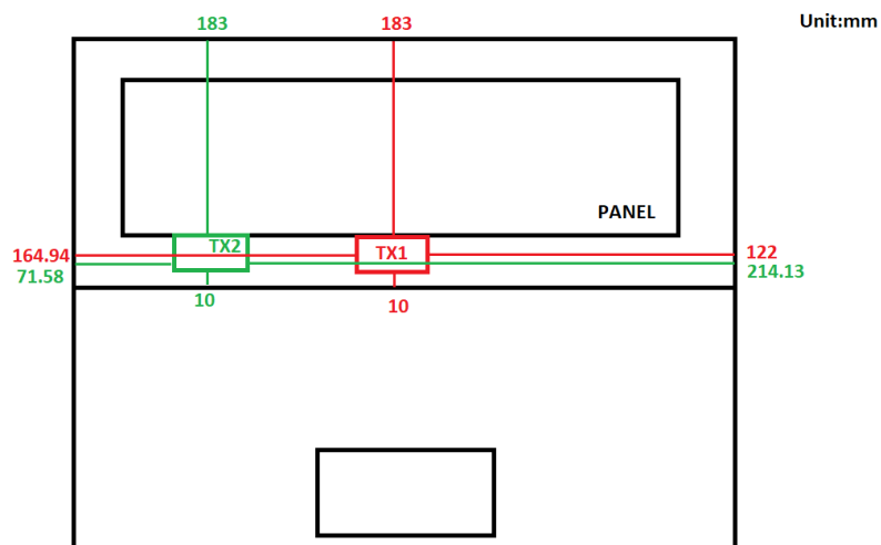
Fig.6 WWAN Antenna location
