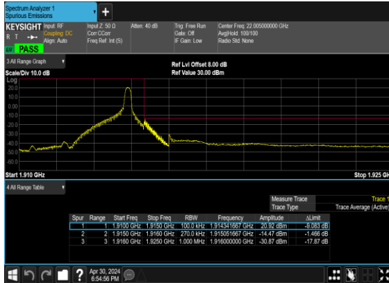
B66_N25(25M)_DFT-s-OFDM_BPSK_Edge_1RB_Right_High_CH
