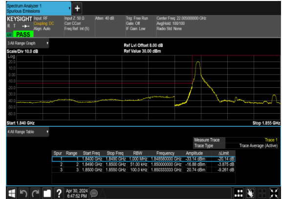
B66_N25(5M)_DFT-s- OFDM_QPSK_Edge_1RB_Left_Low_CH
