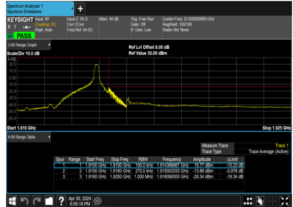
B66_N25(25M)_DFT-s-OFDM_QPSK_Edge_1RB_Right_High_CH
