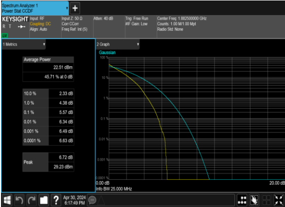
B66_N25(20M)_DFT-s-OFDM_QPSK_Outer_Full_Mid_CH
