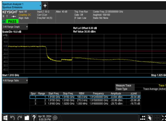
B66_N25(25M)_DFT-s-OFDM_BPSK_Outer_Full_High_CH
