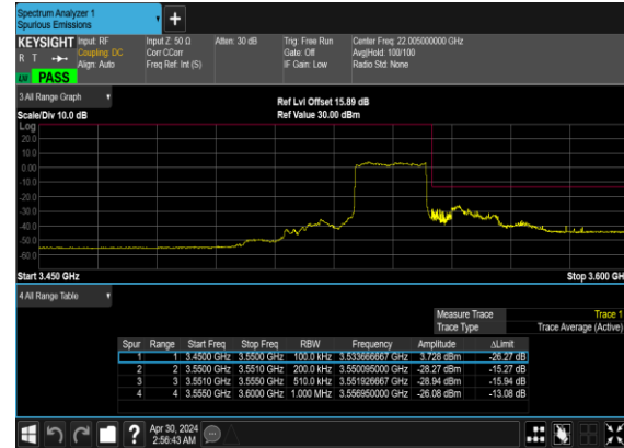
N77(20M)_DFT-s- OFDM_BPSK_Outer_Full_High_CH
