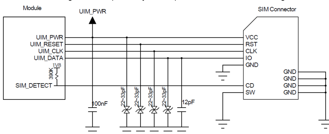
Figure 3-16 Reference circuit for N.C. SIM card slot
