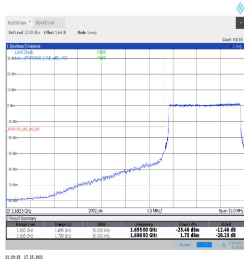
1-N70-15-5-L-6-CP-QPSK-Outer_Full-25@0-Ant1-seegraph-PASS-see graph
