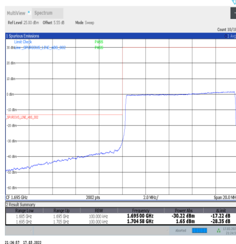
1-N70-15-10-L-6-CP-QPSK-Outer_Full-52@0-Ant1-seegraph-PASS-see graph
