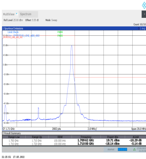
1-N70-15-10-H-2-DFT-PI2BPSK-Edge_1RB_Right-1 @51-Ant1-seegraph-PASS-see graph
