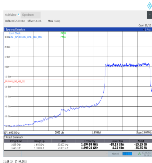
1-N70-15-5-L-3-DFT-PI2BPSK-Outer_Full-25@0-Ant1-seegraph-PASS-see graph
