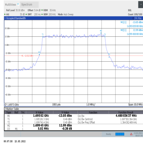
1-N70-15-5-L-2-DFT-PI2BPSK-Outer_Full-25@0-An t1-4.48-5.020-≤5-PASS
