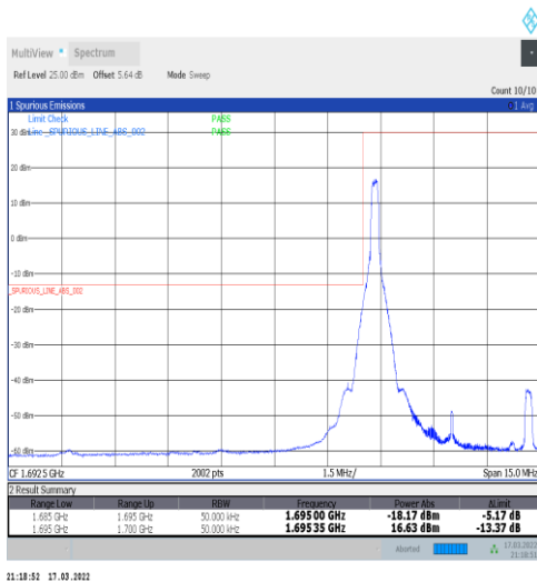
1-N70-15-5-L-1-DFT-PI2BPSK-Edge_1RB_Left-1@0-Ant1-seegraph-PASS-see graph
