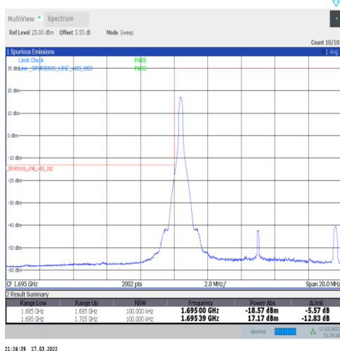
1-N70-15-10-L-4-CP-QPSK-Edge_1RB_Left-1@0-Ant1-seegraph-PASS-see graph
