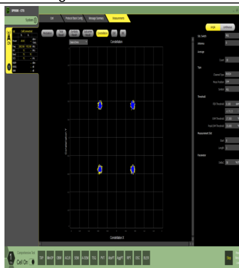
1-N70-15-15-M-6-CP-QPSK-Outer_Full-79@0-Ant1 -see graph-PASS
