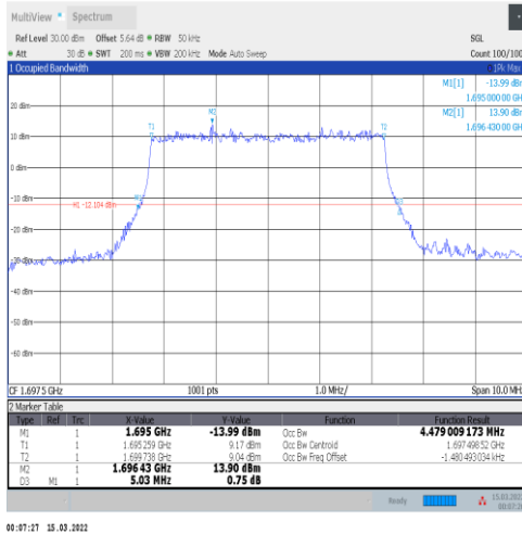
1-N70-15-5-L-1-DFT-QPSK-Outer_Full-25@0-Ant1-4 4.79-5.030-≤5-PASS
