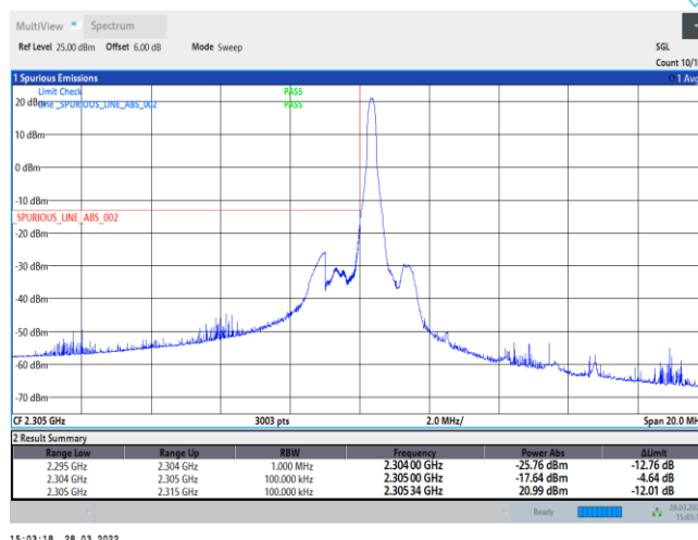
Band30-5MHz-QPSK-27685-25RB#0
