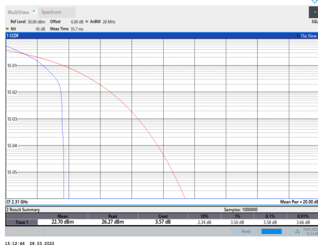
Band30-10MHz-16QAM-27710-1RB#0
