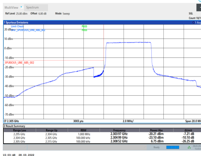
Band30-5MHz-QPSK-27685-25RB#0
