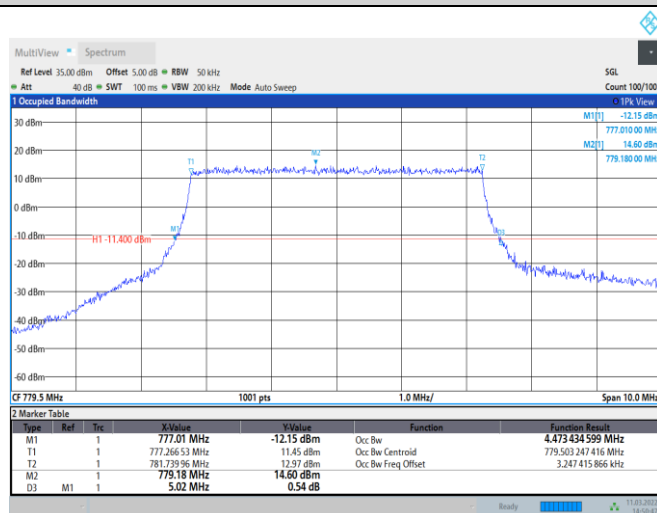
Band13-5MHz-QPSK-23205-25RB#0
