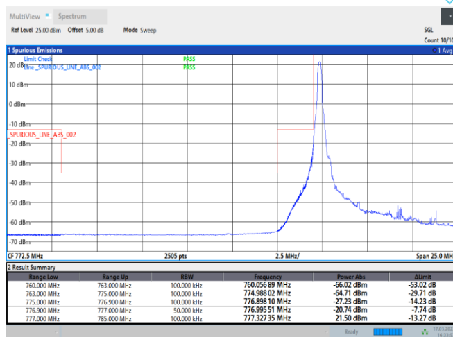
Band13-5MHz-QPSK-23205-25RB#0
