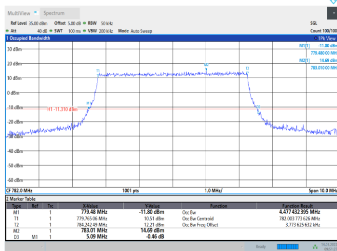
Band13-5MHz-QPSK-23230-25RB#0
