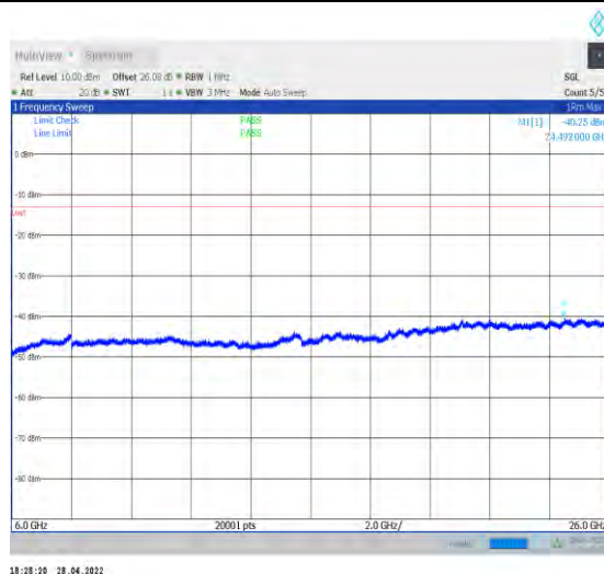
1-N77-3700-3980--30-100-H-1-DFT-QPSK-Edge_1R B_Left-1@0-6000-26000-Ant2--40.25--13-PASS
