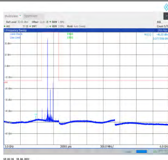
1-N77-3700-3980--30-100-M-1-DFT-QPSK-Edge_1R B_Left-1@0-3000-6000-Ant2--46.35--13-PASS
