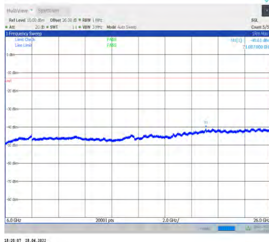
1-N77-3700-3980--30-100-L-1-DFT-QPSK-Edge_1R B_Left-1@0-6000-26000-Ant1--40.61--13-PASS
