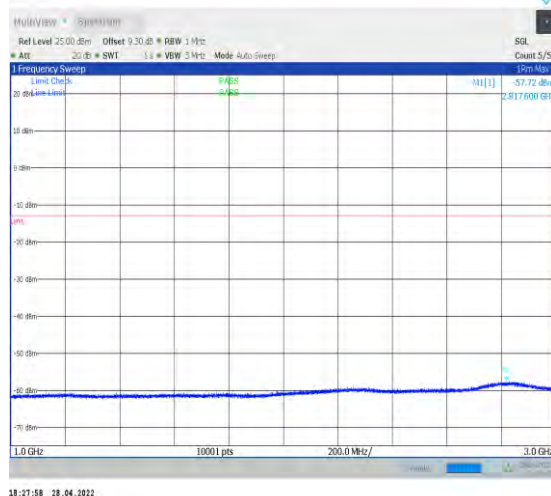
1-N77-3700-3980--30-100-H-1-DFT-QPSK-Edge_1R B_Left-1@0-1000-3000-Ant2--57.72--13-PASS
