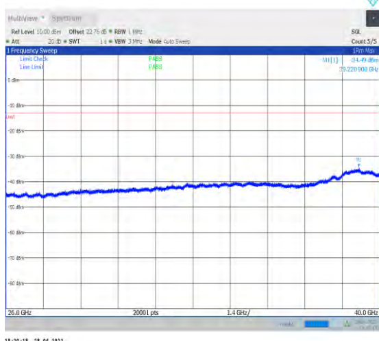
1-N77-3700-3980--30-100-L-1-DFT-QPSK-Edge_1R B_Left-1@0-26000-40000-Ant1--34.49--13-PASS
