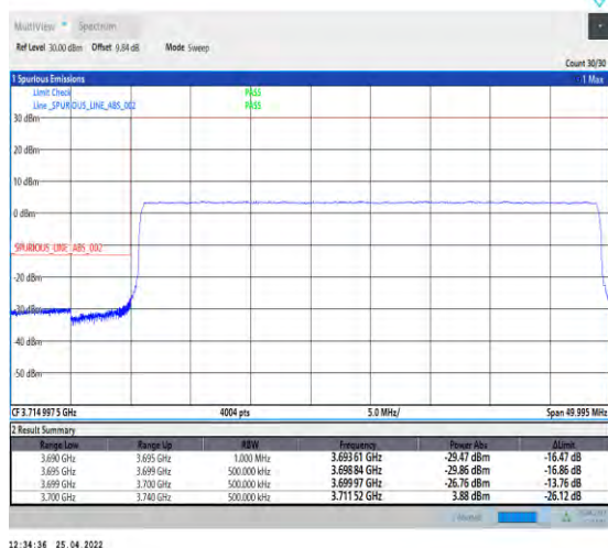
1-N77-3700-3980--30-40-L-6-CP-QPSK-Outer_Full-106@0-Ant1-PASS-see graph
