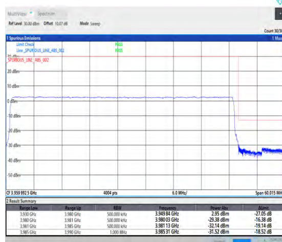
1-N77-3700-3980--30-50-H-6-CP-QPSK-Outer_Fu ll-133@0-Ant2-PASS-see graph
