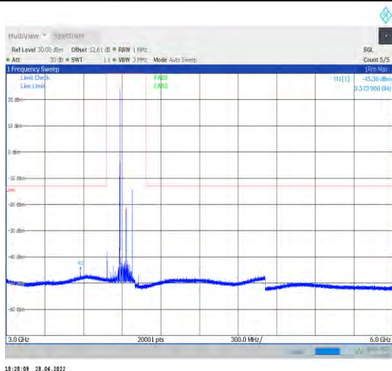
1-N77-3700-3980--30-100-H-1-DFT-QPSK-Edge_1R B_Left-1@0-3000-6000-Ant2--45.36--13-PASS
