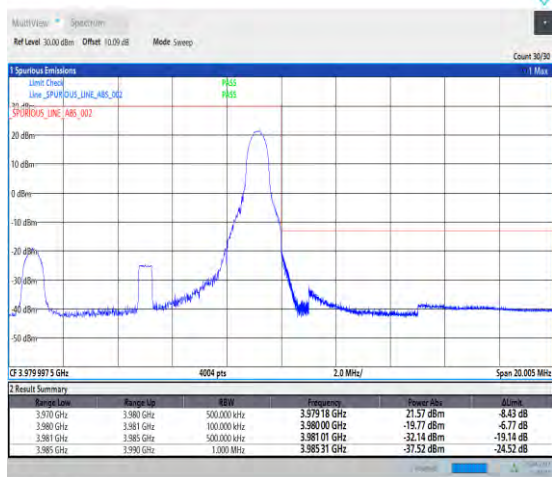
1-N77-3700-3980--30-10-H-5-CP-QPSK-Edge_1RB_Ri ght-1@23-Ant2-PASS-see graph
