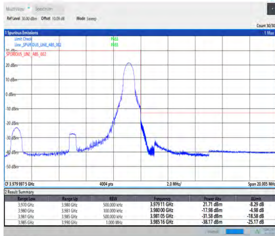
1-N77-3700-3980--30-10-H-5-CP-QPSK-Edge_1RB _Right-1@23-Ant1-PASS-see graph
