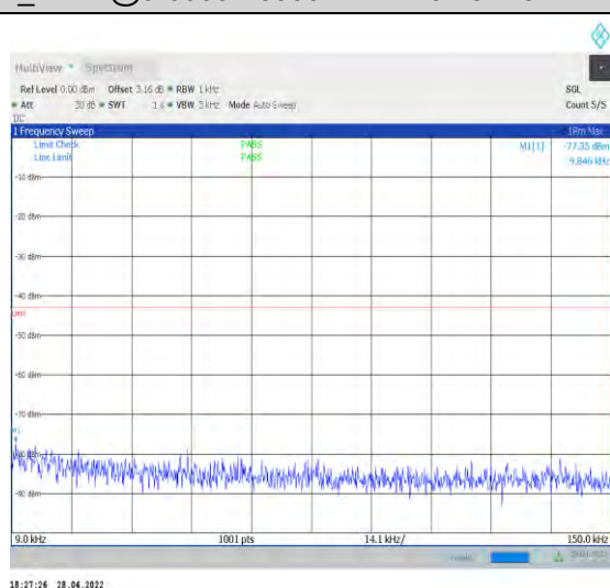
1-N77-3700-3980--30-100-H-1-DFT-QPSK-Edge_1R B_Left-1@0-0.009-0.15-Ant2--77.35--43-PASS
