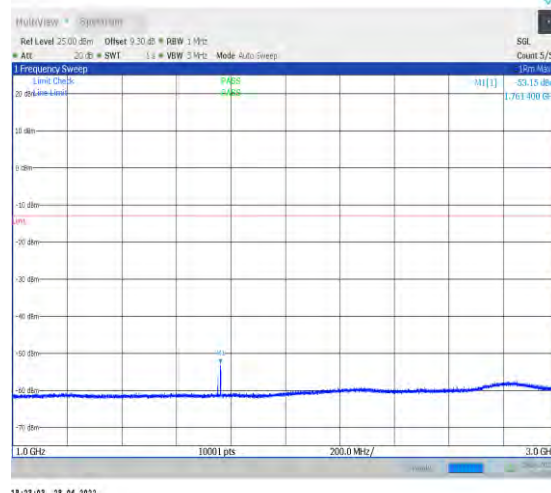
1-N77-3700-3980--30-100-H-1-DFT-QPSK-Edge_1R B_Left-1@0-1000-3000-Ant1--53.15--13-PASS
