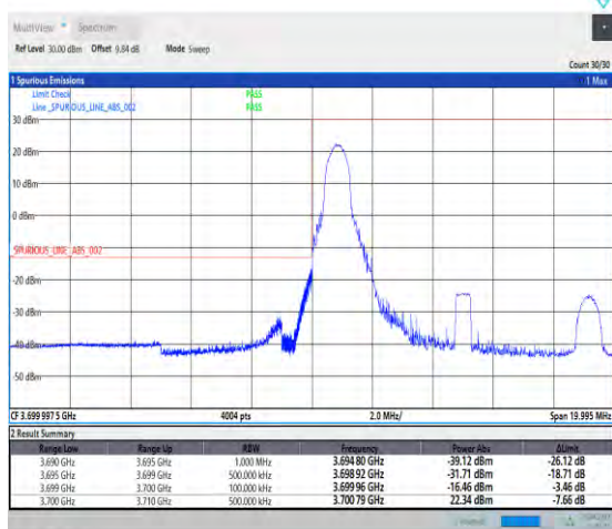
1-N77-3700-3980--30-10-L-4-CP-QPSK-Edge_1RB_Le ft-1@0-Ant2-PASS-see graph
