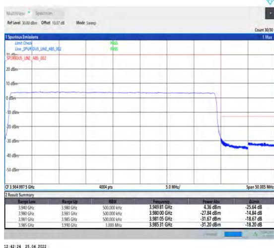
1-N77-3700-3980--30-40-H-6-CP-QPSK-Outer_Full-106@0-Ant1-PASS-see graph
