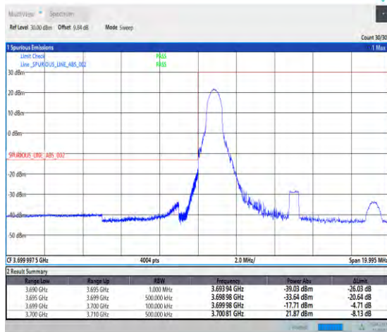
1-N77-3700-3980--30-10-L-4-CP-QPSK-Edge_1RB _Left-1@0-Ant1-PASS-see graph
