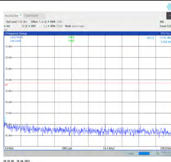
1-N77-3700-3980--30-100-M-1-DFT-QPSK-Edge_1R B_Left-1@0-0.009-0.15-Ant2--77.81--43-PASS
