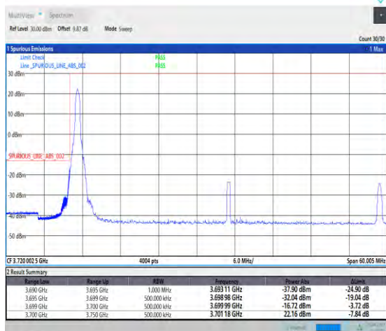
1-N77-3700-3980--30-50-L-4-CP-QPSK-Edge_1RB_Le ft-1@0-Ant2-PASS-see graph
