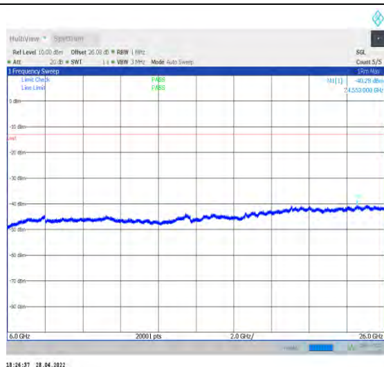
1-N77-3700-3980--30-100-M-1-DFT-QPSK-Edge_1R B_Left-1@0-6000-26000-Ant2--40.28--13-PASS
