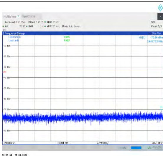
1-N77-3700-3980--30-100-M-1-DFT-QPSK-Edge_1R B_Left-1@0-0.15-30-Ant2--70.86--33-PASS
