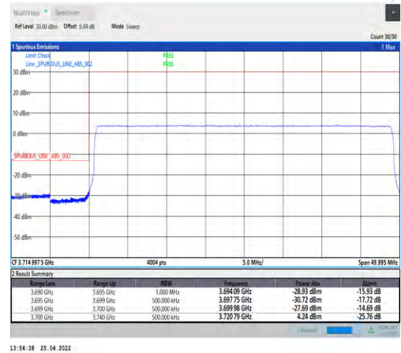
1-N77-3700-3980--30-40-L-6-CP-QPSK-Outer_Ful I-106@0-Ant2-PASS-see graph
