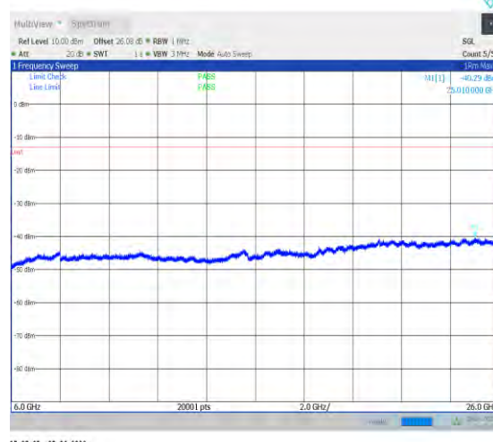
1-N77-3700-3980--30-100-H-1-DFT-QPSK-Edge_1R B_Left-1@0-6000-26000-Ant1--40.29--13-PASS
