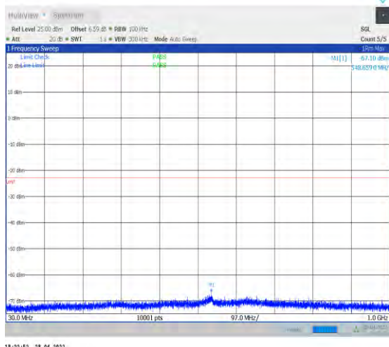
1-N77-3700-3980--30-100-H-1-DFT-QPSK-Edge_1R B_Left-1@0-30-1000-Ant1--67.10--23-PASS
