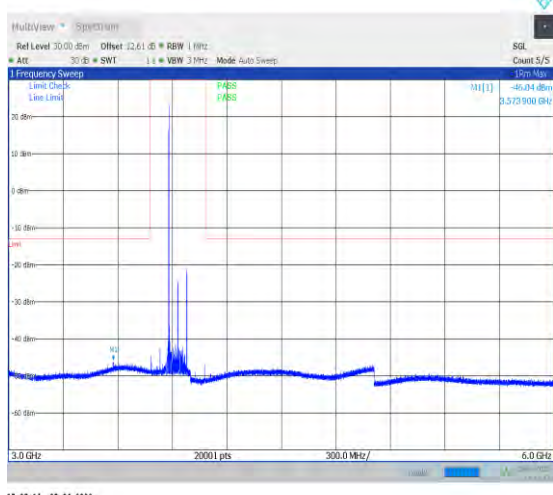
1-N77-3700-3980--30-100-H-1-DFT-QPSK-Edge_1R B_Left-1@0-3000-6000-Ant1--46.04--13-PASS
