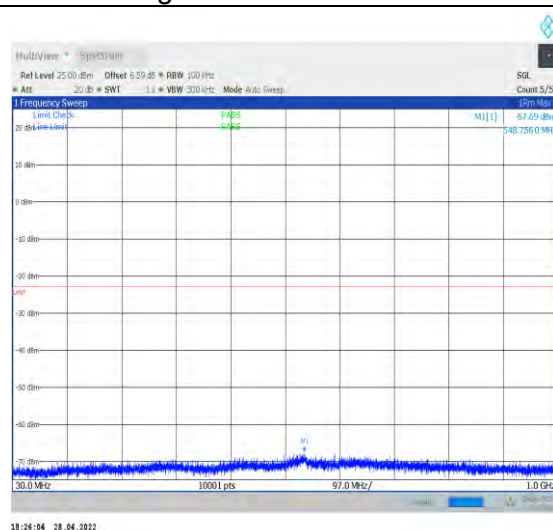
1-N77-3700-3980--30-100-M-1-DFT-QPSK-Edge_1R B_Left-1@0-30-1000-Ant2--67.69--23-PASS
