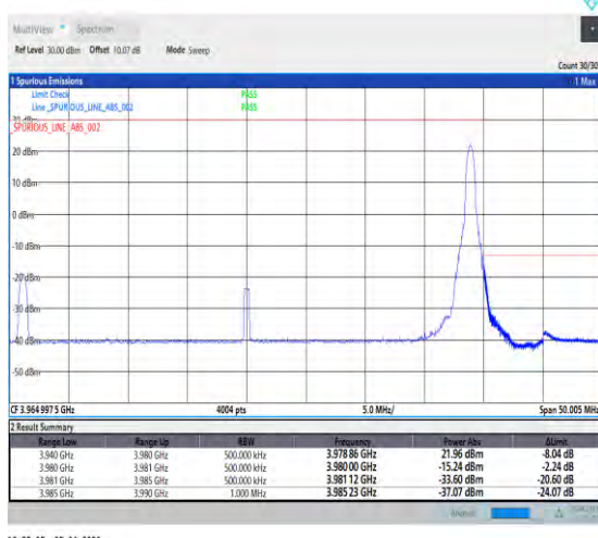
1-N77-3700-3980--30-40-H-5-CP-QPSK-Edge_1RB_Ri ght-1@105-Ant2-PASS-see graph
