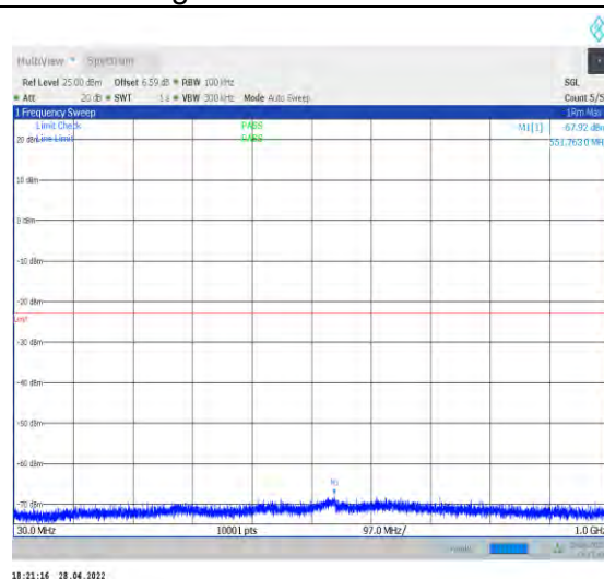
1-N77-3700-3980--30-100-M-1-DFT-QPSK-Edge_1R B_Left-1@0-30-1000-Ant1--67.92--23-PASS
