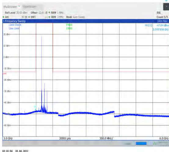
1-N77-3700-3980--30-100-L-1-DFT-QPSK-Edge_1R B_Left-1@0-3000-6000-Ant1--47.04--13-PASS
