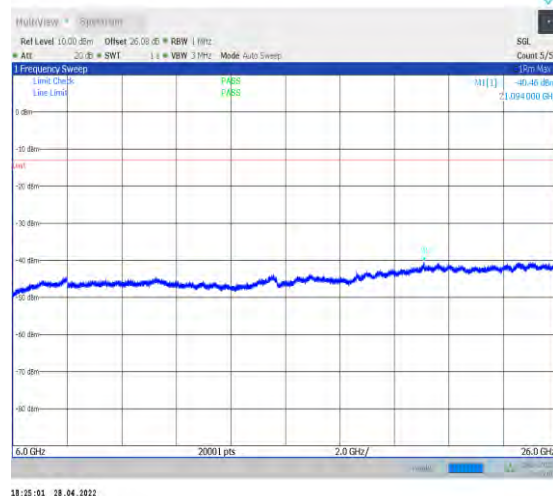
1-N77-3700-3980--30-100-L-1-DFT-QPSK-Edge_1R B_Left-1@0-6000-26000-Ant2--40.46--13-PASS
