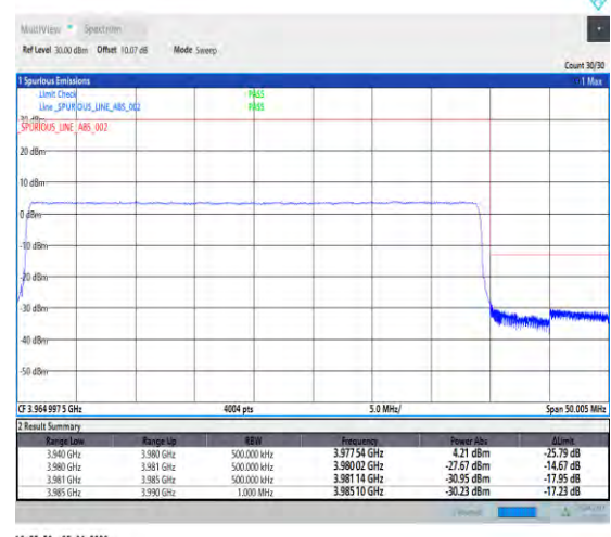
1-N77-3700-3980--30-40-H-6-CP-QPSK-Outer_Fu ll-106@0-Ant2-PASS-see graph
