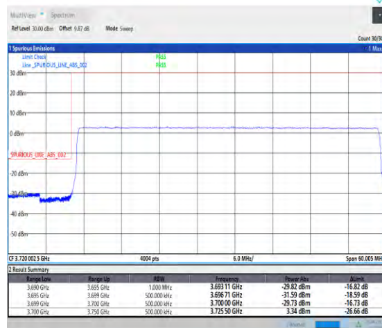
1-N77-3700-3980--30-50-L-6-CP-QPSK-Outer_Ful I-133@0-Ant2-PASS-see graph
