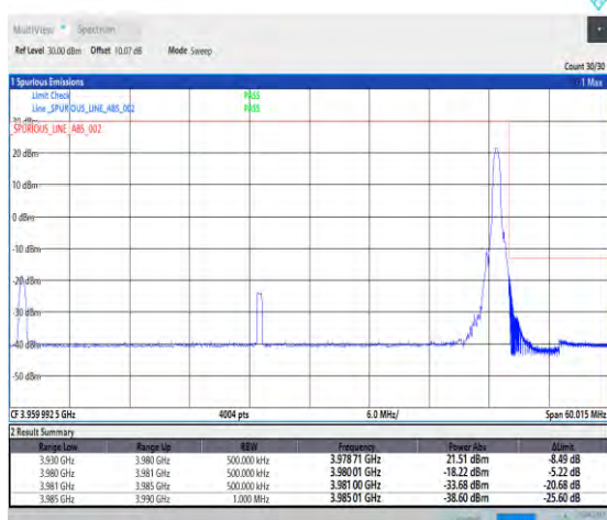
1-N77-3700-3980--30-50-H-5-CP-QPSK-Edge_1RB_Ri ght-1@132-Ant2-PASS-see graph
