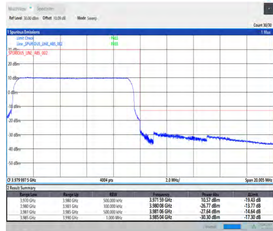
1-N77-3700-3980--30-10-H-6-CP-QPSK-Outer_Full-2 4@0-Ant1-PASS-see graph
