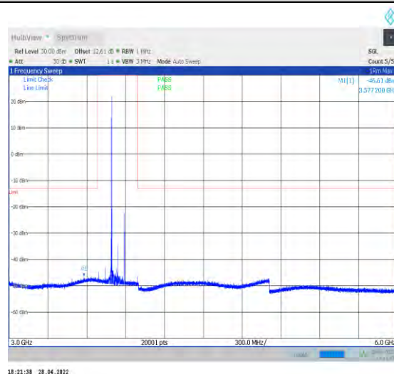
1-N77-3700-3980--30-100-M-1-DFT-QPSK-Edge_1R B_Left-1@0-3000-6000-Ant1--46.61--13-PASS
