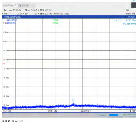
1-N77-3700-3980--30-100-H-1-DFT-QPSK-Edge_1R B_Left-1@0-30-1000-Ant2--67.61--23-PASS
