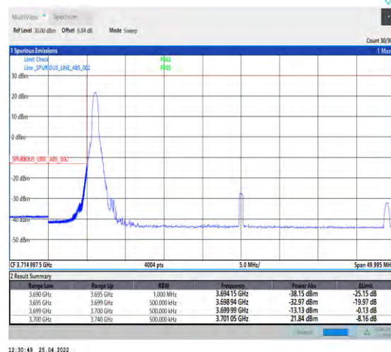
1-N77-3700-3980--30-40-L-4-CP-QPSK-Edge_1RB_Left-1@0-Ant1-PASS-see graph
