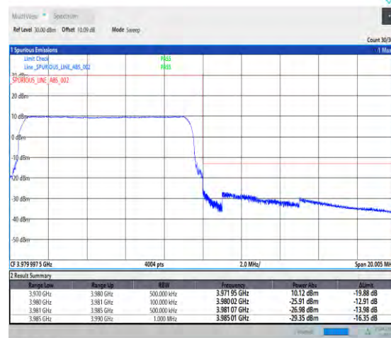
1-N77-3700-3980--30-10-H-6-CP-QPSK-Outer_Fu ll-24@0-Ant2-PASS-see graph
