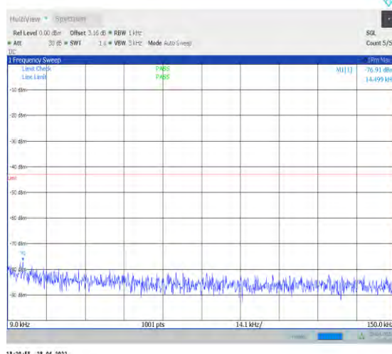
1-N77-3700-3980--30-100-M-1-DFT-QPSK-Edge_1R B_Left-1@0-0.009-0.15-Ant1--76.91--43-PASS
