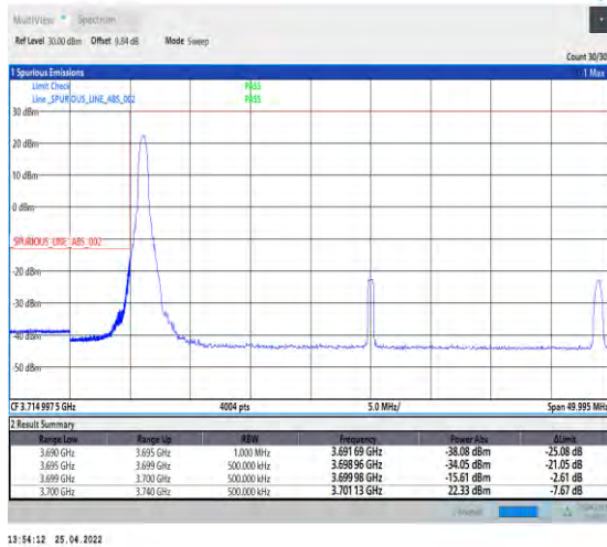
1-N77-3700-3980--30-40-L-4-CP-QPSK-Edge_1RB_Le ft-1@0-Ant2-PASS-see graph
