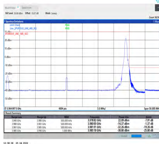
1-N77-3700-3980--30-40-H-5-CP-QPSK-Edge_1RB_Right-1@105-Ant1-PASS-see graph
