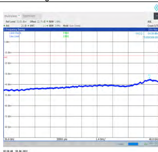
1-N77-3700-3980--30-100-M-1-DFT-QPSK-Edge_1R B_Left-1@0-26000-40000-Ant2--34.58--13-PASS
