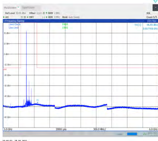
1-N77-3450-3550--30-100-H-1-DFT-QPSK-Edge_1R B_Left-1@0-3000-6000-Ant1--46.93--13-PASS
