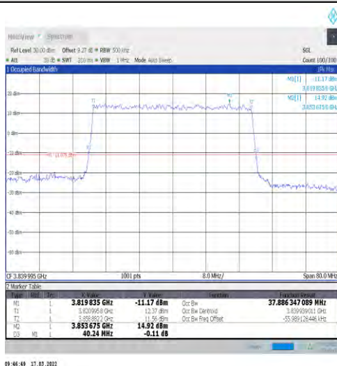
1-N77-3700-3980-30-40-M-6-CP-QPSK-Outer_Full-1 06@0-Ant1-37.886-40.240-≤40-PASS
