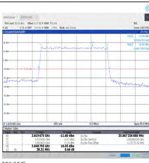
1-N77-3700-3980-30-40-M-4-DFT-64QAM-Outer_Ful I-100@0-Ant1-35.867-38.320-≤40-PASS
