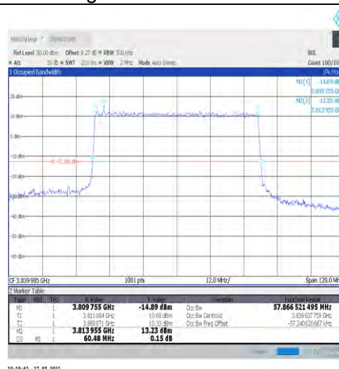
1-N77-3700-3980-30-60-M-7-CP-16QAM-Out_162@0-Ant1-57.867-60.480-≤60-PASS
