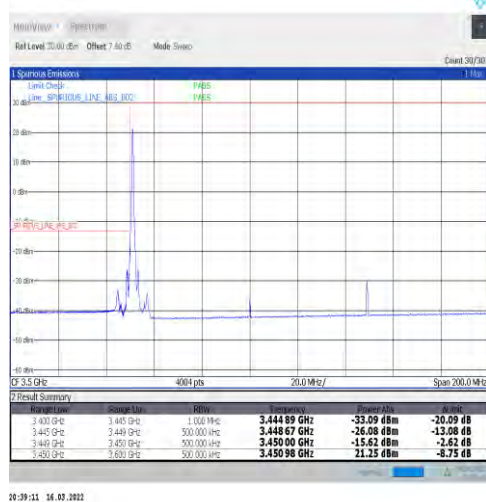
1-N77-3450-3550-30-100-L-4-CP-QPSK-Edge_1RB_L_eft-1@0-Ant1-PASS-see graph
