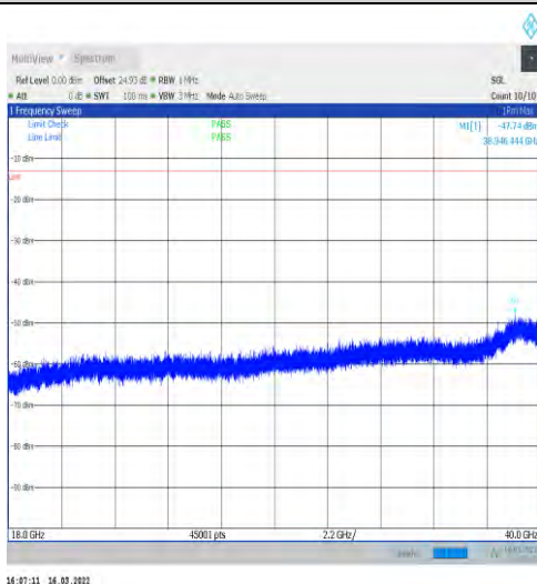
1-N77-3450-3550-30-100-L-1-DFT-PI2BPSK-Inner_1 RB_Left-1@1-18000-40000-Ant1--47.74--13-PASS
