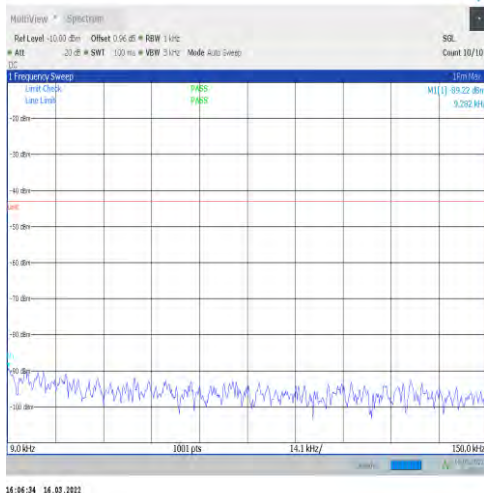
1-N77-3450-3550-30-100-L-1-DFT-PI2BPSK-Inner_1 RB_Left-1@1-0.009-0.15-Ant1--89.22--43-PASS
