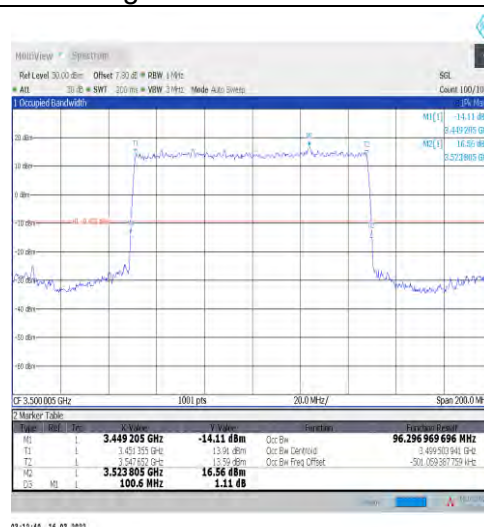
1-N77-3450-3550-30-100-H-2-DFT-PI2BPSK-Outet_Full -270@0-Ant1-96.297-100.600-≤100-PASS
