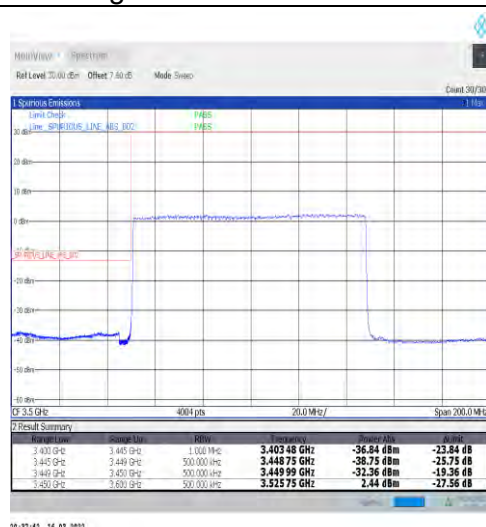
1-N77-3450-3550-30-100-L-3-DFT-PI2BPSK-Outer_Full-270@0-Ant1-PASS-see graph
