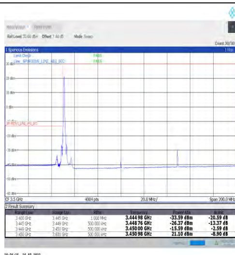
1-N77-3450-3550-30-100-L-1-DFT-PI2BPSK-Edge_1R_B_Left-1@0-Ant1-PASS-see graph
