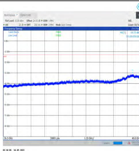
1-N77-3450-3550-30-100-L-1-DFT-PI2BPSK-Inner_1 RB_Left-1@1-26500-40000-Ant1--30.75--13-PASS
