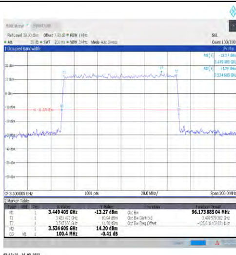
1-N77-3450-3550-30-100-H-3-DFT-16QAM-Outet_Full -270@0-Ant1-96.174-100.400-≤100-PASS
