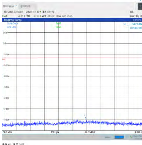
1-N77-3450-3550-30-100-L-1-DFT-PI2BPSK-Inner_1 RB_Left-1@1-30-1000-Ant1--69.24--23-PASS
