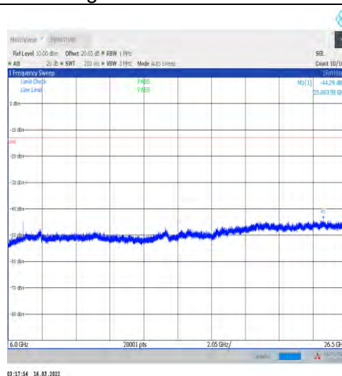
1-N77-3450-3550-30-100-L-1-DFT-PI2BPSK-Inner_1 RB_Left-1@1-6000-26500-Ant1--44.28--13-PASS
