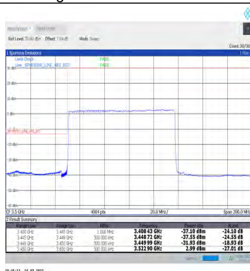
1-N77-3450-3550-30-90-L-3-DFT-PI2BPSK-Outer_Full-240@0-Ant1-PASS-see graph
