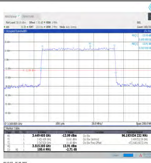
1-N77-3450-3550-30-100-H-4-DFT-64QAM-Outet_Full -270@0-Ant1-96.193-100.400-≤100-PASS
