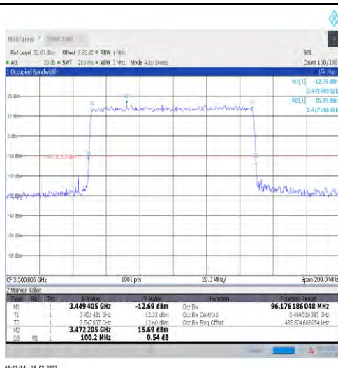
1-N77-3450-3550-30-100-H-1-DFT-QPSK-Outet_Full -270@0-Ant1-96.176-100.200-≤100-PASS
