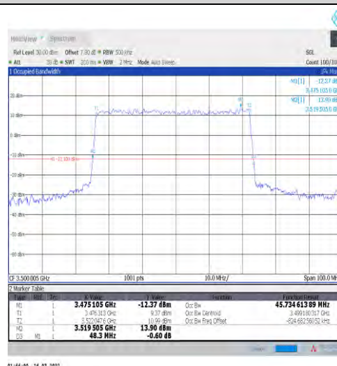
1-N77-3450-3550-30-50-M-4-DFT-64QAM-Outer_Full-128@0-Ant1-45.735-48.300-≤50-PASS
