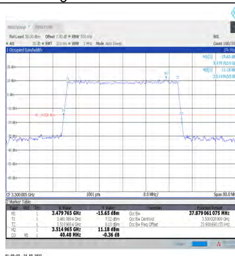
1-N77-3450-3550-30-40-M-9-CP-256QAM-Outer_Fu II-106@0-Ant1-37.879-40.480-≤40-PASS
