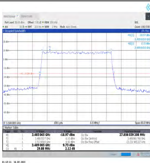
1-N77-3450-3550-30-30-M-9-CP-256QAM-Outer_Ful-I-78@0-Ant1-27.856-29.880-≤30-PASS
