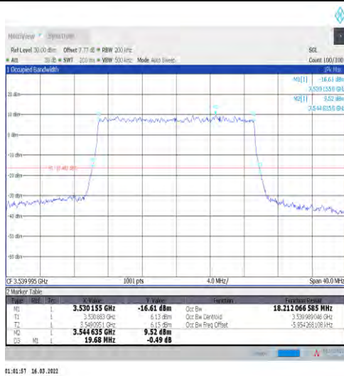
1-N77-3450-3550-30-20-H-9-CP-256QAM-Outer_Ful I-51@0-Ant1-18.212-19.680-≤20-PASS
