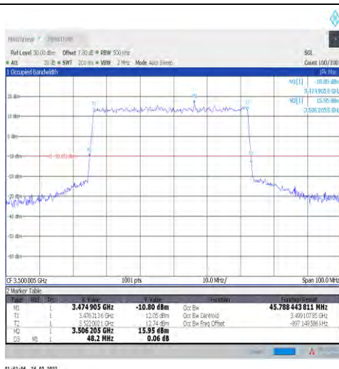
1-N77-3450-3550-30-50-M-1-DFT-QPSK-Outer_Full-128@0-Ant1-45.788-48.200-≤50-PASS
