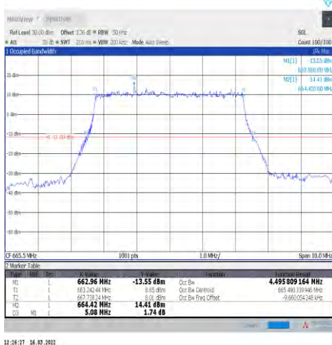
1-N71-15-5-L-1-DFT-QPSK-Outer_Full-25@0-Ant1-4 .496-5.080-≤5-PASS
