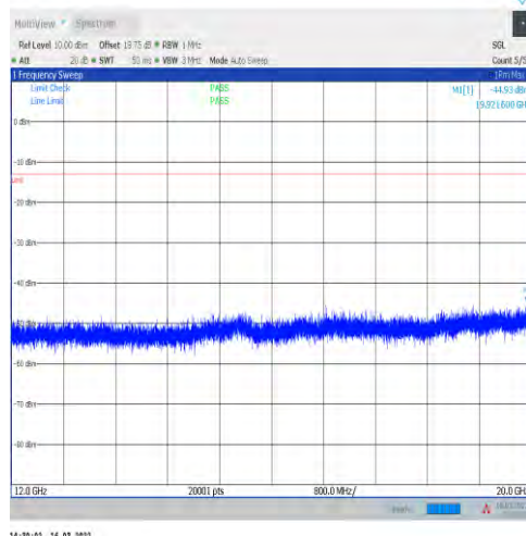
1-N71-15-20-H-1-DFT-PI2BPSK-Inner_1RB_Left-1@ 1-12000-20000-Ant1--44.93--13-PASS
