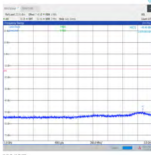
1-N71-15-20-H-1-DFT-PI2BPSK-Inner_1RB_Left-1@ 1-1000-3000-Ant1--48.46--13-PASS
