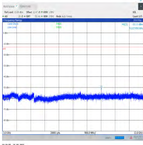
1-N71-15-20-H-1-DFT-PI2BPSK-Inner_1RB_Left-1 @1-3000-12000-Ant1--52.11--13-PASS
