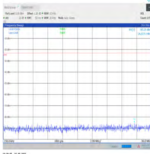
1-N71-15-20-H-1-DFT-PI2BPSK-Inner_1RB_Left-1@ 1-0.15-30-Ant1--85.25--23-PASS
