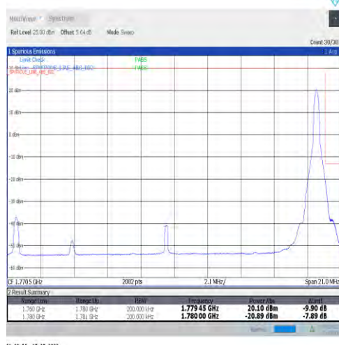
1-N66-15-20-H-5-CP-QPSK-Edge_1RB_Right-1@105-Ant1-seegraph-PASS-see graph
