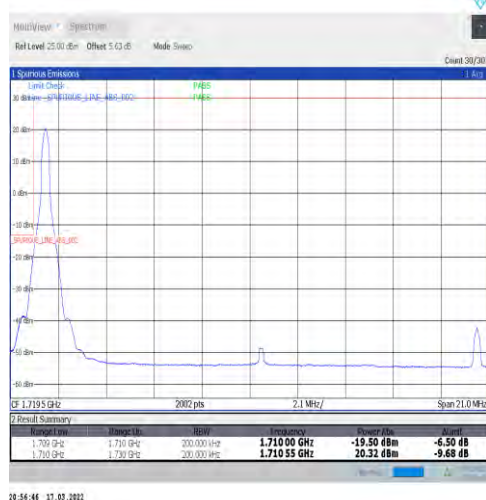
1-N66-15-20-L-4-CP-QPSK-Edge_1RB_Left-1@0-Ant1-seegraph-PASS-see graph
