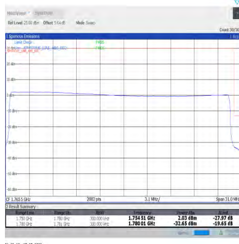
1-N66-15-30-H-6-CP-QPSK-Outer_Full-160@0-Ant1-seegraph-PASS-see graph
