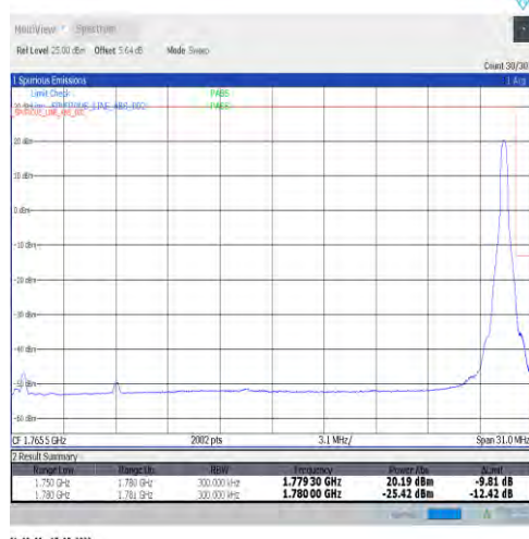
1-N66-15-30-H-5-CP-QPSK-Edge_1RB_Right-1@159-Ant1-seegraph-PASS-see graph
