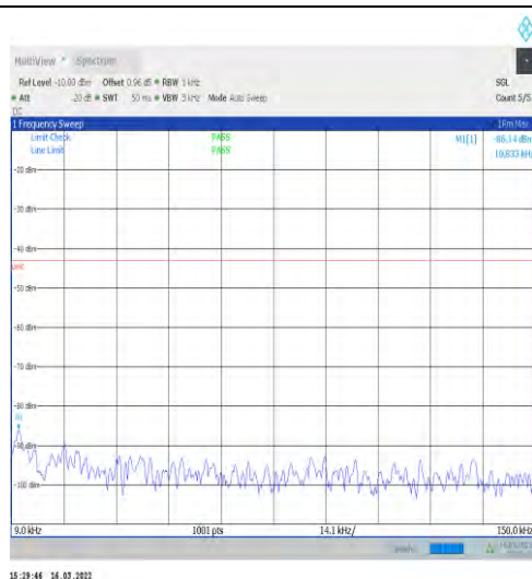
1-N66-15-40-H-1-DFT-PI2BPSK-Inner_1RB_Left-1 @1-0.009-0.15-Ant1--86.14--43-PASS
