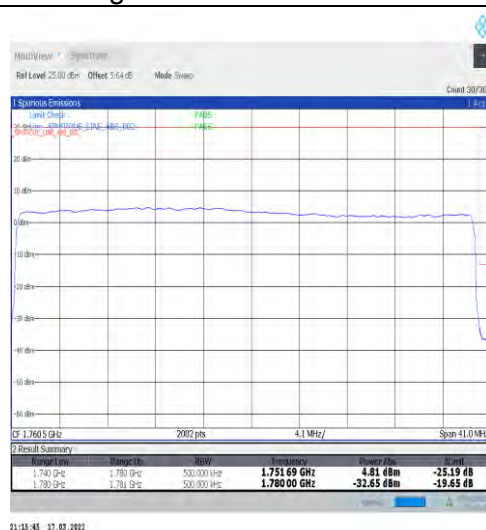
1-N66-15-40-H-3-DFT-PI2BPSK-Outer_Full-216@0-Ant1-seegraph-PASS-see graph
