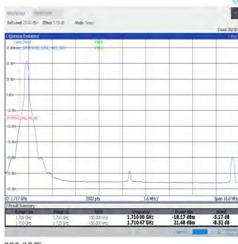
1-N66-15-15-L-1-DFT-PI2BPSK-Edge_1RB_Left-1@0-Ant1-seegraph-PASS-see graph
