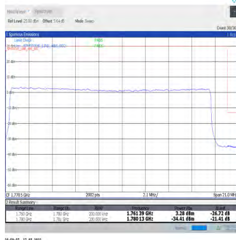
1-N66-15-20-H-3-DFT-PI2BPSK-Outer_Full-100@0-Ant1-seegraph-PASS-see graph
