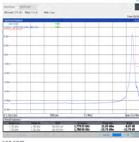
1-N66-15-30-H-2-DFT-PI2BPSK-Edge_1RB_Right-1@159-Ant1-seegraph-PASS-see graph
