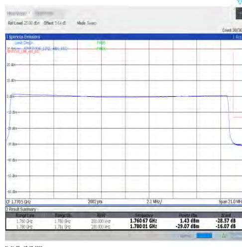
1-N66-15-20-H-6-CP-QPSK-Outer_Full-106@0-Ant1-seegraph-PASS-see graph
