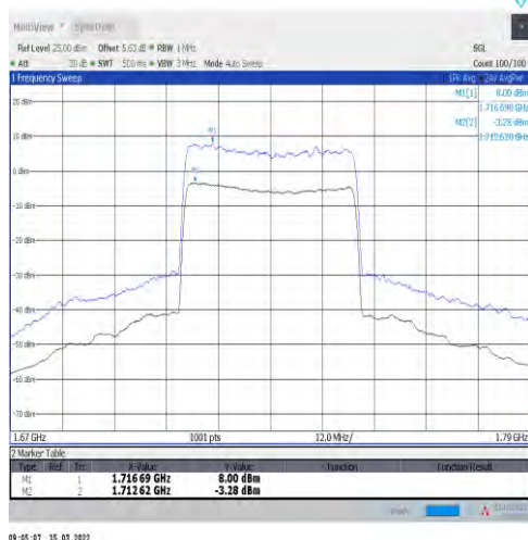
1-N66-15-40-L-1-DFT-256QAM-Outer_Full-216@0-A nt1-11.28-100%-0.00-11.28-PASS-≤13
