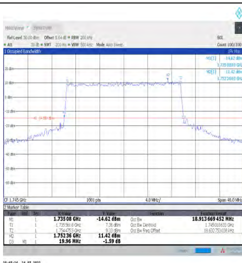
1-N66-15-20-M-7-CP-16QAM-Outer_Full-106@0-Ant 1-18.914-19.960-≤20-PASS
