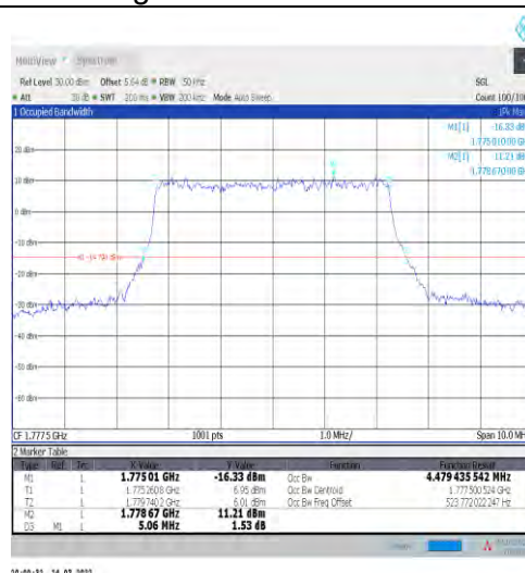
1-N66-15-5-H-4-DFT-64QAM-Outer_Full-25@0-Ant1 -4.479-5.060-≤5-PASS
