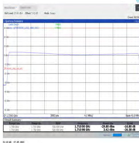
1-N66-15-40-L-6-CP-QPSK-Outer_Full-216@0-Ant1-seegraph-PASS-see graph
