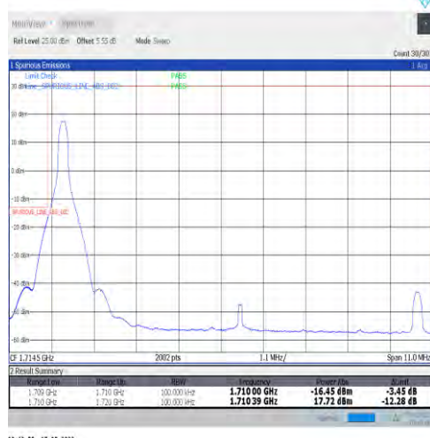
1-N66-15-10-L-4-CP-QPSK-Edge_1RB_Left-1@0-Ant1-seegraph-PASS-see graph
