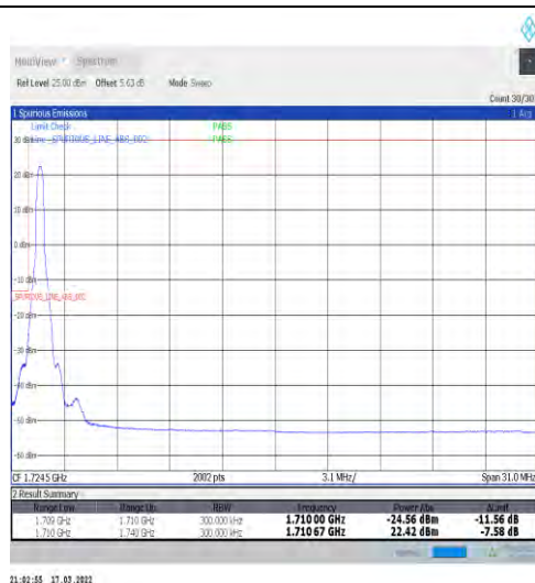
1-N66-15-30-L-1-DFT-PI2BPSK-Edge_1RB_Left-1@0-Ant1-seegraph-PASS-see graph
