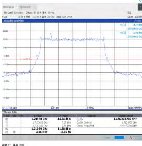
1-N66-15-5-L-3-DFT-16QAM-Outer_Full-25@0-Ant1-4 4.456-4.960-≤5-PASS
