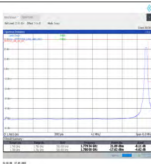
1-N66-15-40-H-2-DFT-PI2BPSK-Edge_1RB_Right-1@215-Ant1-seegraph-PASS-see graph
