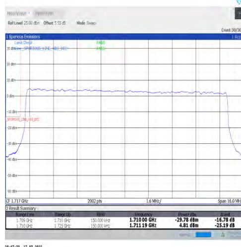
1-N66-15-15-L-3-DFT-PI2BPSK-Outer_Full-75@0-Ant1-seegraph-PASS-see graph
