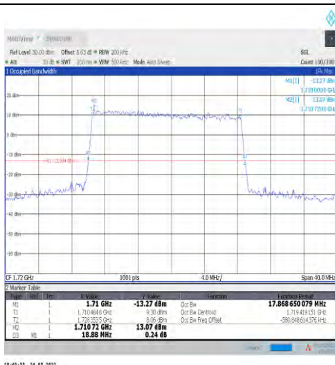
1-N66-15-20-L-4-DFT-64QAM-Outer_Full-100@0-A t1-17.869-18.880-≤20-PASS
