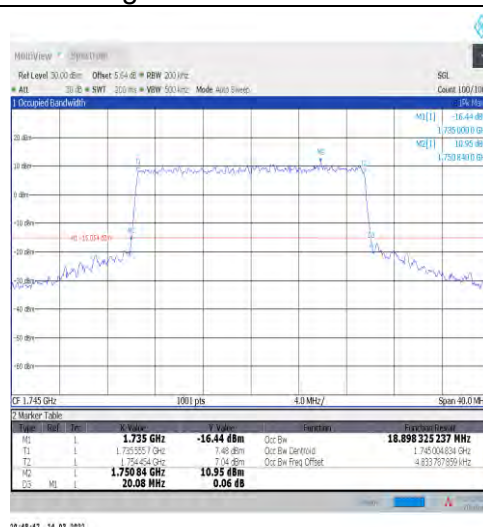
1-N66-15-20-M-8-CP-64QAM-Outer_Full-106@0-Ant 1-18.898-20.080-≤20-PASS
