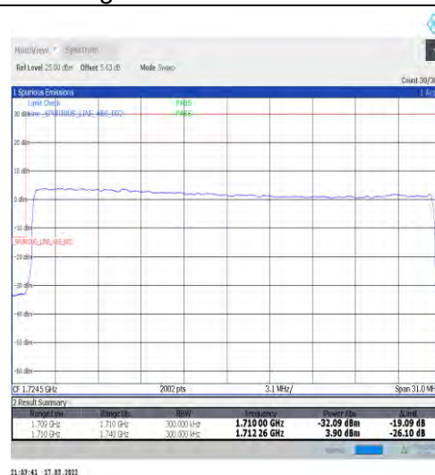
1-N66-15-30-L-3-DFT-PI2BPSK-Outer_Full-160@0-Ant1-seegraph-PASS-see graph
