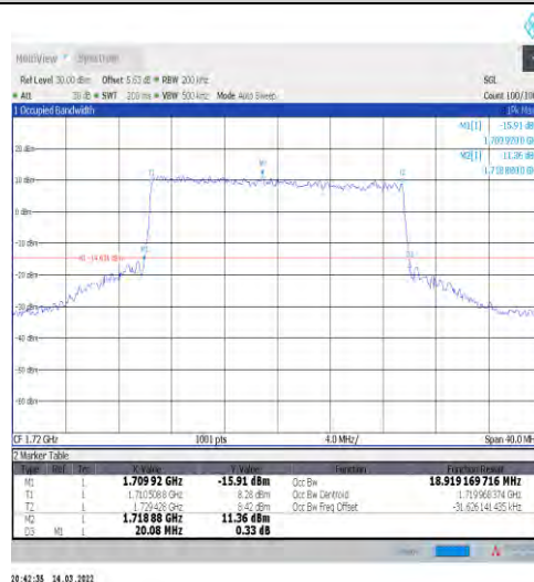
1-N66-15-20-L-7-CP-16QAM-Outer_Full-106@0-Ant 1-18.919-20.080-≤20-PASS
