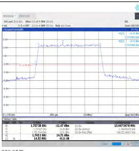
1-N66-15-15-M-2-DFT-PI2BPSK-Outer_Full-75@0-A nt1-13.447-14.520-≤15-PASS
