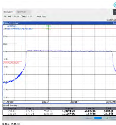
1-N66-15-5-L-6-CP-QPSK-Outer_Full-25@0-Ant1-seegraph-PASS-see graph
