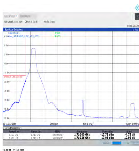
1-N66-15-5-L-1-DFT-PI2BPSK-Edge_1RB_Left-1@0-Ant1-seegraph-PASS-see graph
