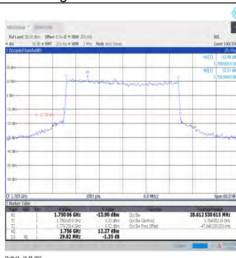
1-N66-15-30-H-8-CP-64QAM-Outer_Full-160@0-Ant 1-28.613-29.820-≤30-PASS
