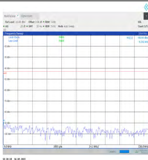
1-N66-15-40-M-1-DFT-PI2BPSK-Inner_1RB_Left-1 @ 1-0.009-0.15-Ant1--90.98--43-PASS
