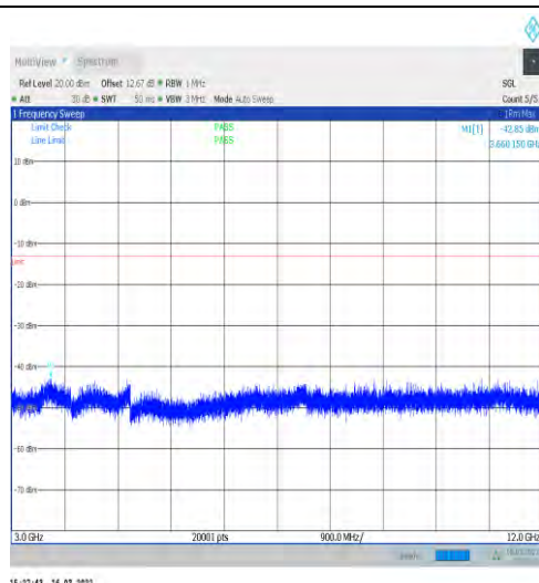
1-N66-15-40-L-1-DFT-PI2BPSK-Inner_1RB_Left-1@ 1-3000-12000-Ant1--42.85--13-PASS
