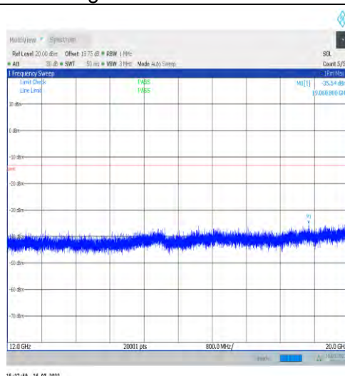
1-N66-15-40-L-1-DFT-PI2BPSK-Inner_1RB_Left-1@ 1-12000-20000-Ant1--35.54--13-PASS
