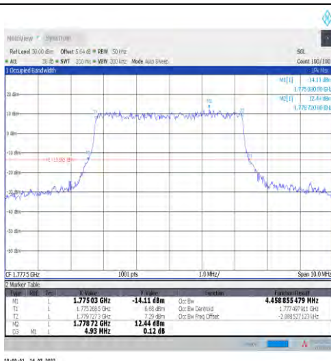
1-N66-15-5-H-3-DFT-16QAM-Outer_Full-25@0-Ant1 -4.459-4.930-≤5-PASS
