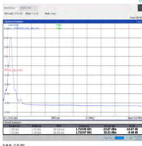
1-N66-15-30-L-4-CP-QPSK-Edge_1RB_Left-1@0-Ant1-seegraph-PASS-see graph
