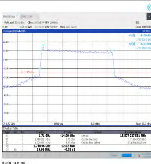
1-N66-15-20-L-6-CP-QPSK-Outer_Full-106@0-Ant1- 18.877-19.960-≤20-PASS
