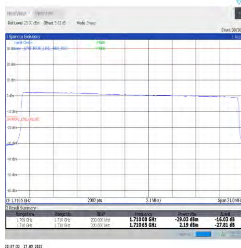
1-N66-15-20-L-6-CP-QPSK-Outer_Full-106@0-Ant1-seegraph-PASS-see graph
