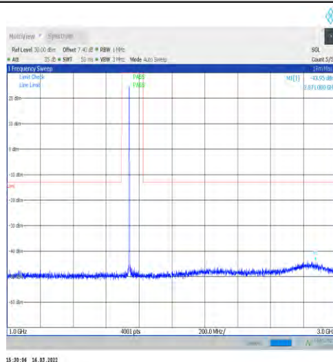
1-N66-15-40-H-1-DFT-PI2BPSK-Inner_1RB_Left-1@ 1-1000-3000-Ant1--43.95--13-PASS
