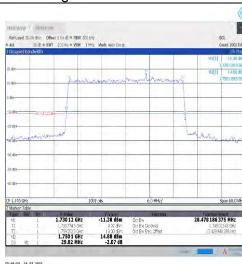
1-N66-15-30-M-1-DFT-QPSK-Outer_Full-160@0-Ant t1-28.478-29.820-≤30-PASS
