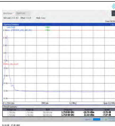
1-N66-15-40-L-1-DFT-PI2BPSK-Edge_1RB_Left-1@0-Ant1-seegraph-PASS-see graph
