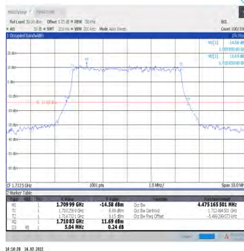
1-N66-15-5-L-4-DFT-64QAM-Outer_Full-25@0-Ant1-4 4.475-5.040-≤5-PASS
