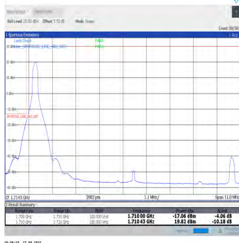
1-N66-15-10-L-1-DFT-PI2BPSK-Edge_1RB_Left-1@0-Ant1-seegraph-PASS-see graph
