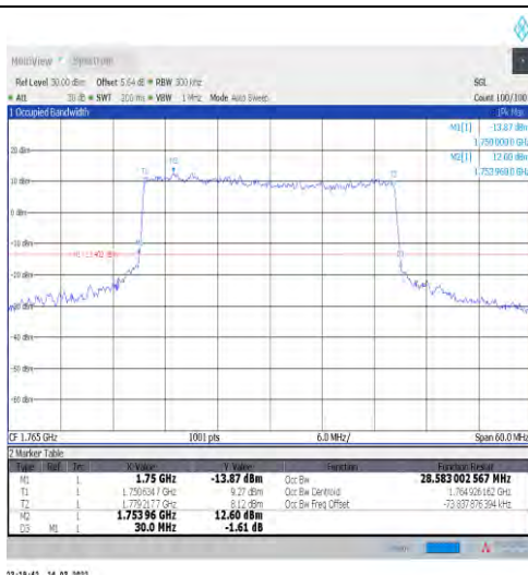
1-N66-15-30-H-7-CP-16QAM-Outer_Full-160@0-Ant 1-28.583-30.000-≤30-PASS
