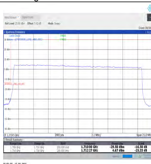
1-N66-15-20-L-3-DFT-PI2BPSK-Outer_Full-100@0-Ant1-seegraph-PASS-see graph
