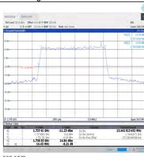
1-N66-15-15-M-3-DFT-16QAM-Outer_Full-75@0-Ant 1-13.443-14.430-≤15-PASS
