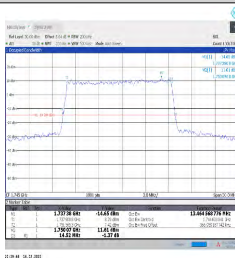
1-N66-15-15-M-5-DFT-256QAM-Outer_Full-75@0-A nt1-13.465-14.520-≤15-PASS
