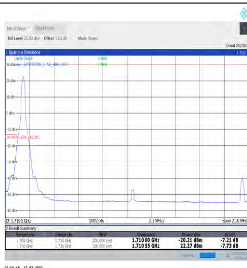
1-N66-15-20-L-1-DFT-PI2BPSK-Edge_1RB_Left-1@0-Ant1-seegraph-PASS-see graph
