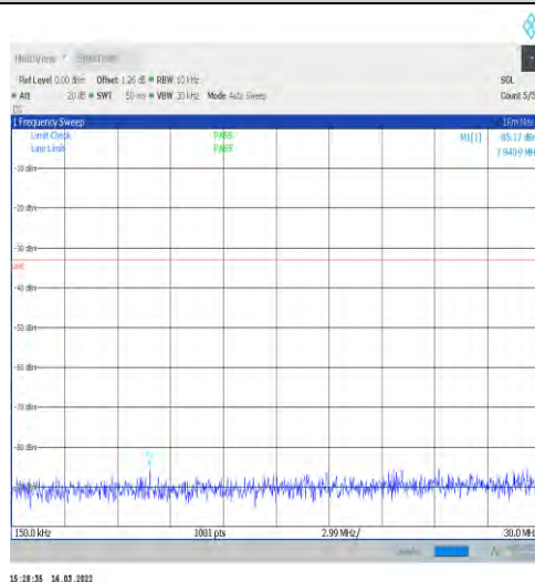
1-N66-15-40-M-1-DFT-PI2BPSK-Inner_1RB_Left-1@ 1-0.15-30-Ant1--85.17--33-PASS
