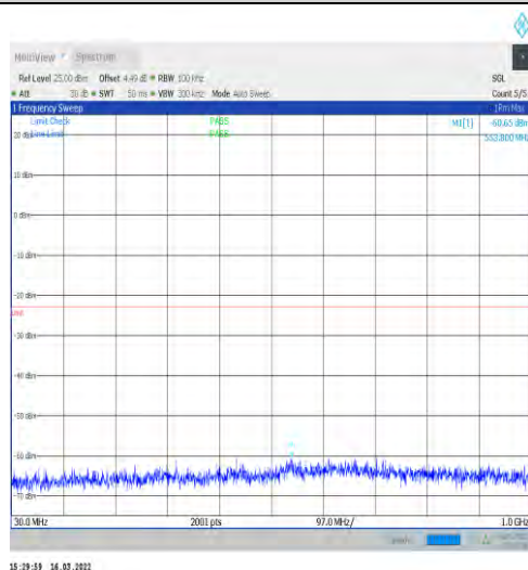
1-N66-15-40-H-1-DFT-PI2BPSK-Inner_1RB_Left-1 @1-30-1000-Ant1--60.65--23-PASS
