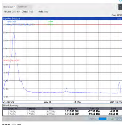
1-N66-15-15-L-4-CP-QPSK-Edge_1RB_Left-1@0-Ant1-seegraph-PASS-see graph
