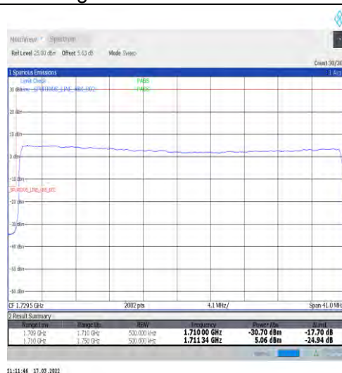
1-N66-15-40-L-3-DFT-PI2BPSK-Outer_Full-216@0-Ant1-seegraph-PASS-see graph
