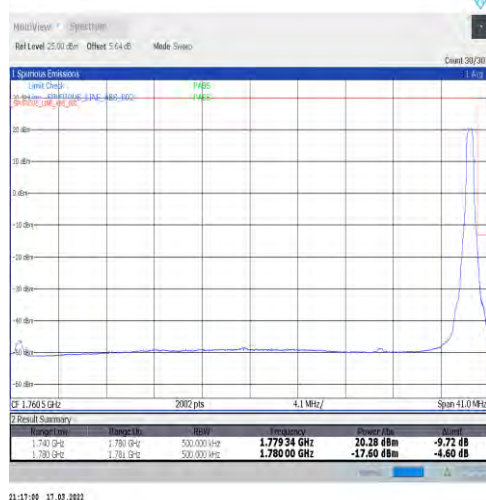
1-N66-15-40-H-5-CP-QPSK-Edge_1RB_Right-1@215-Ant1-seegraph-PASS-see graph
