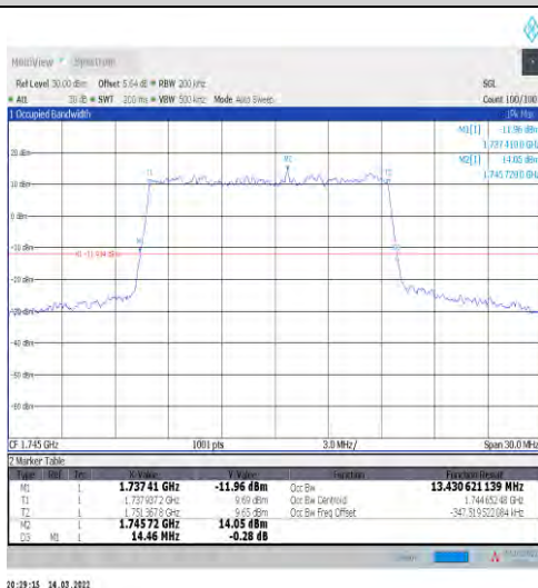
1-N66-15-15-M-4-DFT-64QAM-Outer_Full-75@0-Ant 1-13.431-14.460-≤15-PASS
