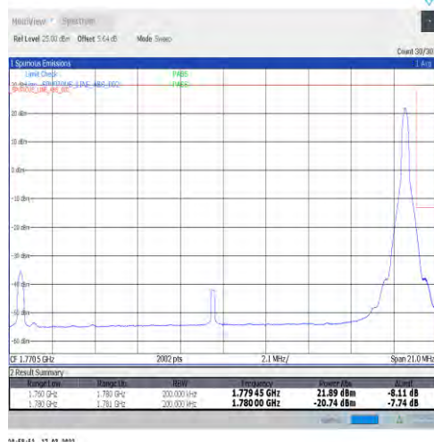
1-N66-15-20-H-2-DFT-PI2BPSK-Edge_1RB_Right-1@105-Ant1-seegraph-PASS-see graph
