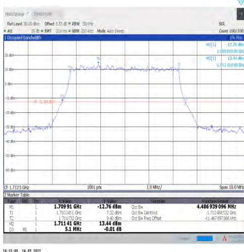
1-N66-15-5-L-1-DFT-QPSK-Outer_Full-25@0-Ant1-4 .487-5.100-≤5-PASS
