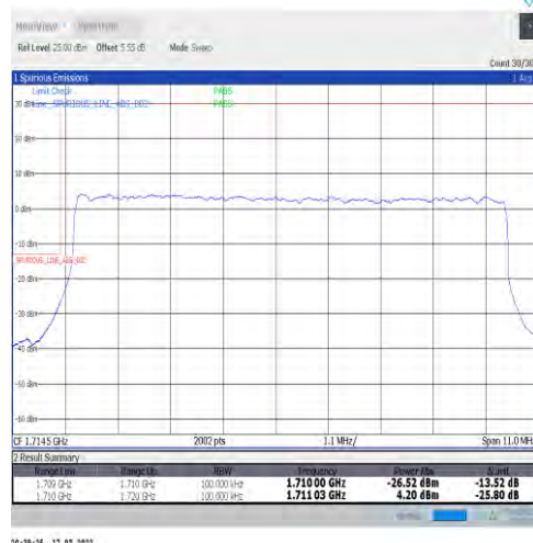
1-N66-15-10-L-3-DFT-PI2BPSK-Outer_Full-50@0-Ant1-seegraph-PASS-see graph
