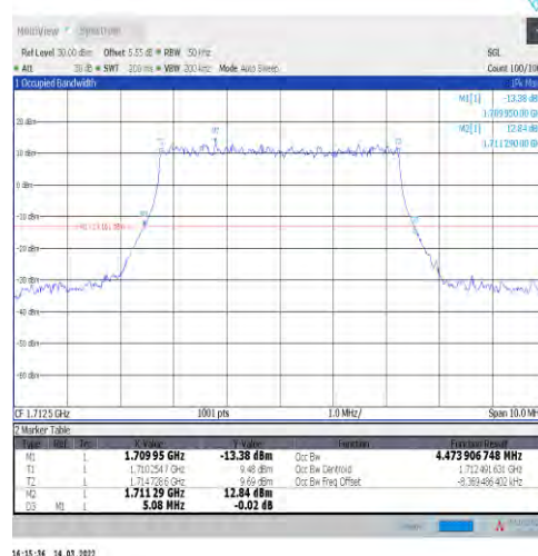
1-N66-15-5-L-2-DFT-PI2BPSK-Outer_Full-25@0-Ant1-4 1-4.474-5.080-≤5-PASS
