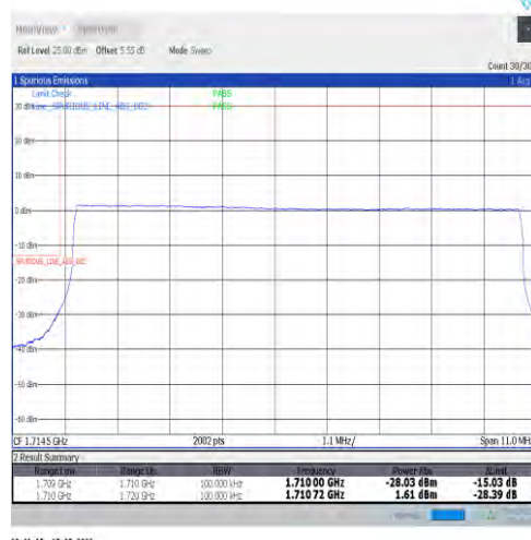
1-N66-15-10-L-6-CP-QPSK-Outer_Full-52@0-Ant1-seegraph-PASS-see graph
