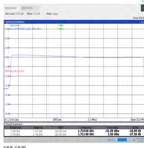
1-N66-15-30-L-6-CP-QPSK-Outer_Full-160@0-Ant1-seegraph-PASS-see graph
