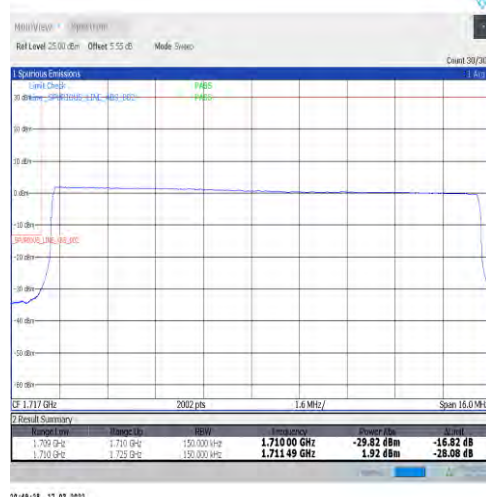
1-N66-15-15-L-6-CP-QPSK-Outer_Full-79@0-Ant1-seegraph-PASS-see graph
