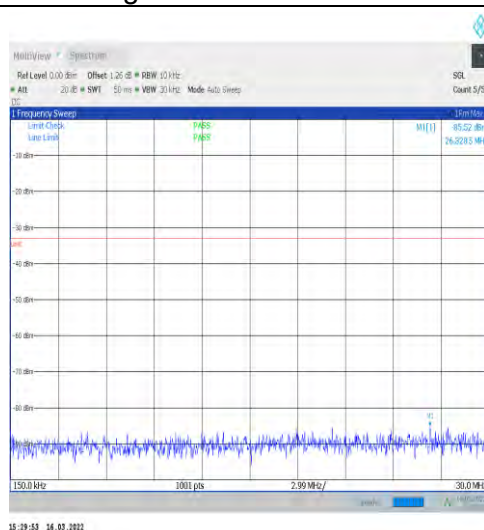
1-N66-15-40-H-1-DFT-PI2BPSK-Inner_1RB_Left-1@ 1-0.15-30-Ant1--85.52--33-PASS
