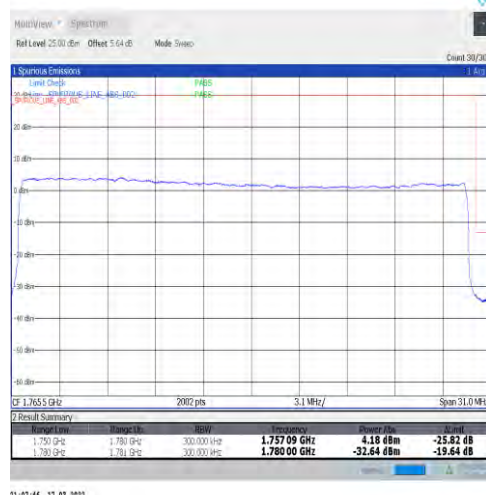
1-N66-15-30-H-3-DFT-PI2BPSK-Outer_Full-160@0-Ant1-seegraph-PASS-see graph
