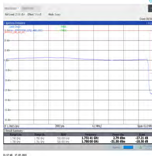
1-N66-15-40-H-6-CP-QPSK-Outer_Full-216@0-Ant1-seegraph-PASS-see graph
