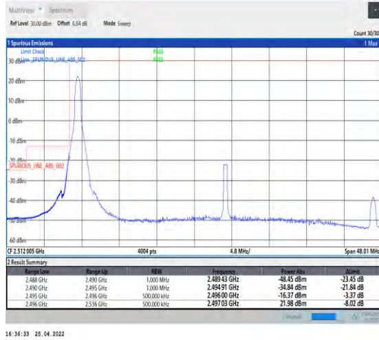
1-N41--30-40-L-4-CP-QPSK-Edge_1RB_Left-1@0-Ant 1-PASS-see graph
