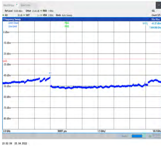
1-N41--30-100-H-1-DFT-QPSK-Edge_1RB_Left-1@ 0-3000-18000-Ant2--41.37--25-PASS
