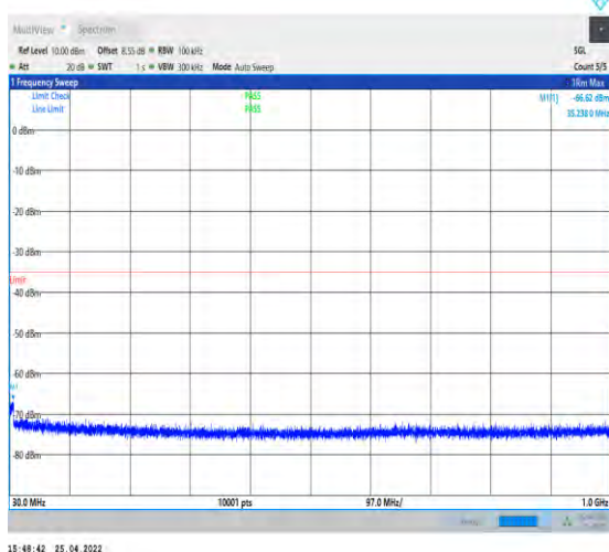
1-N41--30-100-H-1-DFT-QPSK-Edge_1RB_Left-1@ 0-30-1000-Ant1--66.62--35-PASS
