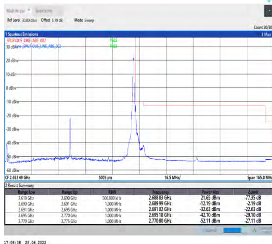
1-N41--30-80-H-5-CP-QPSK-Edge_1RB_Right-1@216-Ant 1-PASS-see graph
