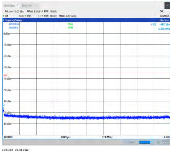
1-N41--30-100-M-1-DFT-QPSK-Edge_1RB_Left-1@ 0-30-1000-Ant2--66.97--35-PASS
