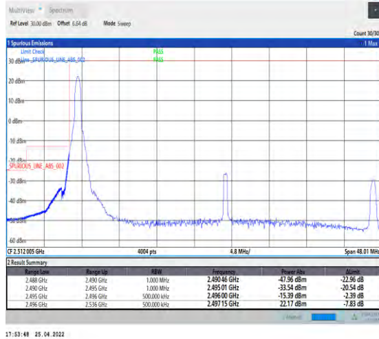
1-N41--30-40-L-4-CP-QPSK-Edge_1RB_Left-1@0-Ant 2-PASS-see graph
