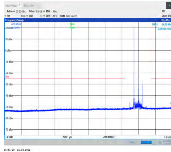
1-N41--30-100-M-1-DFT-QPSK-Edge_1RB_Left-1@ 0-1000-3000-Ant2--50.09--25-PASS
