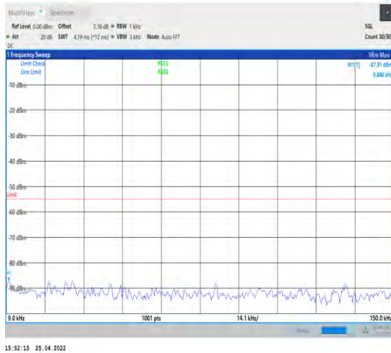
1-N41--30-100-H-1-DFT-QPSK-Edge_1RB_Left-1@ 0-0.009-0.15-Ant2--87.31--55-PASS
