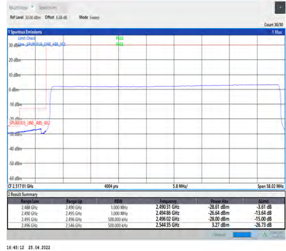
1-N41--30-50-L-6-CP-QPSK-Outer_Full-133@0-A nt1-PASS-see graph
