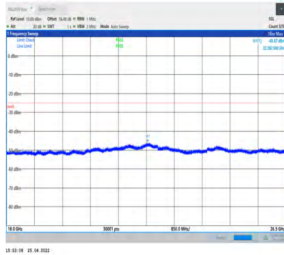
1-N41--30-100-H-1-DFT-QPSK-Edge_1RB_Left-1@ -18000-26500-Ant2--45.87--25-PASS
