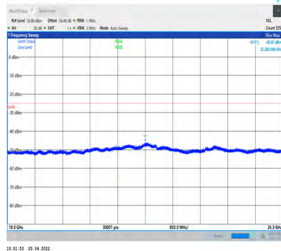
1-N41--30-100-M-1-DFT-QPSK-Edge_1RB_Left-1@ 0-18000-26500-Ant2--45.81--25-PASS
