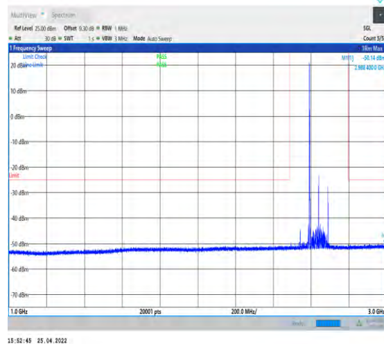
1-N41--30-100-H-1-DFT-QPSK-Edge_1RB_Left-1@ -1000-3000-Ant2--50.14--25-PASS
