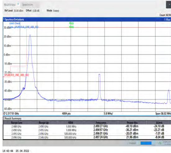
1-N41--30-50-L-4-CP-QPSK-Edge_1RB_Left-1@0-Ant 1-PASS-see graph
