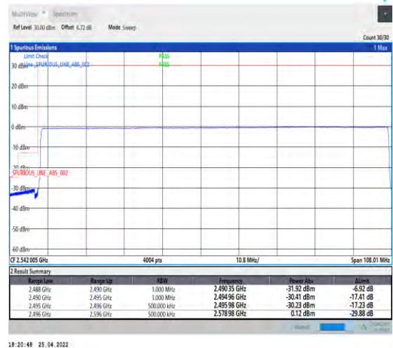
1-N41--30-100-L-6-CP-QPSK-Outer_Full-273@0-Ant 2-PASS-see graph
