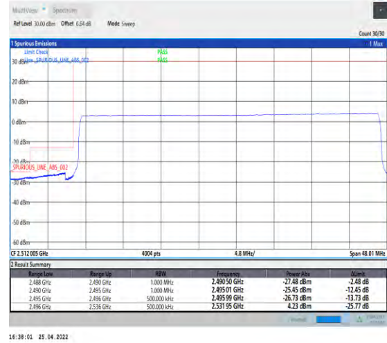
1-N41--30-40-L-6-CP-QPSK-Outer_Full-106@0-A nt1-PASS-see graph
