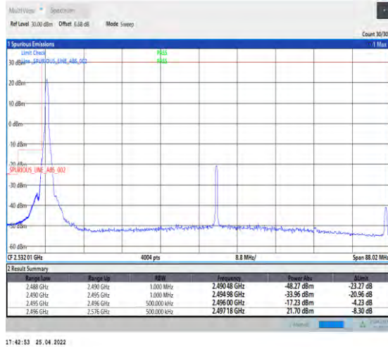
1-N41--30-80-L-4-CP-QPSK-Edge_1RB_Left-1@0-Ant 1-PASS-see graph
