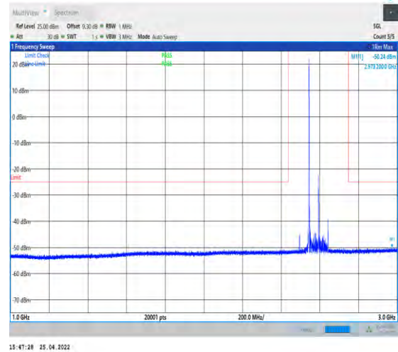
1-N41--30-100-M-1-DFT-QPSK-Edge_1RB_Left-1@ 0-1000-3000-Ant1--50.24--25-PASS
