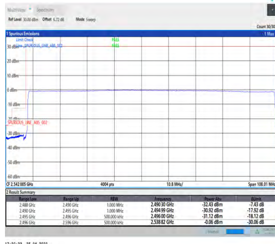
1-N41--30-100-L-6-CP-QPSK-Outer_Full-273@0-Ant1-PASS-see graph
