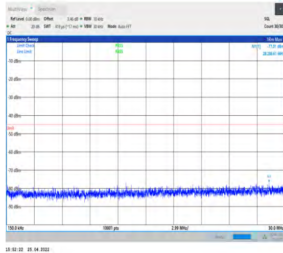
1-N41--30-100-H-1-DFT-QPSK-Edge_1RB_Left-1@ -0.15-30-Ant2--77.01--45-PASS
