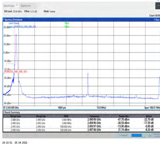
1-N41--30-100-L-4-CP-QPSK-Edge_1RB_Left-1@0-Ant 2-PASS-see graph
