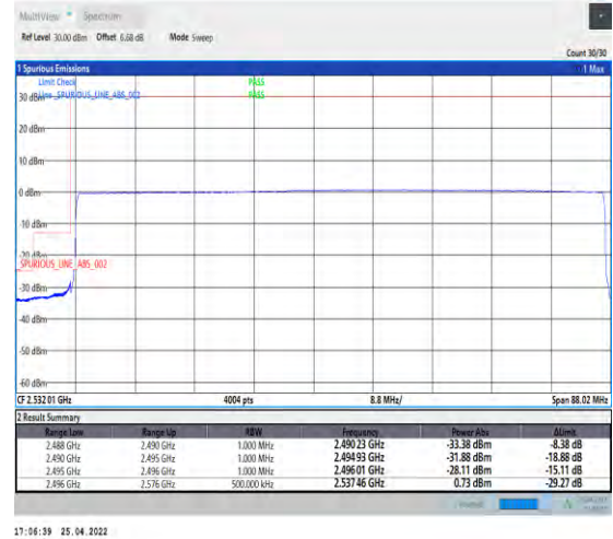
1-N41--30-80-L-6-CP-QPSK-Outer_Full-217@0-A nt1-PASS-see graph
