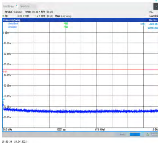
1-N41--30-100-H-1-DFT-QPSK-Edge_1RB_Left-1@ 0-30-1000-Ant2--66.66--35-PASS
