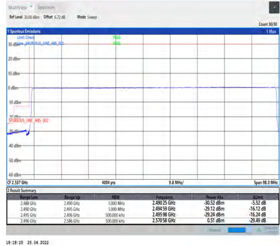
1-N41--30-90-L-6-CP-QPSK-Outer_Full-245@0-Ant 2-PASS-see graph
