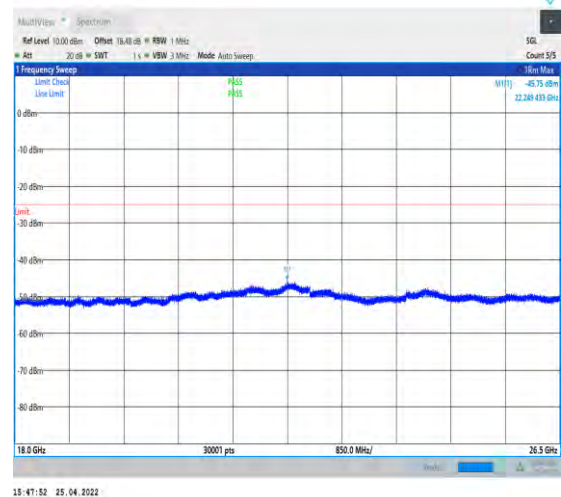
1-N41--30-100-M-1-DFT-QPSK-Edge_1RB_Left-1@ 0-18000-26500-Ant1--45.75--25-PASS
