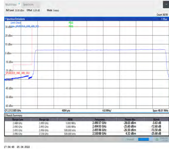
1-N41--30-40-L-6-CP-QPSK-Outer_Full-106@0-A nt2-PASS-see graph
