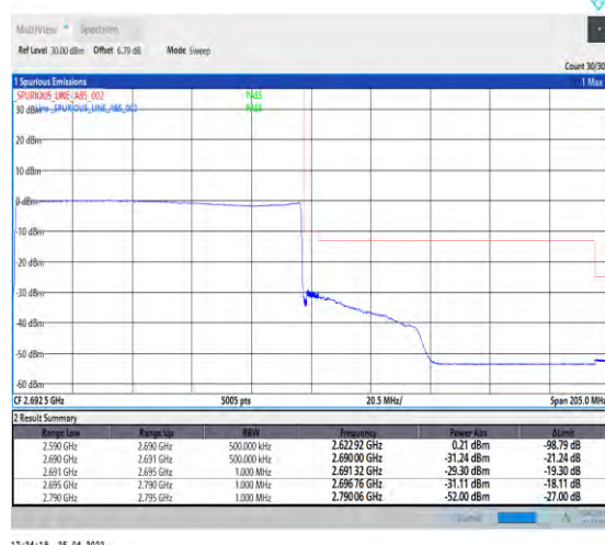
1-N41--30-100-H-6-CP-QPSK-Outer_Full-273@0-Ant1-PASS-see graph
