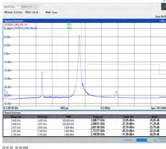
1-N41--30-50-H-5-CP-QPSK-Edge_1RB_Right-1@132-Ant 1-PASS-see graph
