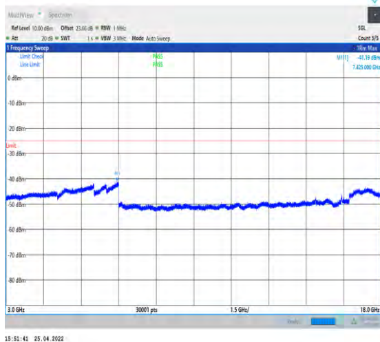
1-N41--30-100-M-1-DFT-QPSK-Edge_1RB_Left-1@ 0-3000-18000-Ant2--41.19--25-PASS
