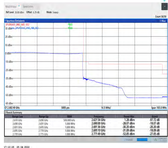
1-N41--30-80-H-6-CP-QPSK-Outer_Full-217@0-A nt1-PASS-see graph
