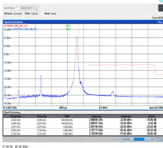
1-N41--30-40-H-5-CP-QPSK-Edge_1RB_Right-1@105-Ant 2-PASS-see graph
