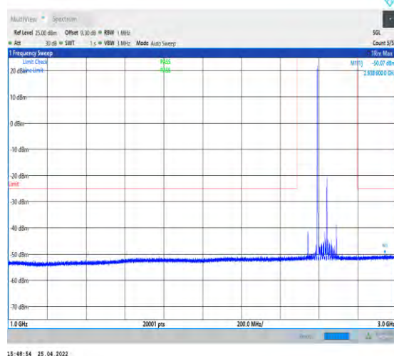
1-N41--30-100-H-1-DFT-QPSK-Edge_1RB_Left-1@ -1000-3000-Ant1--50.07--25-PASS
