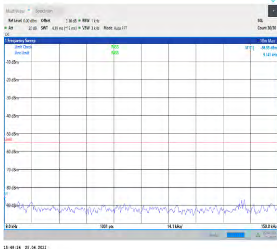
1-N41--30-100-H-1-DFT-QPSK-Edge_1RB_Left-1@ 0-0.009-0.15-Ant1--86.93--55-PASS
