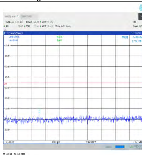
1-N41-30-100-H-1-DFT-PI2BPSK-Inner_1RB_Left-1 @1-0.15-30-Ant1--74.88--45-PASS
