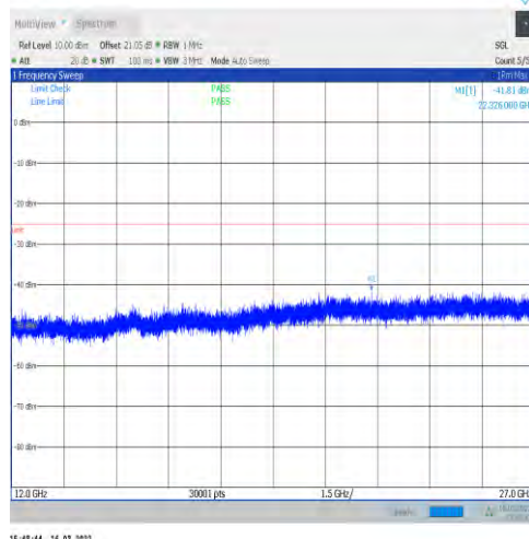
1-N41-30-100-H-1-DFT-PI2BPSK-Inner_1RB_Left-1 @1-12000-27000-Ant1--41.81--25-PASS
