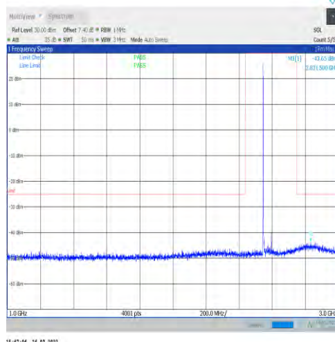
1-N41-30-100-M-1-DFT-PI2BPSK-Inner_1RB_Left-1 @1-1000-3000-Ant1--43.65--25-PASS
