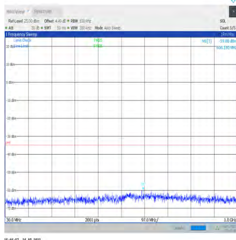
1-N41-30-100-M-1-DFT-PI2BPSK-Inner_1RB_Left-1 @1-30-1000-Ant1--59.88--35-PASS
