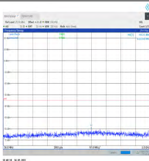
1-N41-30-100-H-1-DFT-PI2BPSK-Inner_1RB_Left-1 @1-30-1000-Ant1--60.31--35-PASS
