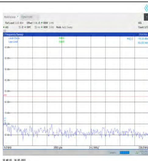
1-N41-30-100-H-1-DFT-PI2BPSK-Inner_1RB_Left-1 @1-0.009-0.15-Ant1--78.10--55-PASS
