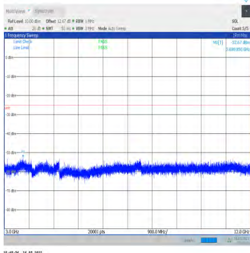
1-N41-30-100-H-1-DFT-PI2BPSK-Inner_1RB_Left-1 @1-3000-12000-Ant1--52.67--25-PASS
