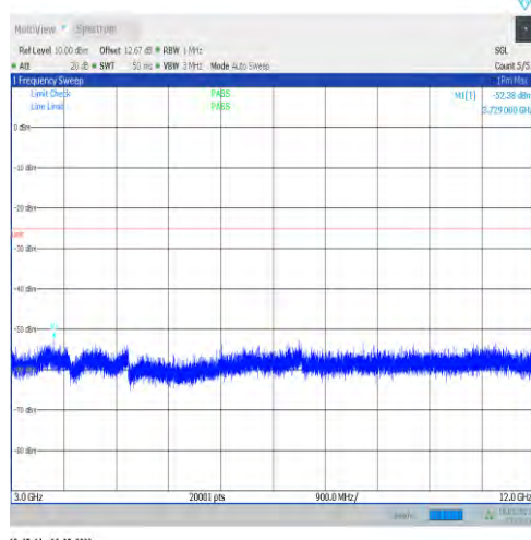
1-N41-30-100-M-1-DFT-PI2BPSK-Inner_1RB_Left-1 @1-3000-12000-Ant1--52.38--25-PASS
