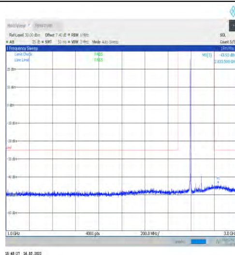
1-N41-30-100-H-1-DFT-PI2BPSK-Inner_1RB_Left-1 @1-1000-3000-Ant1--43.93--25-PASS
