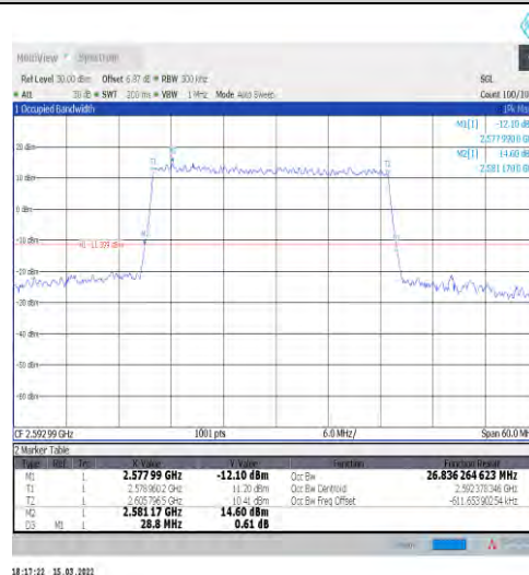
1-N41-30-30-M-4-DFT-64QAM-Outer_Full-75@0-Ant1 1-26.836-28.800-≤30-PASS
