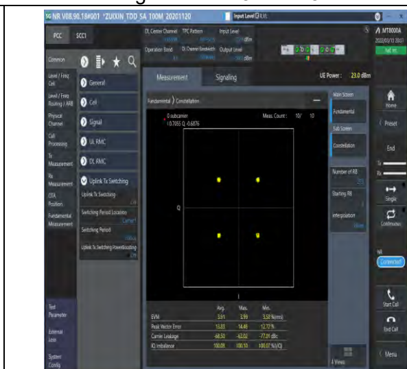
1-N41-30-100-M-6-CP-QPSK-Outer_Full-273@0-An t1-see graph-PASS
