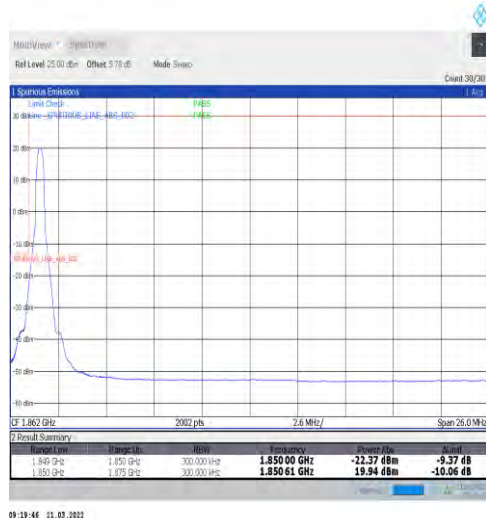
1-N25-15-25-L-4-CP-QPSK-Edge_1RB_Left-1@0-Ant1-seegraph-PASS-see graph
