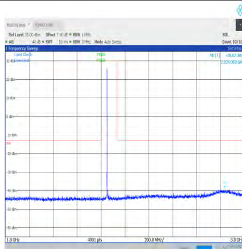
1-N25-15-40-L-1-DFT-PI2BPSK-Inner_1RB_Left-1@ 1-0.15-30-Ant1--90.91--33-PASS
