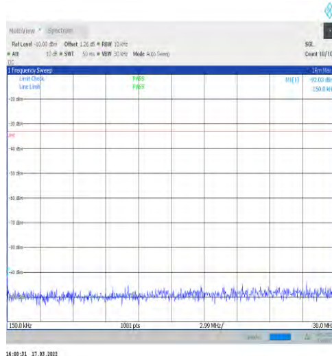
1-N25-15-40-M-1-DFT-PI2BPSK-Inner_1RB_Left-1@ 1-0.15-30-Ant1--92.03--33-PASS
