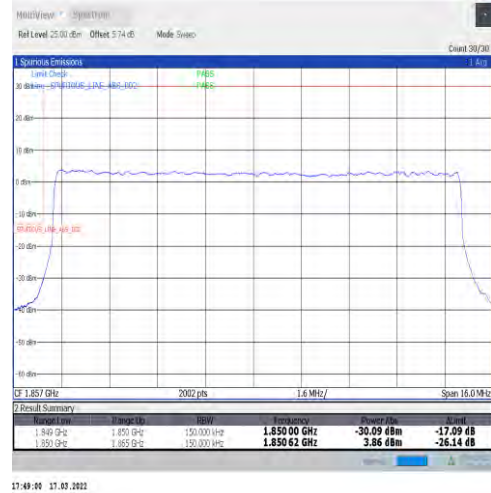
1-N25-15-15-L-3-DFT-PI2BPSK-Outer_Full-75@0-Ant1-seegraph-PASS-see graph
