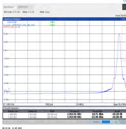
1-N25-15-25-H-5-CP-QPSK-Edge_1RB_Right-1@132-Ant1-seegraph-PASS-see graph
