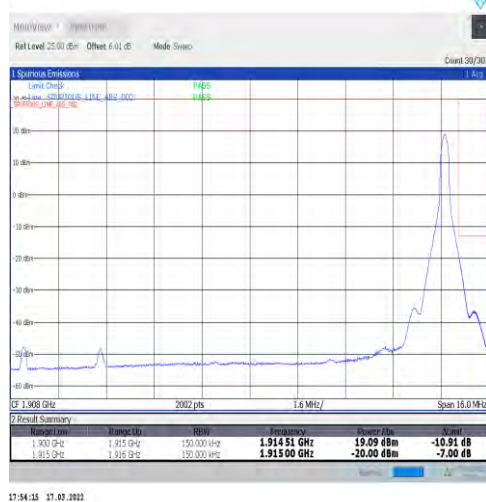
1-N25-15-15-H-5-CP-QPSK-Edge_1RB_Right-1@78-Ant1-seegraph-PASS-see graph
