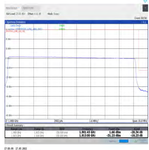
1-N25-15-15-H-6-CP-QPSK-Outer_Full-79@0-Ant1-seegraph-PASS-see graph
