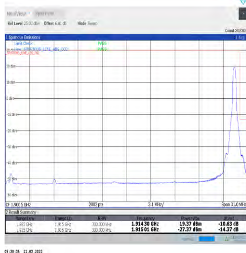
1-N25-15-30-H-5-CP-QPSK-Edge_1RB_Right-1@159-Ant1-seegraph-PASS-see graph
