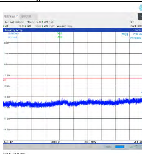
1-N25-15-40-L-1-DFT-PI2BPSK-Inner_1RB_Left-1@ 1-12000-20000-Ant1--29.15--13-PASS
