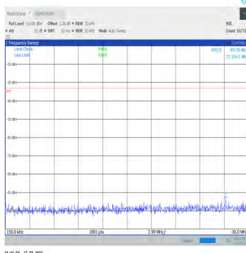
1-N25-15-40-H-1-DFT-PI2BPSK-Inner_1RB_Left-1@ 1-0.15-30-Ant1--93.70--33-PASS
