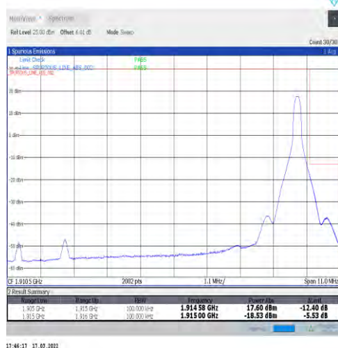
1-N25-15-10-H-5-CP-QPSK-Edge_1RB_Right-1@51-Ant1-seegraph-PASS-see graph
