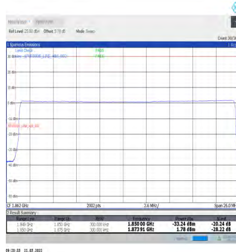
1-N25-15-25-L-6-CP-QPSK-Outer_Full-133@0-Ant1-seegraph-PASS-see graph
