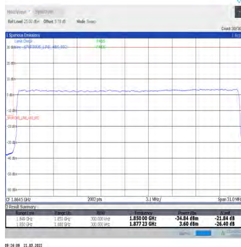
1-N25-15-30-L-3-DFT-PI2BPSK-Outer_Full-160@0-Ant1-seegraph-PASS-see graph
