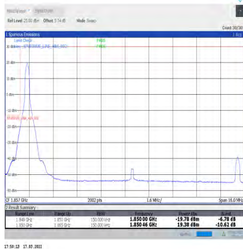
1-N25-15-15-L-4-CP-QPSK-Edge_1RB_Left-1@0-Ant1-seegraph-PASS-see graph
