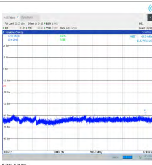
1-N25-15-40-L-1-DFT-PI2BPSK-Inner_1RB_Left-1@ 1-3000-12000-Ant1--38.74--13-PASS
