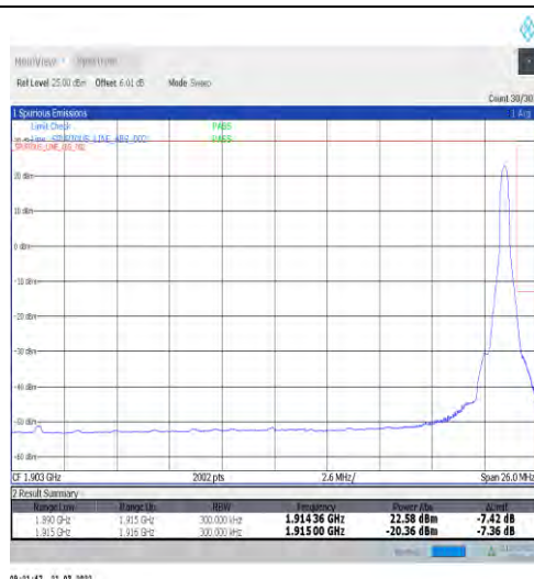
1-N25-15-25-H-2-DFT-PI2BPSK-Edge_1RB_Right-1@132-Ant1-seegraph-PASS-see graph
