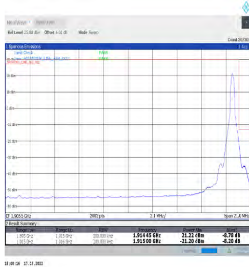
1-N25-15-20-H-2-DFT-PI2BPSK-Edge_1RB_Right-1@105-Ant1-seegraph-PASS-see graph
