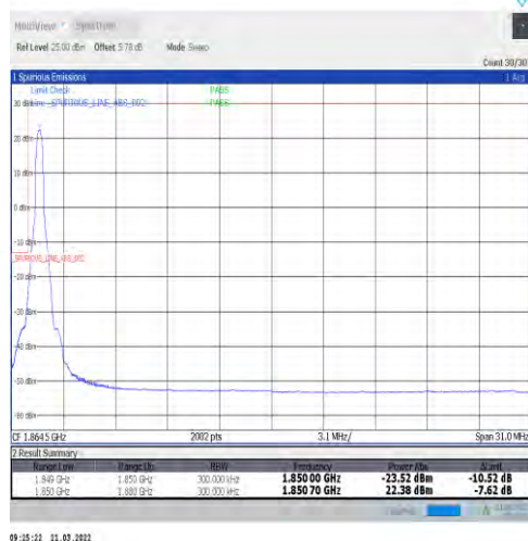
1-N25-15-30-L-1-DFT-PI2BPSK-Edge_1RB_Left-1@0-Ant1-seegraph-PASS-see graph
