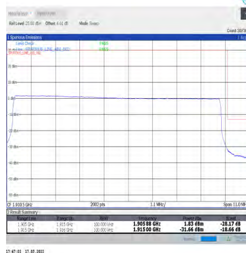
1-N25-15-10-H-6-CP-QPSK-Outer_Full-52@0-Ant1-seegraph-PASS-see graph
