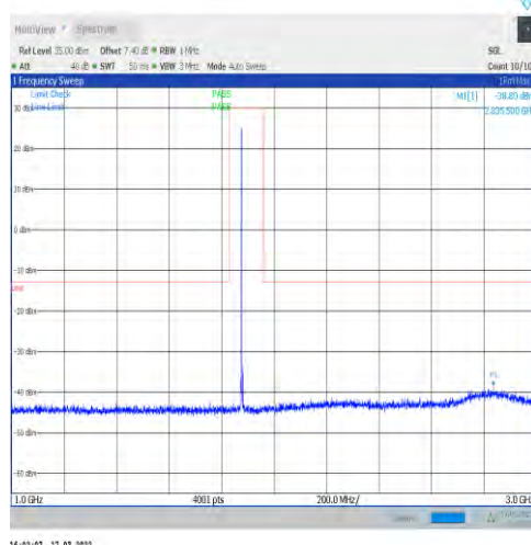
1-N25-15-40-H-1-DFT-PI2BPSK-Inner_1RB_Left-1@ 1-1000-3000-Ant1--38.80--13-PASS
