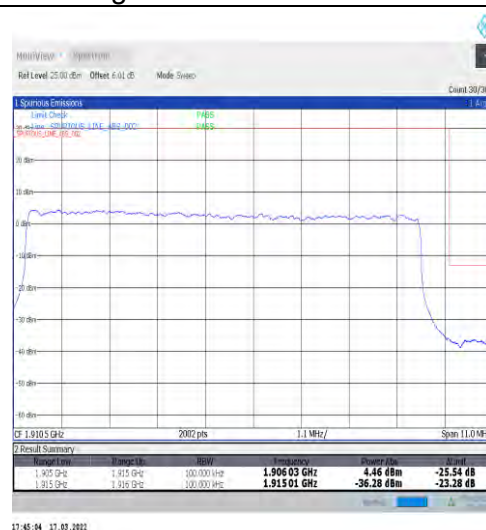
1-N25-15-10-H-3-DFT-PI2BPSK-Outer_Full-50@0-Ant1-seegraph-PASS-see graph
