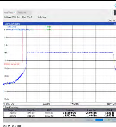
1-N25-15-5-L-6-CP-QPSK-Outer_Full-25@0-Ant1-seegraph-PASS-see graph
