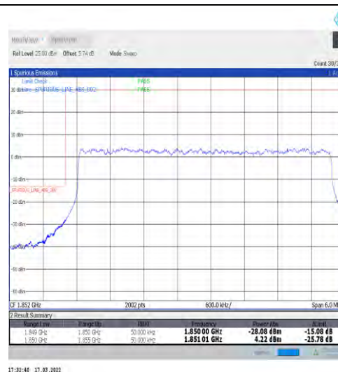
1-N25-15-5-L-3-DFT-PI2BPSK-Outer_Full-25@0-Ant1-seegraph-PASS-see graph
