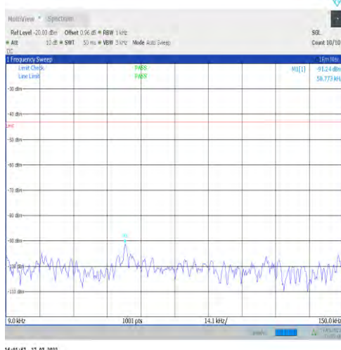
1-N25-15-40-H-1-DFT-PI2BPSK-Inner_1RB_Left-1 @1-0.009-0.15-Ant1--91.24--43-PASS
