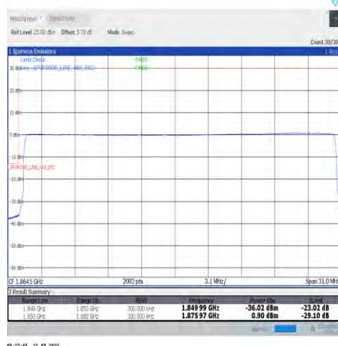
1-N25-15-30-L-6-CP-QPSK-Outer_Full-160@0-Ant1-seegraph-PASS-see graph
