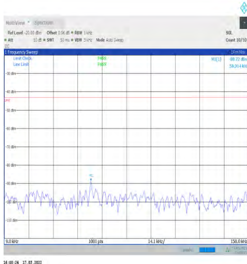
1-N25-15-40-M-1-DFT-PI2BPSK-Inner_1RB_Left-1@ 1-0.009-0.15-Ant1--88.72--43-PASS
