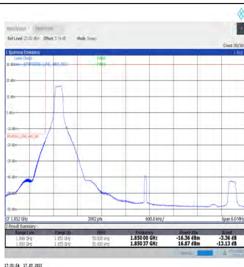
1-N25-15-5-L-1-DFT-PI2BPSK-Edge_1RB_Left-1@0-Ant1-seegraph-PASS-see graph
