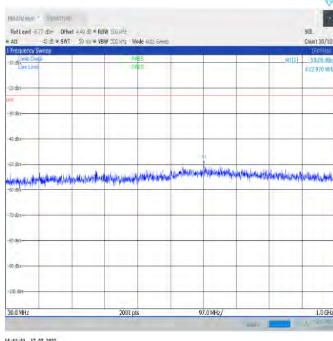
1-N25-15-40-H-1-DFT-PI2BPSK-Inner_1RB_Left-1 @1-30-1000-Ant1--50.08--23-PASS
