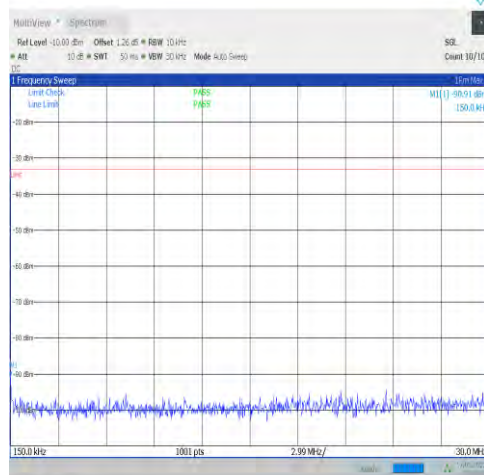
1-N25-15-40-L-1-DFT-PI2BPSK-Inner_1RB_Left-1@ 1-0.15-30-Ant1--90.91--33-PASS
