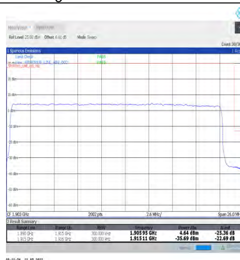
1-N25-15-25-H-3-DFT-PI2BPSK-Outer_Full-128@0-Ant1-seegraph-PASS-see graph
