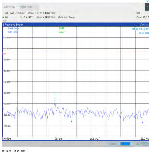
1-N25-15-40-L-1-DFT-PI2BPSK-Inner_1RB_Left-1@ 1-0.009-0.15-Ant1--88.68--43-PASS
