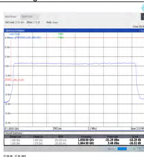
1-N25-15-20-L-3-DFT-PI2BPSK-Outer_Full-100@0-Ant1-seegraph-PASS-see graph
