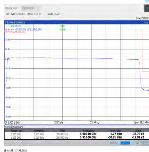
1-N25-15-20-H-6-CP-QPSK-Outer_Full-106@0-Ant1-seegraph-PASS-see graph
