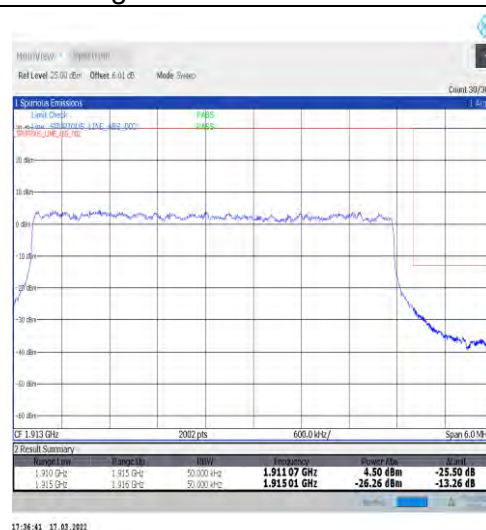
1-N25-15-5-H-3-DFT-PI2BPSK-Outer_Full-25@0-Ant1-seegraph-PASS-see graph
