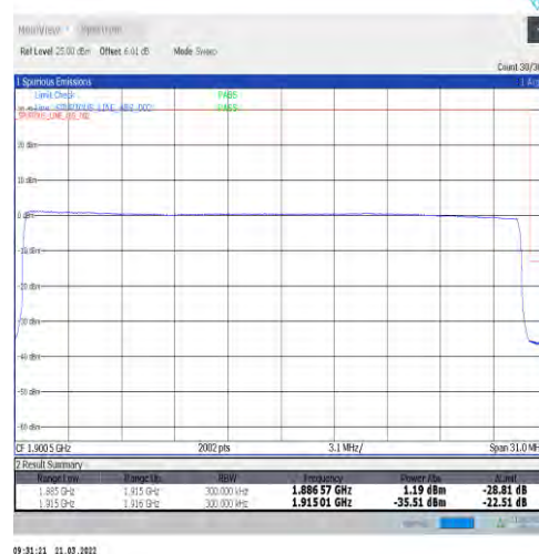
1-N25-15-30-H-6-CP-QPSK-Outer_Full-160@0-Ant1-seegraph-PASS-see graph
