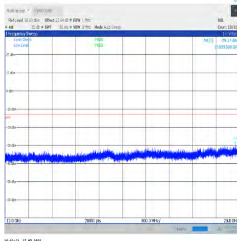
1-N25-15-40-H-1-DFT-PI2BPSK-Inner_1RB_Left-1@ 1-12000-20000-Ant1--29.17--13-PASS
