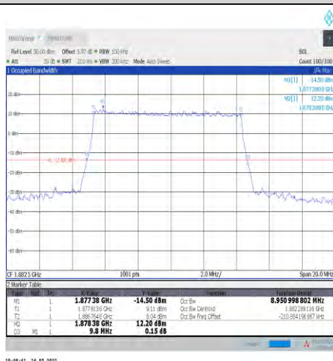
1-N25-15-10-M-3-DFT-16QAM-Outer_Full-50@0-Ant1 1-8.951-9.800≤10-PASS
