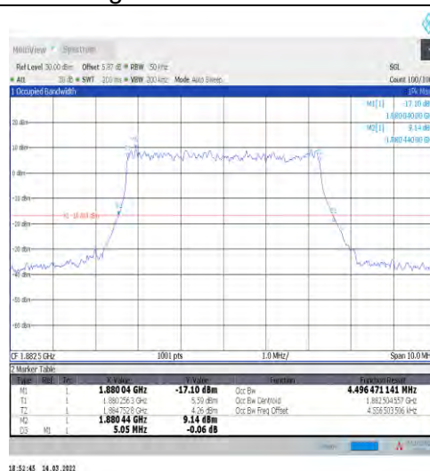
1-N25-15-5-M-5-DFT-256QAM-Outer_Full-25@0-Ant 1-4.496-5.050-≤5-PASS
