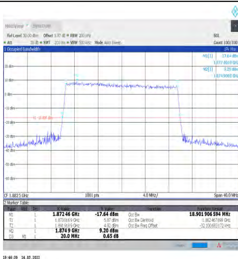
1-N25-15-20-M-9-CP-256QAM-Outer_Full-106@0-Ant 1-18.902-20.000-≤20-PASS
