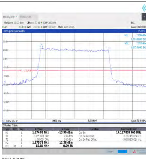
1-N25-15-15-M-6-CP-QPSK-Outer_Full-79@0-Ant1- 14.128-15.180≤15-PASS
