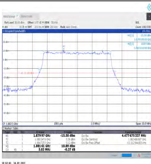
1-N25-15-5-M-6-CP-QPSK-Outer_Full-25@0-Ant1-4. 478-5.030-≤5-PASS
