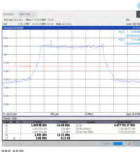
1-N25-15-5-L-3-DFT-16QAM-Outer_Full-25@0-Ant1-4 4.478-5.060-≤5-PASS
