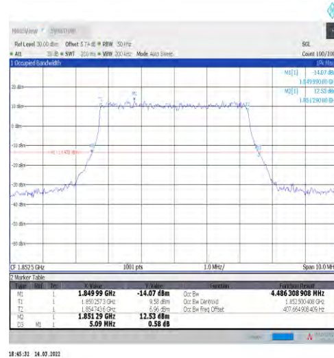
1-N25-15-5-L-2-DFT-PI2BPSK-Outer_Full-25@0-Ant1-4 1-4.486-5.090-≤5-PASS
