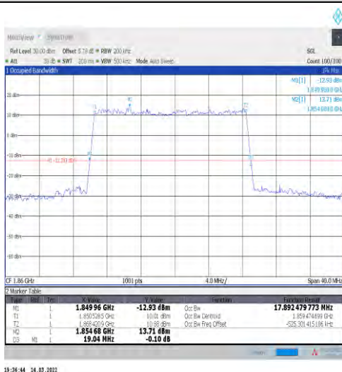
1-N25-15-20-L-2-DFT-PI2BPSK-Outer_Full-100@0-Ant1-17.892-19.040-≤20-PASS
