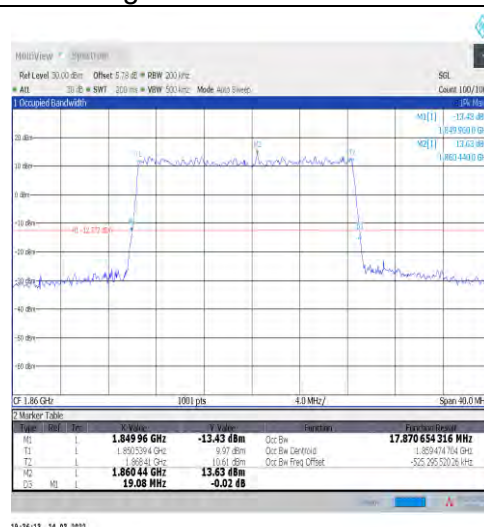
1-N25-15-20-L-1-DFT-QPSK-Outer_Full-100@0-Ant 1-17.871-19.080-≤20-PASS
