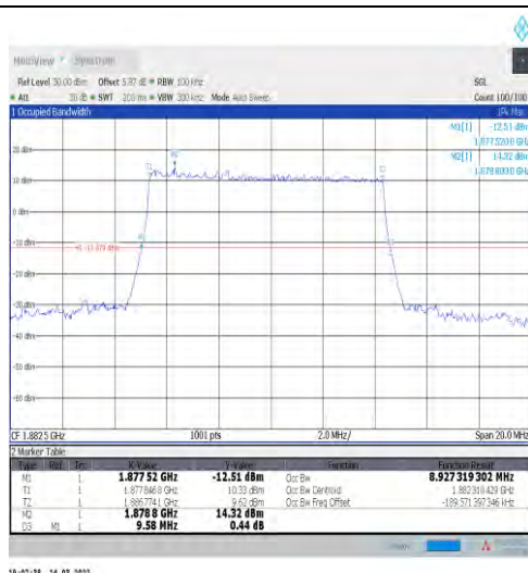
1-N25-15-10-M-1-DFT-QPSK-Outer_Full-50@0-Ant1 -8.927-9.580≤10-PASS
