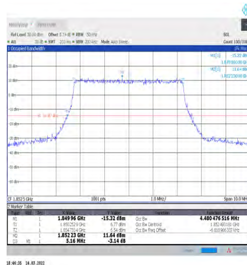
1-N25-15-5-L-4-DFT-64QAM-Outer_Full-25@0-Ant1-4 4.48-5.160-≤5-PASS
