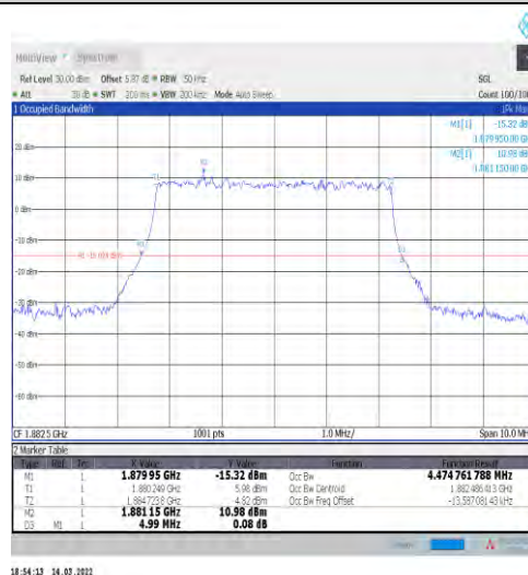
1-N25-15-5-M-7-CP-16QAM-Outer_Full-25@0-Ant1- 4.475-4.990-≤5-PASS
