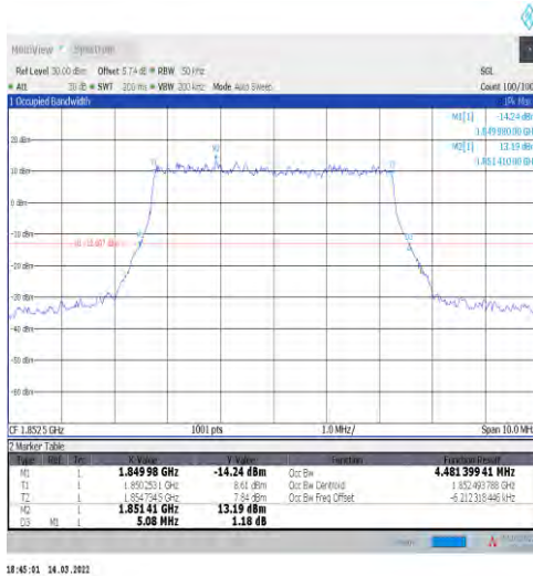
1-N25-15-5-L-1-DFT-QPSK-Outer_Full-25@0-Ant1-4 1.481-5.080-≤5-PASS
