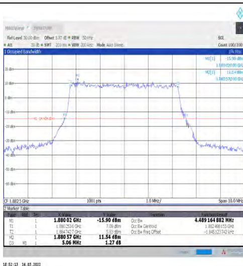
1-N25-15-5-M-4-DFT-64QAM-Outer_Full-25@0-Ant1 -4.489-5.060-≤5-PASS
