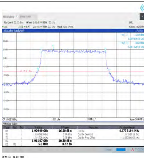
1-N25-15-5-H-7-CP-16QAM-Outer_Full-25@0-Ant1-4.477-5.000-≤5-PASS
