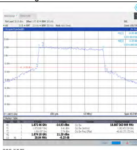
1-N25-15-20-M-8-CP-64QAM-Outer_Full-106@0-Ant 1-18.887-20.040-≤20-PASS
