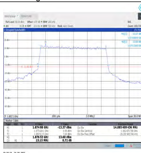
1-N25-15-15-M-7-CP-16QAM-Outer_Full-79@0-Ant1 -14.085-15.150≤15-PASS
