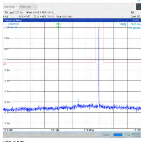
1-N12-15-15-M-1-DFT-PI2BPSK-Inner_1RB_Left-1 @1-30-1000-Ant1--50.80--13-PASS
