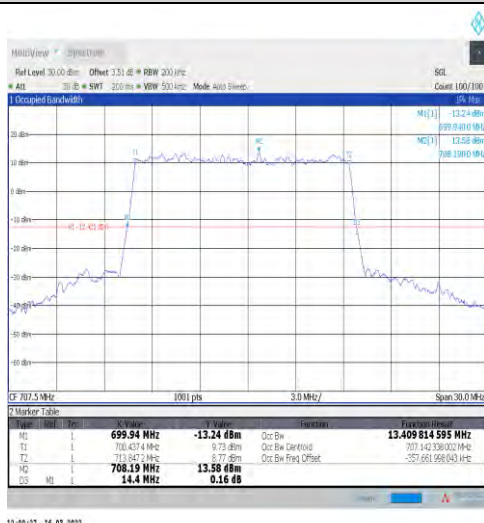
1-N12-15-15-M-4-DFT-64QAM-Outer_Full-75@0-Ant 1-13.41-14.400-≤15-PASS
