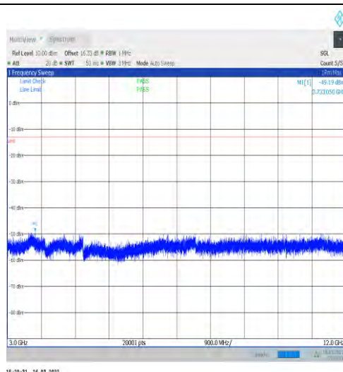
1-N12-15-15-L-1-DFT-PI2BPSK-Inner_1RB_Left-1@ 1-3000-12000-Ant1--49.19--13-PASS
