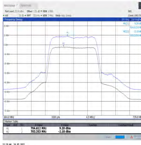
1-N12-15-15-L-2-CP-256QAM-Outer_Full-79@0-Ant t1-11.38-100%-0.00-11.38-PASS-≤13
