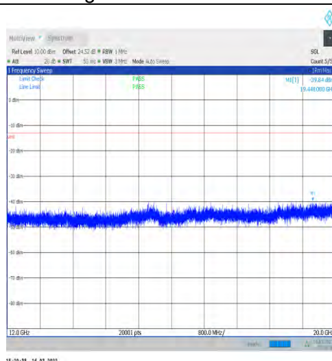
1-N12-15-15-L-1-DFT-PI2BPSK-Inner_1RB_Left-1@ 1-12000-20000-Ant1--39.84--13-PASS
