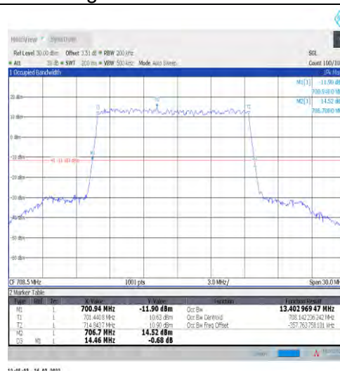
1-N12-15-15-H-2-DFT-PI2BPSK-Outer_Full-75@0-Ant1 -13.403-14.460≤15-PASS
