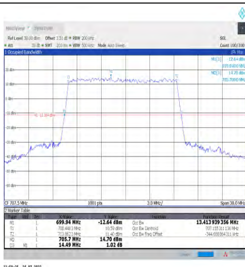
1-N12-15-15-M-2-DFT-PI2BPSK-Outer_Full-75@0-A nt1-13.414-14.490-≤15-PASS
