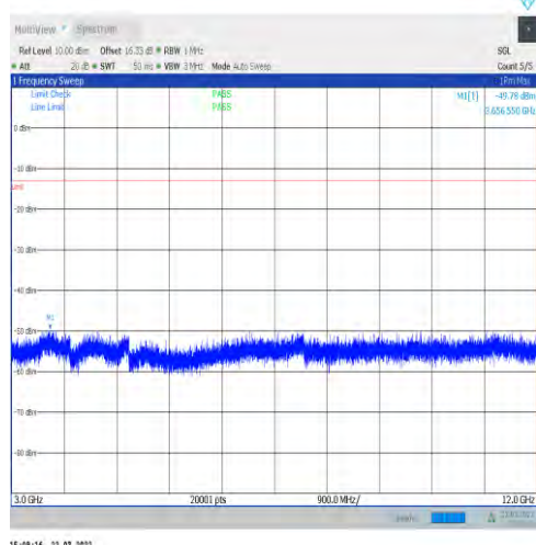
1-N12-15-15-M-1-DFT-PI2BPSK-Inner_1RB_Left-1 @1-3000-12000-Ant1--49.78--13-PASS
