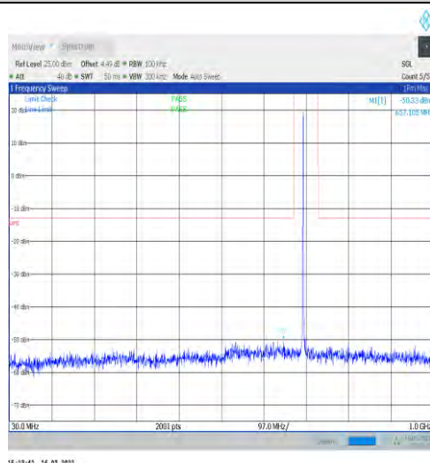
1-N12-15-15-H-1-DFT-PI2BPSK-Inner_1RB_Left-1 @1-30-1000-Ant1--50.33--13-PASS
