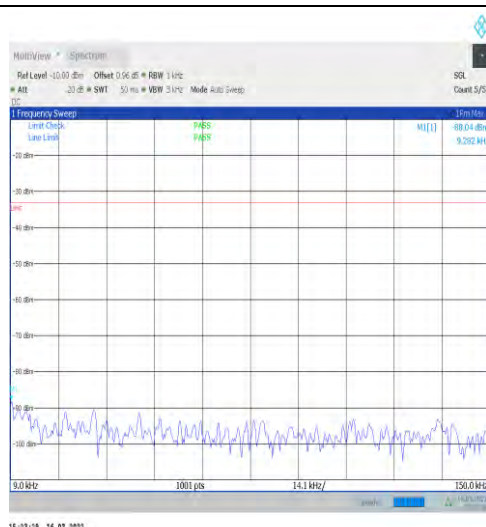
1-N12-15-15-H-1-DFT-PI2BPSK-Inner_1RB_Left-1 @1-0.009-0.15-Ant1--88.04--33-PASS
