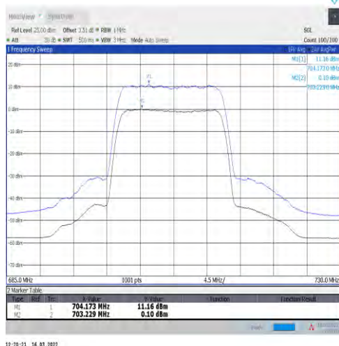
1-N12-15-15-M-1-DFT-256QAM-Outer_Full-75@0-A nt1-11.06-100%-0.00-11.06-PASS-≤13
