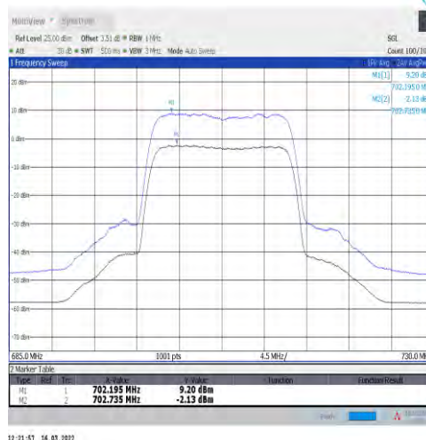
1-N12-15-15-M-2-CP-256QAM-Outer_Full-79@0-Ant t1-11.33-100%-0.00-11.33-PASS-≤13
