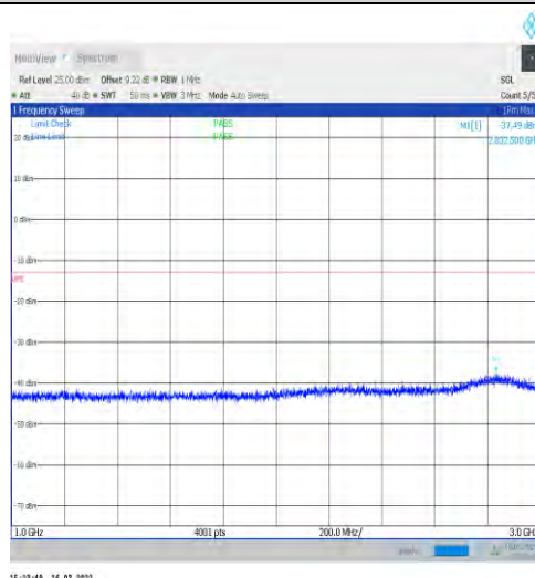
1-N12-15-15-H-1-DFT-PI2BPSK-Inner_1RB_Left-1@ 1-1000-3000-Ant1--37.49--13-PASS
