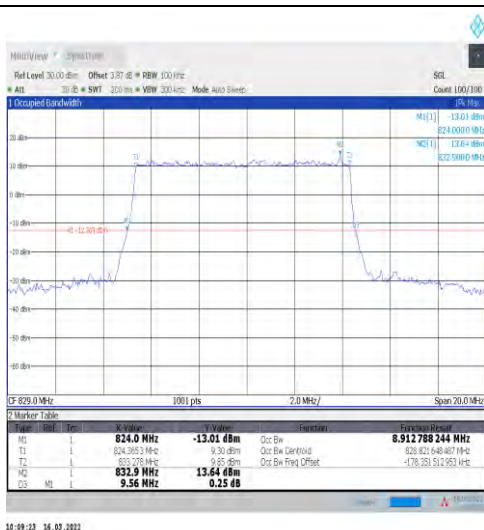
1-N5-15-10-L-2-DFT-PI2BPSK-Outer_Full-50@0-Ant 1-8.913-9.560-≤10-PASS
