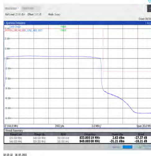
1-N5-15-20-H-6-CP-QPSK-Outer_Full-106@0-Ant1-seegraph-PASS-see graph
