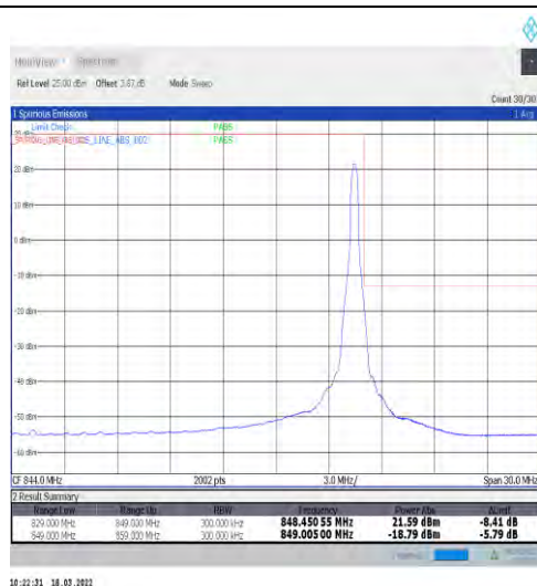
1-N5-15-20-H-2-DFT-PI2BPSK-Edge_1RB_Right-1@105-Ant1-seegraph-PASS-see graph
