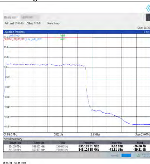
1-N5-15-15-H-3-DFT-PI2BPSK-Outer_Full-75@0- Ant1-seegraph-PASS-see graph
