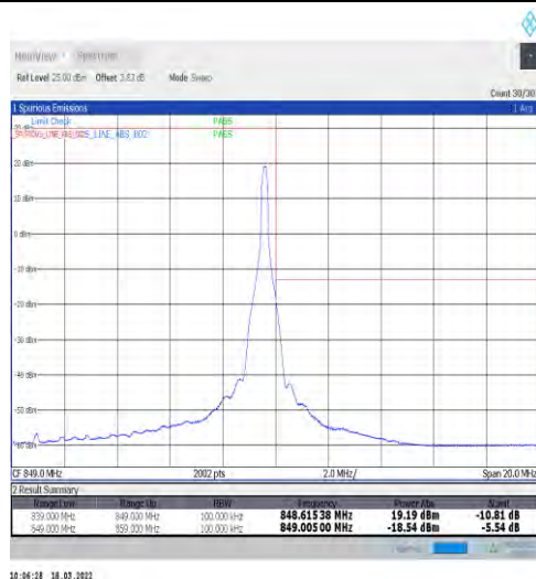
1-N5-15-10-H-2-DFT-PI2BPSK-Edge_1RB_Right-1@5 1-Ant1-seegraph-PASS-see graph
