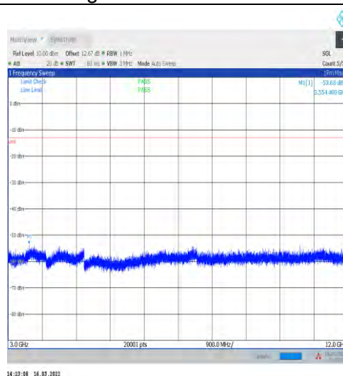
1-N5-15-20-M-1-DFT-PI2BPSK-Inner_1RB_Left-1@ 1-3000-12000-Ant1--53.68--13-PASS
