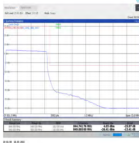
1-N5-15-5-H-6-CP-QPSK-Outer_Full-25@0-Ant1-seegraph-PASS-see graph
