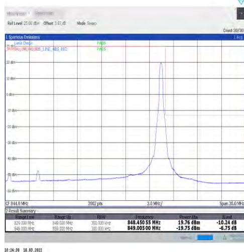
1-N5-15-20-H-5-CP-QPSK-Edge_1RB_Right-1@105-Ant1-seegraph-PASS-see graph
