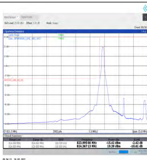
1-N5-15-5-L-1-DFT-PI2BPSK-Edge_1RB_Left-1@0-Ant1-seegraph-PASS-see graph
