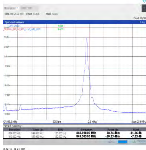
1-N5-15-15-H-5-CP-QPSK-Edge_1RB_Right-1@78-An t1-seegraph-PASS-see graph
