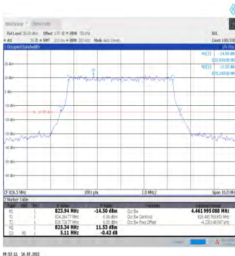
1-N5-15-5-L-3-DFT-16QAM-Outer_Full-25@0-Ant1- 4.462-5.110-≤5-PASS
