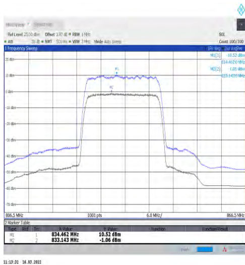
1-N5-15-20-M-1-DFT-256QAM-Outer_Full-100@0-A nt1-11.58-100%-0.00-11.58-PASS-≤13
