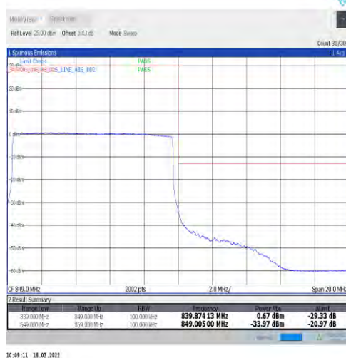
1-N5-15-10-H-6-CP-QPSK-Outer_Full-52@0-Ant1 -seegraph-PASS-see graph
