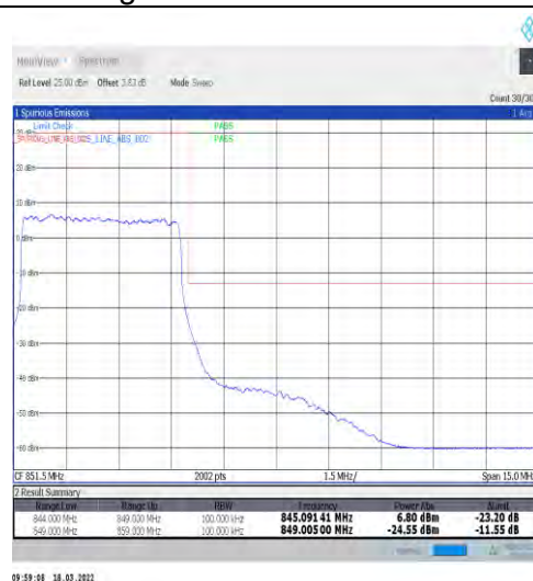
1-N5-15-5-H-3-DFT-PI2BPSK-Outer_Full-25@0-Ant1-seegraph-PASS-see graph
