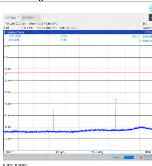
1-N5-15-20-H-1-DFT-PI2BPSK-Inner_1RB_Left-1@1 -1000-3000-Ant1--39.66--13-PASS
