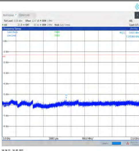
1-N5-15-20-H-1-DFT-PI2BPSK-Inner_1RB_Left-1@ 1-3000-12000-Ant1--54.01--13-PASS
