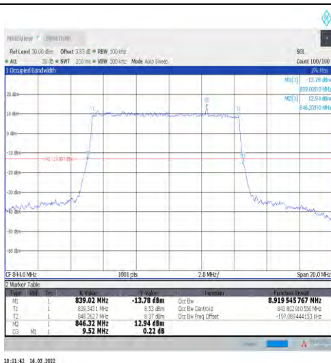
1-N5-15-10-H-4-DFT-64QAM-Outer_Full-50@0-Ant1 -8.92-9.520-≤10-PASS
