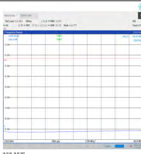
1-N5-15-20-H-1-DFT-PI2BPSK-Inner_1RB_Left-1@ 1-0.15-30-Ant1--90.45--23-PASS
