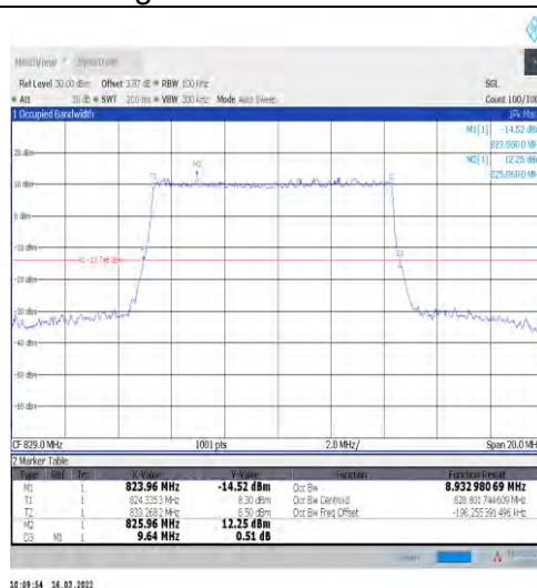
1-N5-15-10-L-3-DFT-16QAM-Outer_Full-50@0-Ant1 8.933-9.640-≤10-PASS
