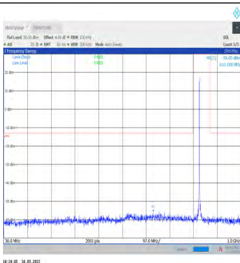
1-N5-15-20-H-1-DFT-PI2BPSK-Inner_1RB_Left-1@ 1-30-1000-Ant1--56.05--13-PASS
