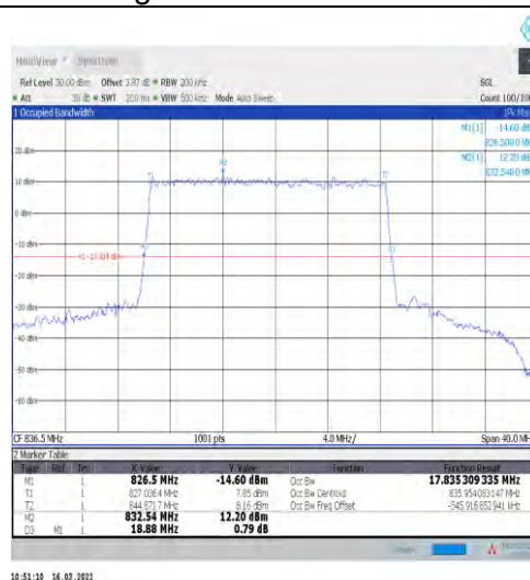
1-N5-15-20-M-4-DFT-64QAM-Outer_Full-100@0-Ant 1-17.835-18.880-≤20-PASS
