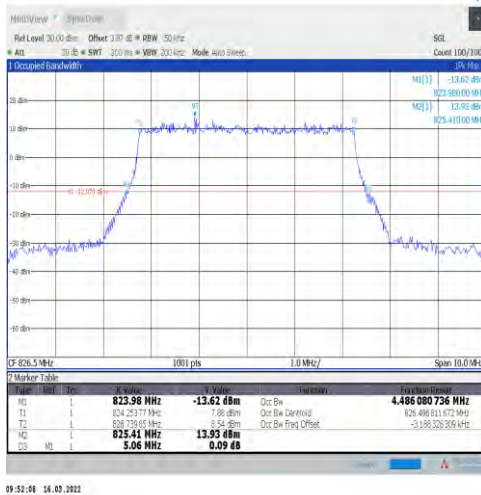
1-N5-15-5-L-1-DFT-QPSK-Outer_Full-25@0-Ant1-4. 486-5.060-≤5-PASS
