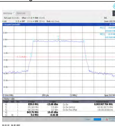
1-N5-15-10-H-5-DFT-256QAM-Outer_Full-50@0-Ant 1-8.906-9.600-≤10-PASS
