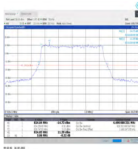
1-N5-15-5-L-4-DFT-64QAM-Outer_Full-25@0-Ant1-4 .49-5.060-≤5-PASS
