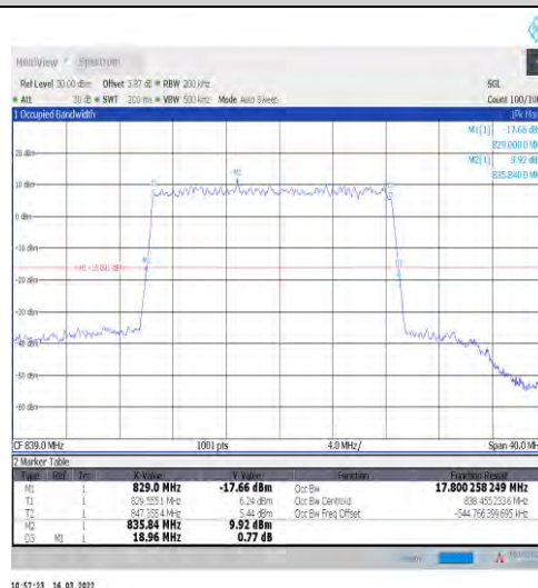
1-N5-15-20-H-5-DFT-256QAM-Outer_Full-100@0-A nt1-17.8-18.960-≤20-PASS
