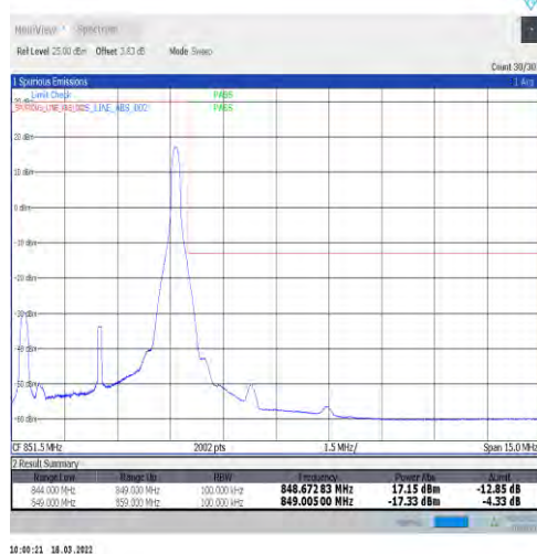
1-N5-15-5-H-5-CP-QPSK-Edge_1RB_Right-1@24-Ant1-seegraph-PASS-see graph
