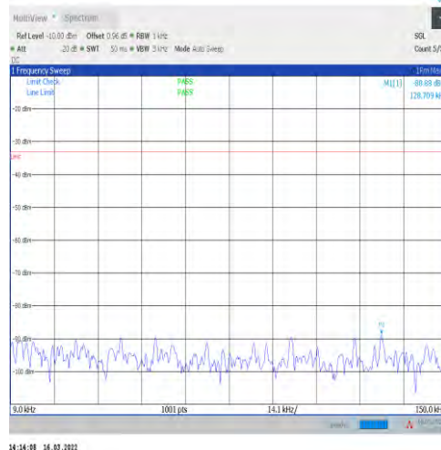
1-N5-15-20-M-1-DFT-PI2BPSK-Inner_1RB_Left-1@ 1-0.009-0.15-Ant1--88.88--33-PASS
