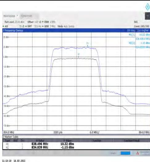
1-N5-15-20-L-1-DFT-256QAM-Outer_Full-100@0-An t1-11.47-100%-0.00-11.47-PASS-≤13
