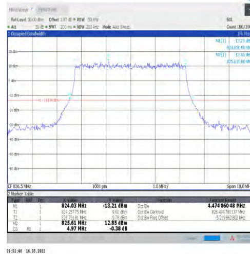
1-N5-15-5-L-2-DFT-PI2BPSK-Outer_Full-25@0-Ant1 -4.474-4.970-≤5-PASS
