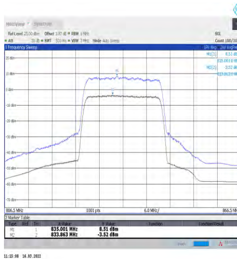
1-N5-15-20-M-2-CP-256QAM-Outer_Full-106@0-Ant t1-12.03-100%-0.00-12.03-PASS-≤13
