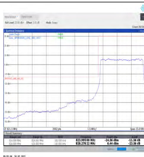
1-N5-15-5-L-3-DFT-PI2BPSK-Outer_Full-25@0-Ant1-seegraph-PASS-see graph
