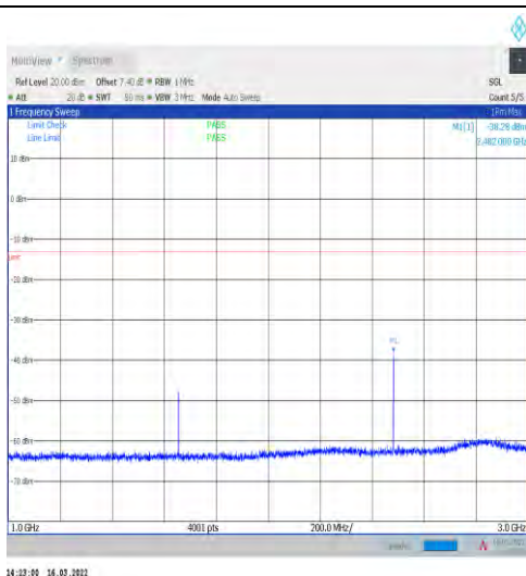
1-N5-15-20-M-1-DFT-PI2BPSK-Inner_1RB_Left-1@ 1-1000-3000-Ant1--38.28--13-PASS
