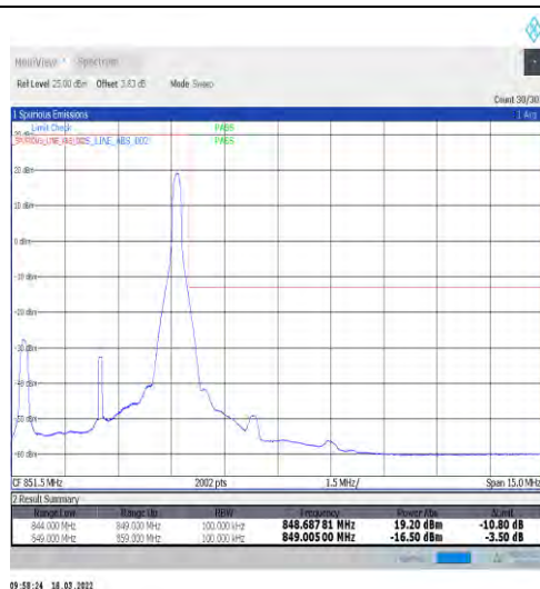
1-N5-15-5-H-2-DFT-PI2BPSK-Edge_1RB_Right-1@24-Ant1-seegraph-PASS-see graph
