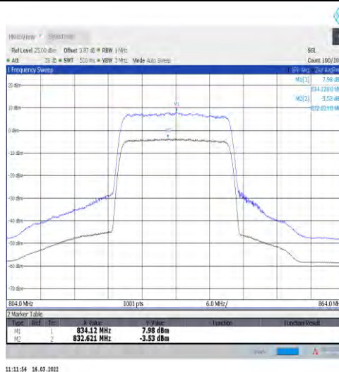
1-N5-15-20-L-2-CP-256QAM-Outer_Full-106@0-Ant 1-11.51-100%-0.00-11.51-PASS-≤13
