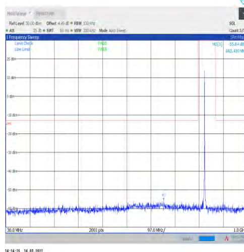
1-N5-15-20-M-1-DFT-PI2BPSK-Inner_1RB_Left-1@ 1-30-1000-Ant1--55.84--13-PASS
