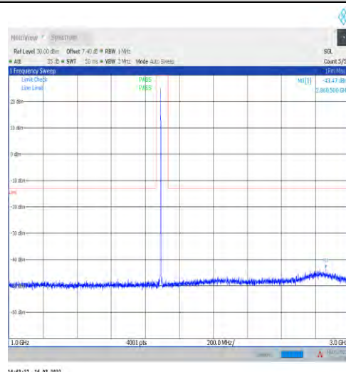
1-N2-15-20-H-1-DFT-PI2BPSK-Inner_1RB_Left-1@ -1000-3000-Ant1--43.47--13-PASS
