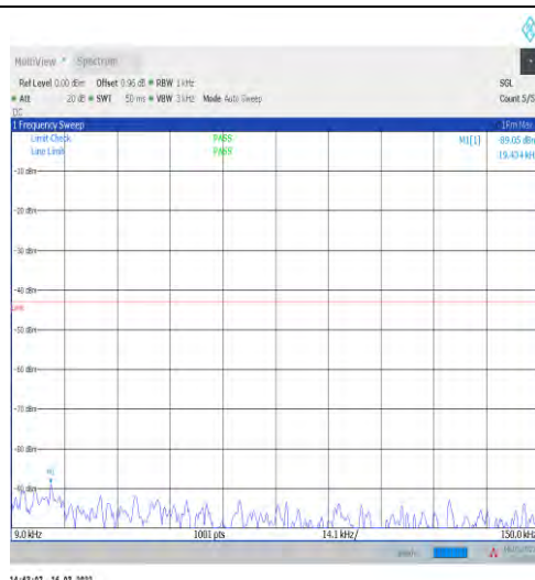
1-N2-15-20-H-1-DFT-PI2BPSK-Inner_1RB_Left-1@ 1-0.009-0.15-Ant1--89.05--43-PASS
