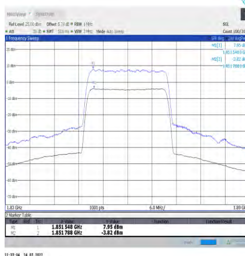
1-N2-15-20-L-2-CP-256QAM-Outer_Full-106@0-Ant t1-11.77-100%-0.00-11.77-PASS-≤13
