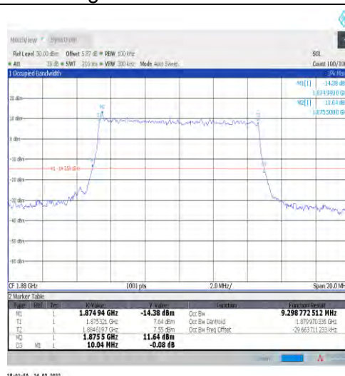
1-N2-15-10-M-6-CP-QPSK-Outer_Full-52@0-Ant1-9. 299-10.040-≤10-PASS
