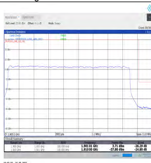
1-N2-15-10-H-3-DFT-PI2BPSK-Outer_Full-50@0-Ant1-seegraph-PASS-see graph
