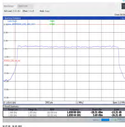
1-N2-15-10-L-3-DFT-PI2BPSK-Outer_Full-50@0-Ant1-seegraph-PASS-see graph
