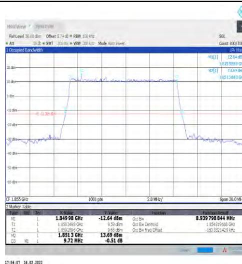
1-N2-15-10-L-1-DFT-QPSK-Outer_Full-50@0-Ant1-8 .94-9.720-≤10-PASS
