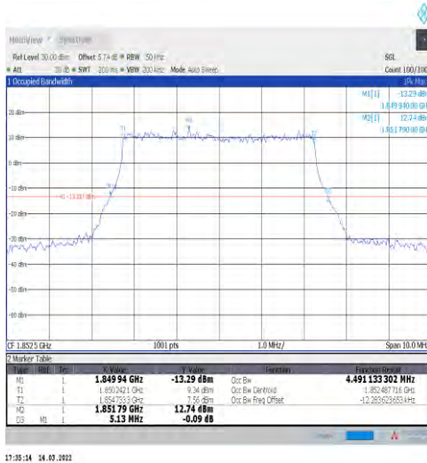
1-N2-15-5-L-1-DFT-QPSK-Outer_Full-25@0-Ant1-4. 491-5.130-≤5-PASS
