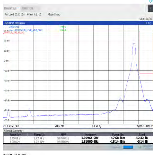
1-N2-15-10-H-5-CP-QPSK-Edge_1RB_Right-1@51-Ant1-seegraph-PASS-see graph
