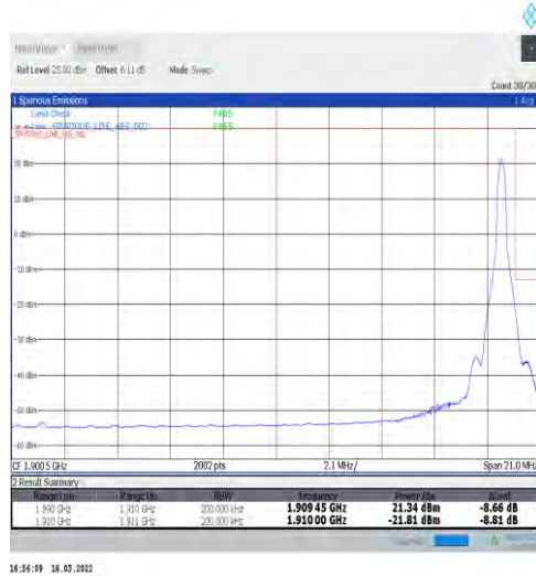
1-N2-15-20-H-2-DFT-PI2BPSK-Edge_1RB_Right-1@105-Ant1-seegraph-PASS-see graph
