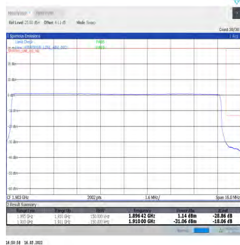
1-N2-15-15-H-6-CP-QPSK-Outer_Full-79@0-Ant1-seegraph-PASS-see graph
