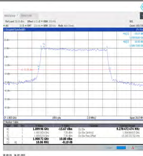
1-N2-15-10-H-7-CP-16QAM-Outer_Full-52@0-Ant1- 9.278-10.060≤10-PASS
