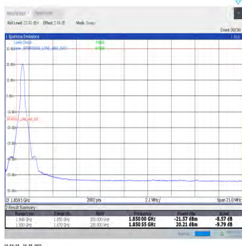
1-N2-15-20-L-4-CP-QPSK-Edge_1RB_Left-1@0-Ant1- seegraph-PASS-see graph
