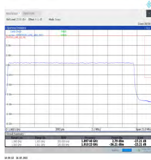
1-N2-15-20-H-3-DFT-PI2BPSK-Outer_Full-100@0-Ant1-seegraph-PASS-see graph
