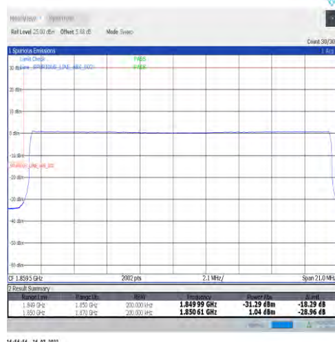
1-N2-15-20-L-6-CP-QPSK-Outer_Full-106@0-Ant 1-seegraph-PASS-see graph
