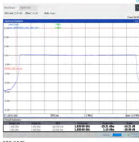
1-N2-15-10-L-6-CP-QPSK-Outer_Full-52@0-Ant1-seegraph-PASS-see graph
