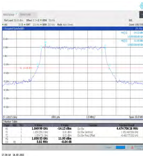
1-N2-15-5-L-3-DFT-16QAM-Outer_Full-25@0-Ant1- 4.475-5.020-≤5-PASS
