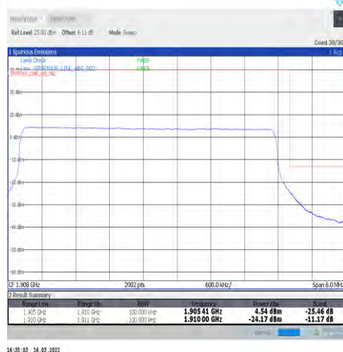
1-N2-15-5-H-6-CP-QPSK-Outer_Full-25@0-Ant1-s eegraph-PASS-see graph
