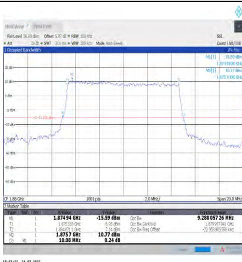
1-N2-15-10-M-7-CP-16QAM-Outer_Full-52@0-Ant1- 9.288-10.080-≤10-PASS
