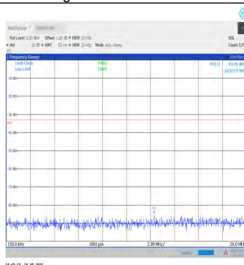
1-N2-15-20-H-1-DFT-PI2BPSK-Inner_1RB_Left-1@ -0.15-30-Ant1--84.96--33-PASS
