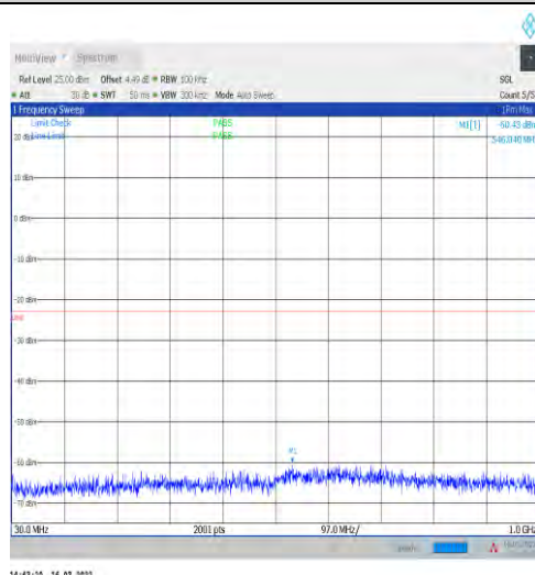
1-N2-15-20-H-1-DFT-PI2BPSK-Inner_1RB_Left-1@ 1-30-1000-Ant1--60.43--23-PASS
