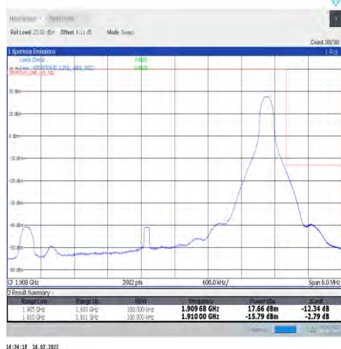
1-N2-15-5-H-5-CP-QPSK-Edge_1RB_Right-1@24-Ant 1-seegraph-PASS-see graph
