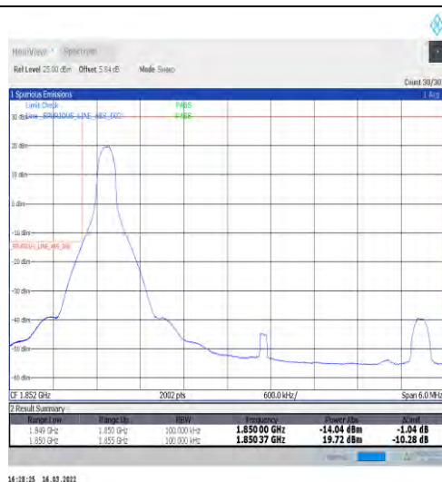
1-N2-15-5-L-1-DFT-PI2BPSK-Edge_1RB_Left-1@0-Ant1-seegraph-PASS-see graph
