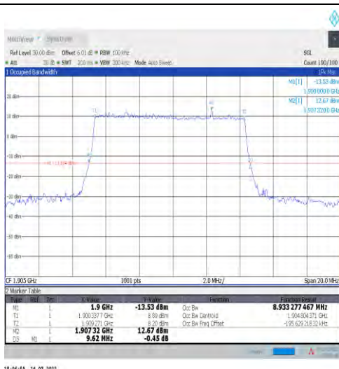
1-N2-15-10-H-4-DFT-64QAM-Outer_Full-50@0-Ant1 -8.933-9.620≤10-PASS
