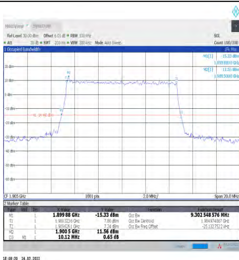
1-N2-15-10-H-6-CP-QPSK-Outer_Full-52@0-Ant1-9. 303-10.120≤10-PASS
