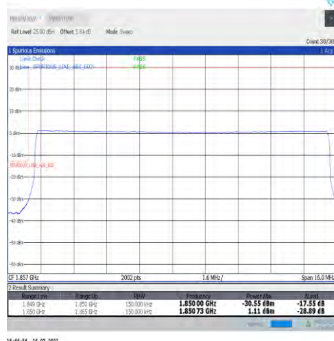
1-N2-15-15-L-6-CP-QPSK-Outer_Full-79@0-Ant1-seegraph-PASS-see graph
