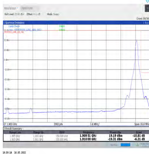
1-N2-15-15-H-5-CP-QPSK-Edge_1RB_Right-1@78-Ant1-seegraph-PASS-see graph
