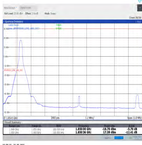
1-N2-15-10-L-4-CP-QPSK-Edge_1RB_Left-1@0-Ant1-seegraph-PASS-see graph
