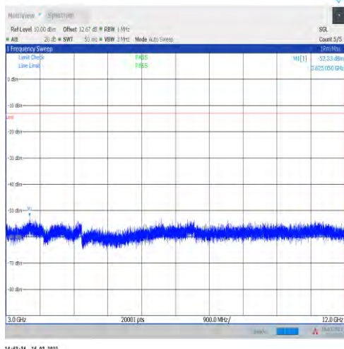
1-N2-15-20-H-1-DFT-PI2BPSK-Inner_1RB_Left-1@ 1-3000-12000-Ant1--52.33--13-PASS
