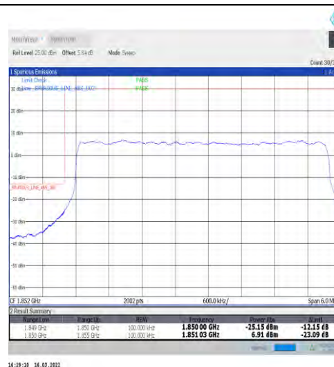
1-N2-15-5-L-3-DFT-PI2BPSK-Outer_Full-25@0-Ant1-seegraph-PASS-see graph
