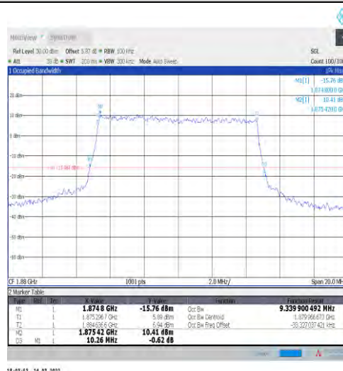
1-N2-15-10-M-8-CP-64QAM-Outer_Full-52@0-Ant1- 9.34-10.260-≤10-PASS
