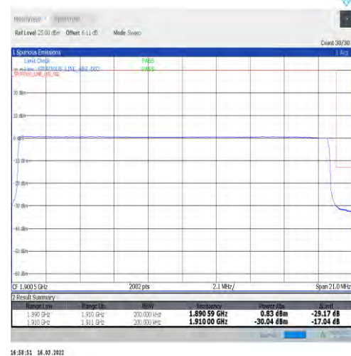
1-N2-15-20-H-6-CP-QPSK-Outer_Full-106@0-Ant1-seegraph-PASS-see graph
