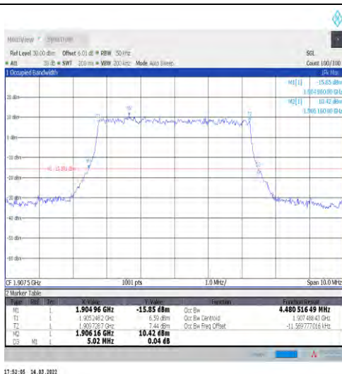
1-N2-15-5-H-7-CP-16QAM-Outer_Full-25@0-Ant1-4. 481-5.020-≤5-PASS
