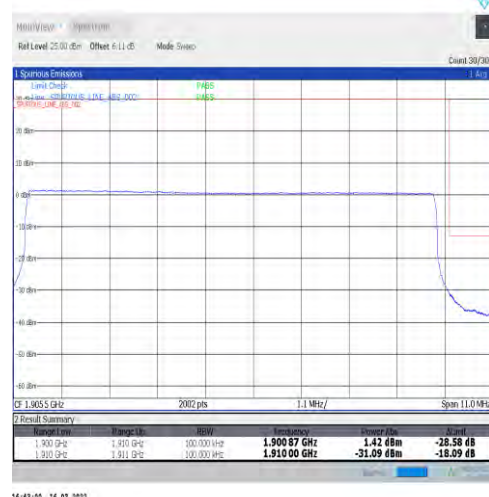
1-N2-15-10-H-6-CP-QPSK-Outer_Full-52@0-Ant1-seegraph-PASS-see graph
