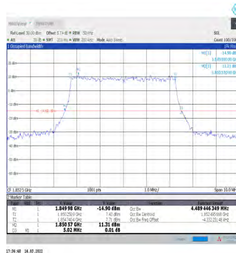
1-N2-15-5-L-4-DFT-64QAM-Outer_Full-25@0-Ant1-4 .489-5.020-≤5-PASS
