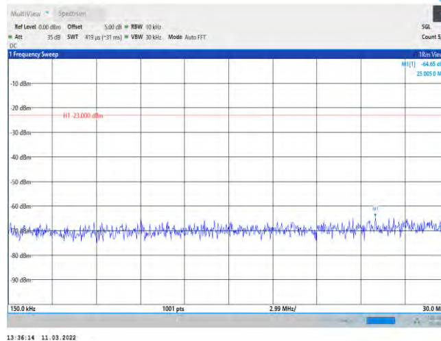
Band5-10MHz-QPSK-20450-1RB#0-Range2:0.15~30MHz
