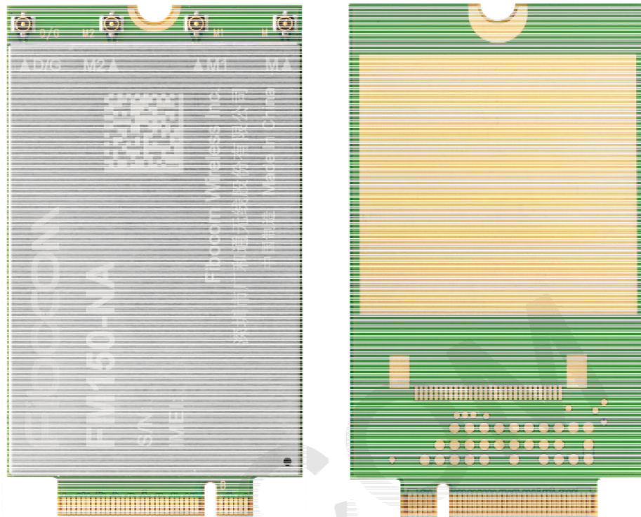
Figure 6-1 Module Appearance
