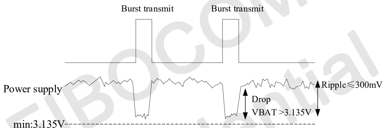
Figure 3-3 Power Supply Requirement
