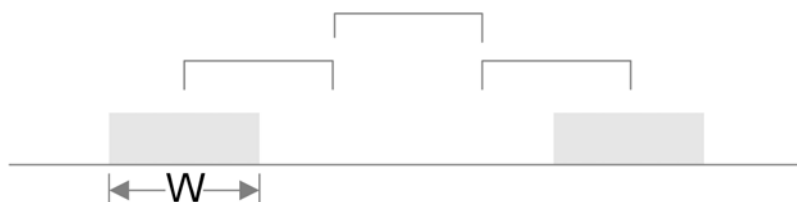
Figure 21. 3W principle
