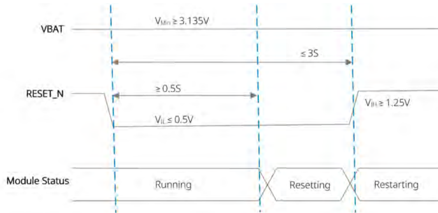
Figure 10. Reset sequence
