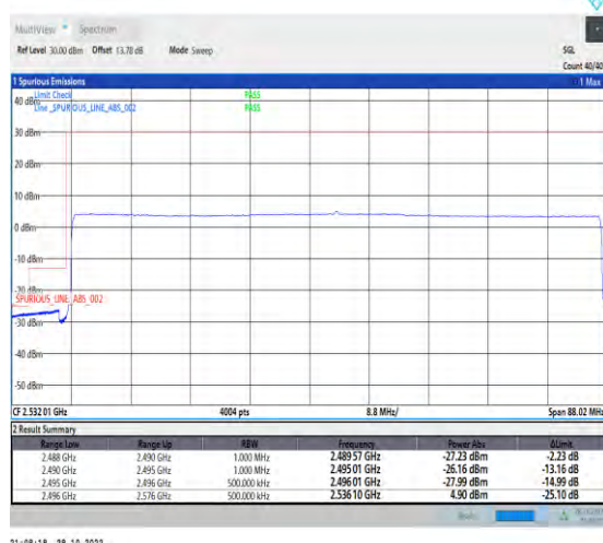
1-N41-PC2-30-80-L-6-CP-QPSK-Outer_Full-217@0-Ant1-1--PASS-see graph
