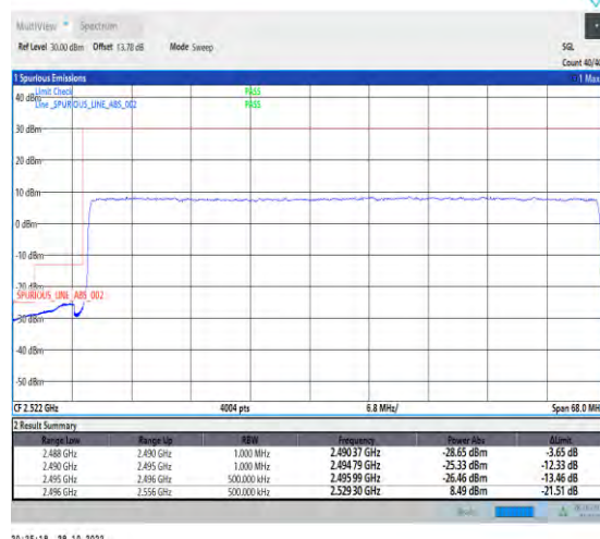
1-N41-PC2-30-60-L-3-DFT-PI2BPSK-Outer_Full-162@0-Ant1-1--PASS-see graph
