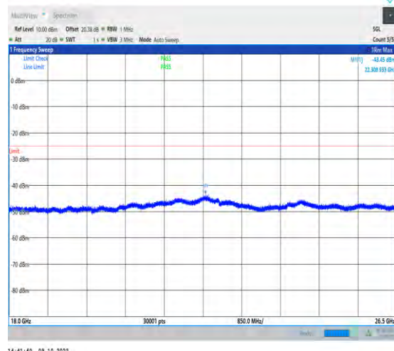
1-N41-PC2-30-100-L-1-DFT-QPSK-Edge_1RB_Left- 1@0-18000-26500-Ant1-22308.93--43.45--25-PASS
