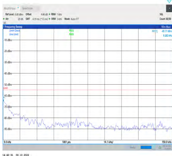
1-N41-PC2-30-100-M-1-DFT-QPSK-Edge_1RB_Left -1@0-0.009-0.15-Ant1-0.01--65.17--55-PASS
