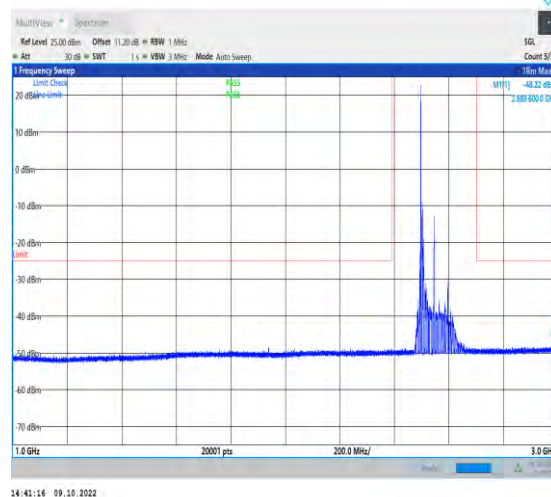
1-N41-PC2-30-100-L-1-DFT-QPSK-Edge_1RB_Left- 1@0-1000-3000-Ant1-2978.40--48.22--25-PASS
