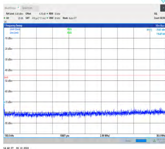
1-N41-PC2-30-100-M-1-DFT-QPSK-Edge_1RB_Left- 1@0-0.15-30-Ant1-0.18--73.87--45-PASS
