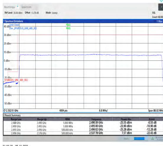
1-N41-PC2-30-80-L-3-DFT-PI2BPSK-Outer_Full-216@0-Ant1-1--PASS-see graph
