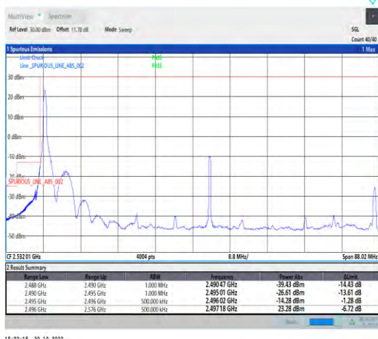
1-N41-PC2-30-80-L-1-DFT-PI2BPSK-Edge_1RB_Left-1@0-Ant1-1--PASS-see graph
