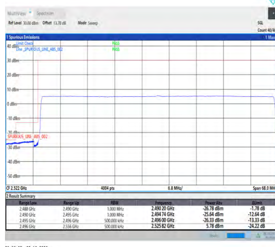
1-N41-PC2-30-60-L-6-CP-QPSK-Outer_Full-162@0-Ant1-1--PASS-see graph
