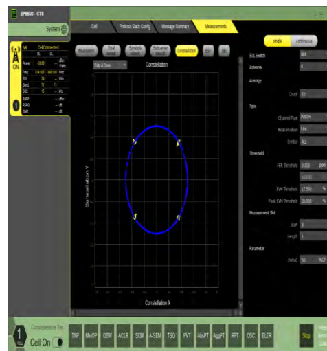
1-N71-15-20-M-2-DFT-QPSK-Outer_Full-100@0-Ant1-see graph-PASS
