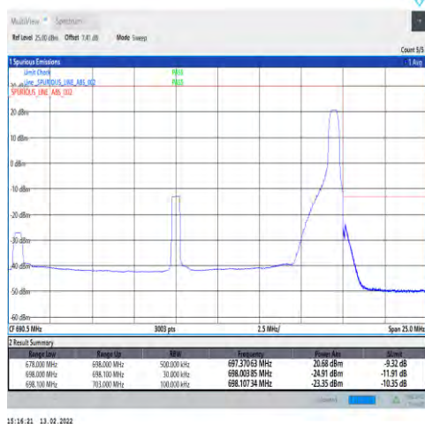
1-N71-PC3-15-20-H-5-CP-QPSK-Edge_1RB_Right-1@105-Ant1-PASS-see graph
