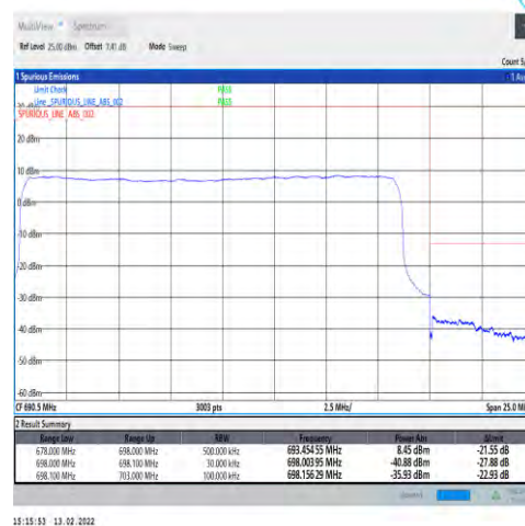
1-N71-PC3-15-20-H-3-DFT-PI2BPSK-Outer_Full-100@0-Ant1-PASS-see graph
