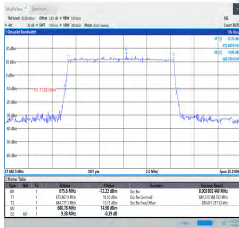
1-N71-PC3-15-10-M-1-DFT-QPSK-Outer_Ful I-50@0-Ant1-8.904-9.380-≤10-PASS
