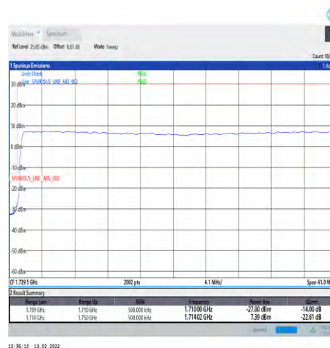
1-N66-PC3-15-40-L-3-DFT-PI2BPSK-Outer_Full-216@0-Ant1-seegraph-PASS-see graph
