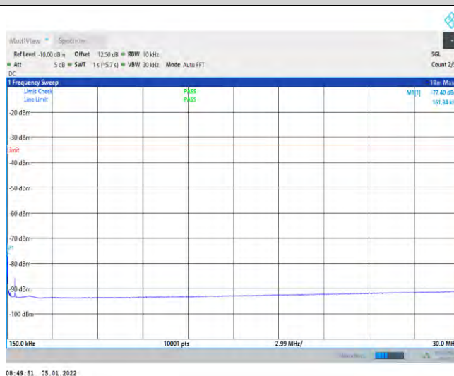
1-N66-PC3-15-40-M-4-DFT-QPSK-Edge_1RB_Left-1@0 -0.15-30--77.40--33-PASS
