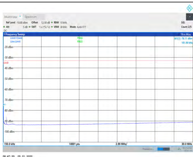
1-N66-PC3-15-40-L-4-DFT-QPSK-Edge_1RB_Left-1@0 -0.15-30--78.11--33-PASS
