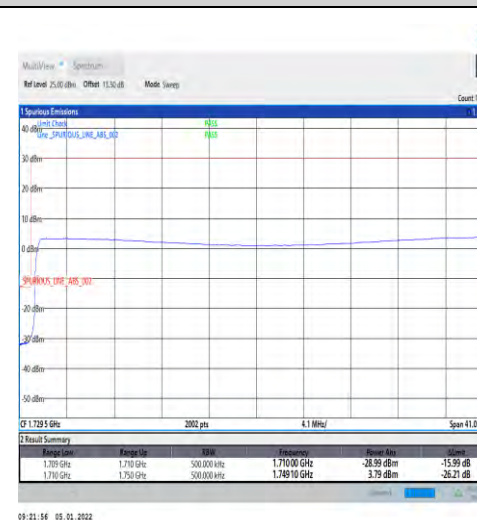
1-N66-PC3-15-40-L-6-CP-QPSK-Outer_Full-216@0-Ant1-seegraph-PASS-see graph
