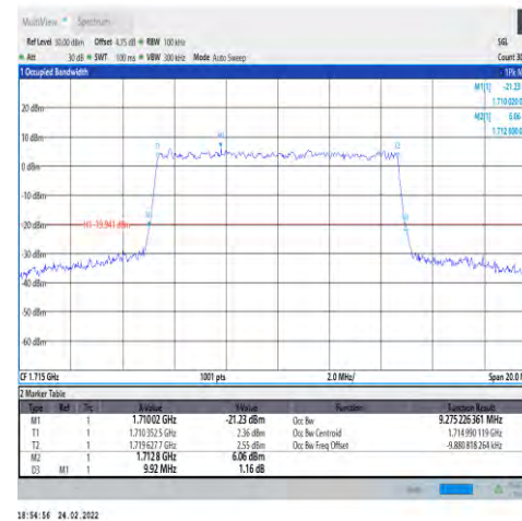
1-N66-PC3-15-10-L-9-CP-256QAM-Outer_Full-52@0-Ant1-9.275-9.920-≤10-PASS
