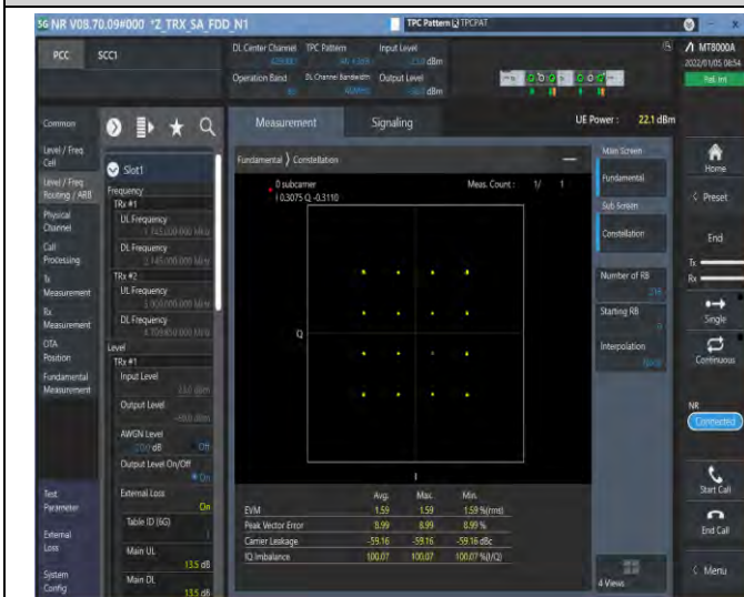
1-N66-PC3-15-40-M-3-DFT-16QAM-Outer_Full-216@0- see graph-PASS
