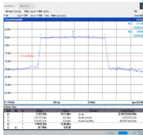
1-N66-PC3-15-25-M-3-DFT-16QAM-Outer_Full-128@0-Ant1-22.765-24.100-≤25-PASS
