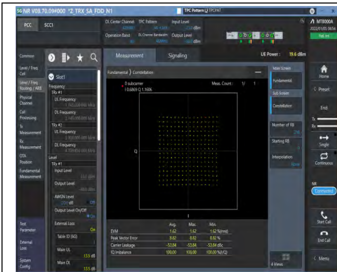
1-N66-PC3-15-40-M-5-DFT-256QAM-Outer_Full-216@0 -see graph-PASS
