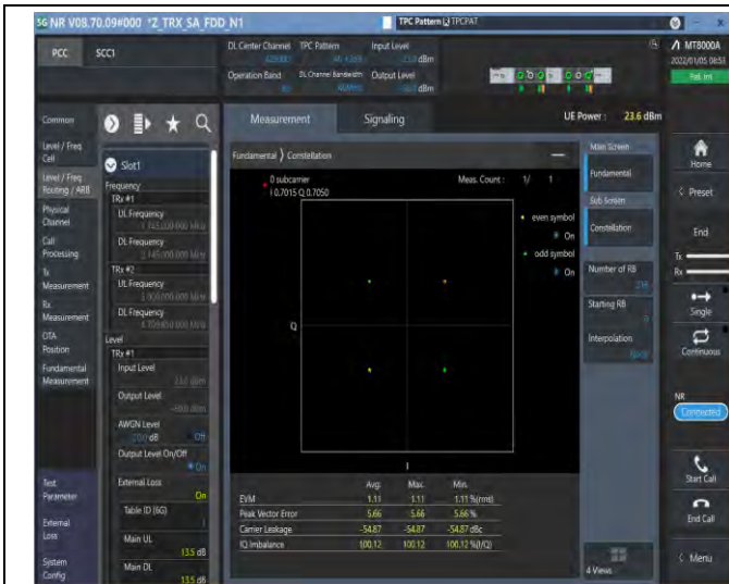
1-N66-PC3-15-40-M-1-DFT-PI2BPSK-Outer_Full-216@ 0-see graph-PASS
