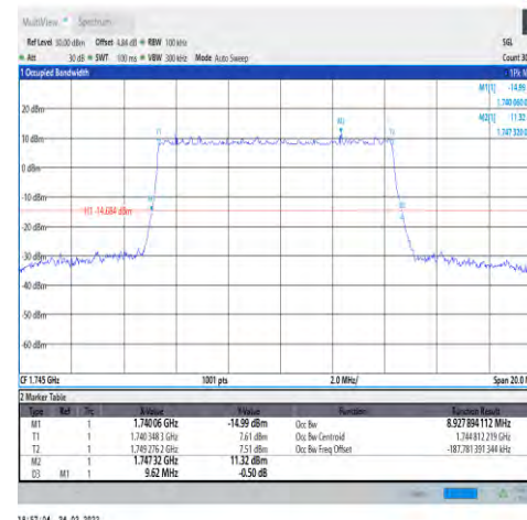
1-N66-PC3-15-10-M-4-DFT-64QAM-Outer_Full-50@0-Ant1-8.928-9.620-≤10-PASS
