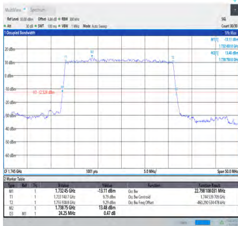
1-N66-PC3-15-25-M-2-DFT-PI2BPSK-Outer_Full-128@0-Ant1-22.798-24.250-≤25-PASS
