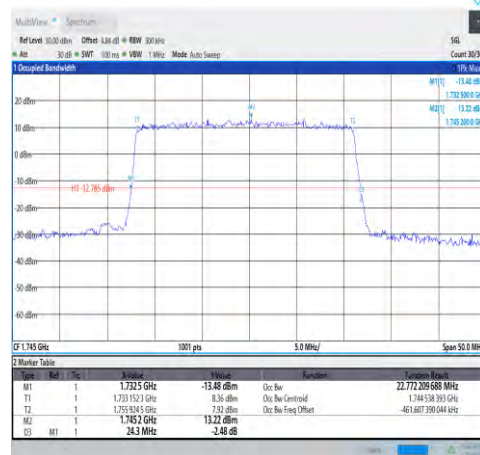
1-N66-PC3-15-25-M-1-DFT-QPSK-Outer_Full-128@0-Ant1-22.772-24.300-≤25-PASS
