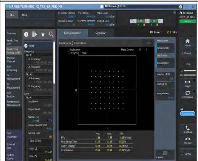
1-N66-PC3-15-40-M-4-DFT-64QAM-Outer_Full-216 @0-see graph-PASS
