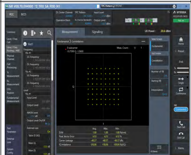
1-N66-PC3-15-40-M-8-CP-64QAM-Outer_Full-216@ 0-see graph-PASS
