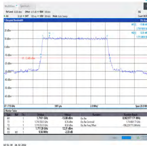
1-N66-PC3-15-10-L-1-DFT-QPSK-Outer_Full-50@0-Ant1-8.903-9.560-≤10-PASS
