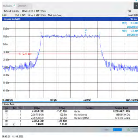
1-N41-30-10-H-5-DFT-256QAM-Outer_Full-2 4@0-Ant1-8.567-9.400-≤10-PASS
