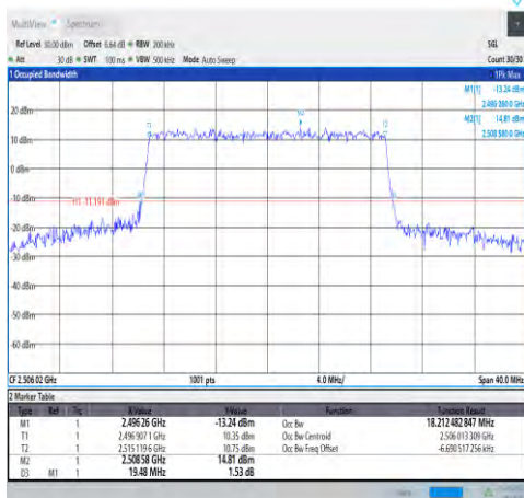
1-N41-30-20-L-7-CP-16QAM-Outer_Full-51 @0-Ant1-18.212-19.480-≤20-PASS
