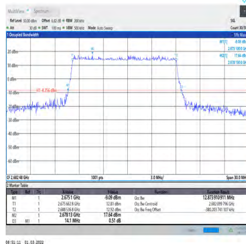
1-N41-30-15-H-3-DFT-16QAM-Outer_Full-36 @0-Ant1-12.874-14.100-≤15-PASS
