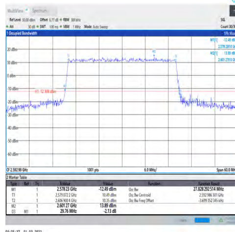
1-N41-30-30-M-6-CP-QPSK-Outer_Full-78@ 0-Ant1-27.828-29.760-≤30-PASS
