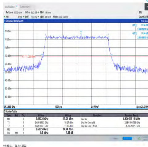
1-N41-30-10-H-4-DFT-64QAM-Outer_Full-24 @0-Ant1-8.601-9.500-≤10-PASS
