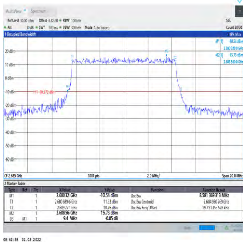
1-N41-30-10-H-3-DFT-16QAM-Outer_Full-24 @0-Ant1-8.581-9.400-≤10-PASS
