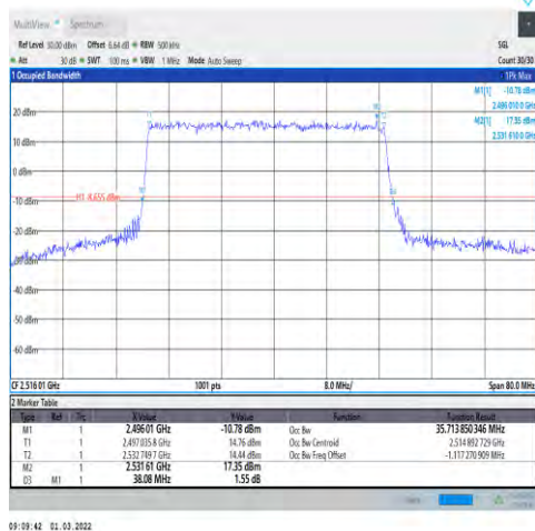
1-N41-30-40-L-1-DFT-QPSK-Outer_Full-100 @0-Ant1-35.714-38.080-≤40-PASS
