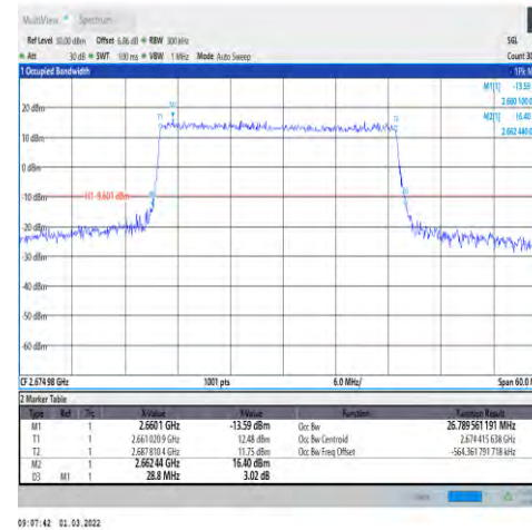
1-N41-30-30-H-3-DFT-16QAM-Outer_Full-75 @0-Ant1-26.79-28.800-≤30-PASS
