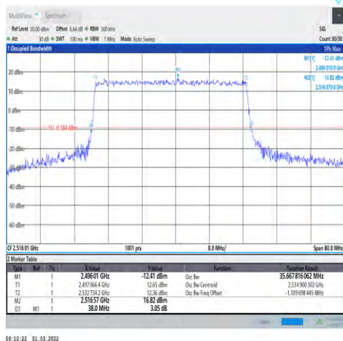
1-N41-30-40-L-3-DFT-16QAM-Outer_Full-10 0@0-Ant1-35.668-38.000-≤40-PASS
