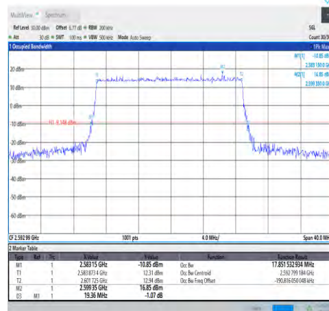
1-N41-30-20-M-1-DFT-QPSK-Outer_Full-50 @0-Ant1-17.852-19.360-≤20-PASS
