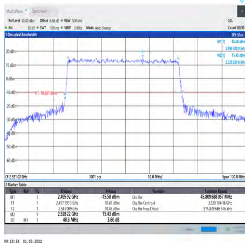
1-N41-30-50-L-4-DFT-64QAM-Outer_Full-12 8@0-Ant1-45.81-48.600-≤50-PASS
