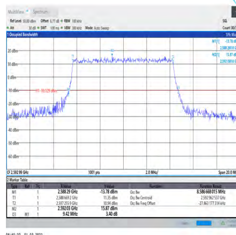
1-N41-30-10-M-3-DFT-16QAM-Outer_Full-24 @0-Ant1-8.587-9.420-≤10-PASS
