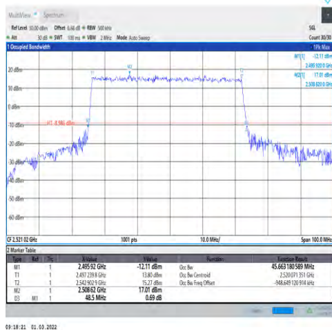
1-N41-30-50-L-2-DFT-PI2BPSK-Outer_Full-1 28@0-Ant1-45.663-48.500-≤50-PASS
