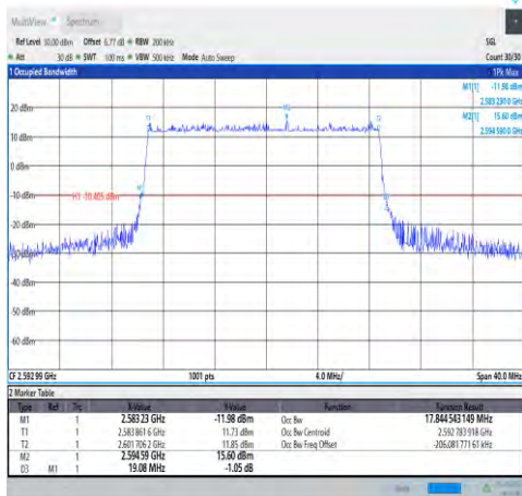
1-N41-30-20-M-4-DFT-64QAM-Outer_Full-50@0-Ant1-17.845-19.080-≤20-PASS
