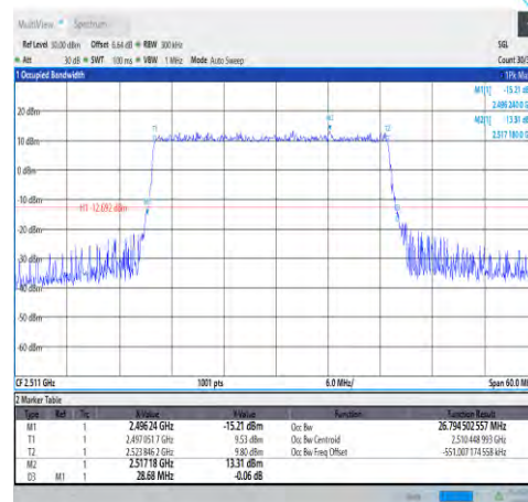
1-N41-30-30-L-5-DFT-256QAM-Outer_Full-7 5@0-Ant1-26.795-28.680-≤30-PASS
