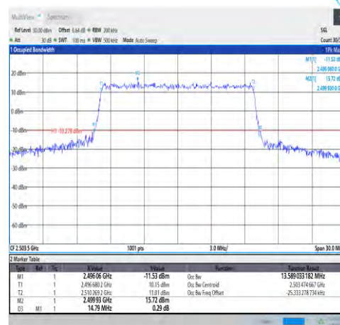
1-N41-30-15-L-7-CP-16QAM-Outer_Full-38 @0-Ant1-13.589-14.790-≤15-PASS
