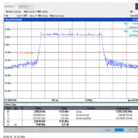
1-N41-30-20-L-4-DFT-64QAM-Outer_Full-50 @0-Ant1-17.835-19.080-≤20-PASS
