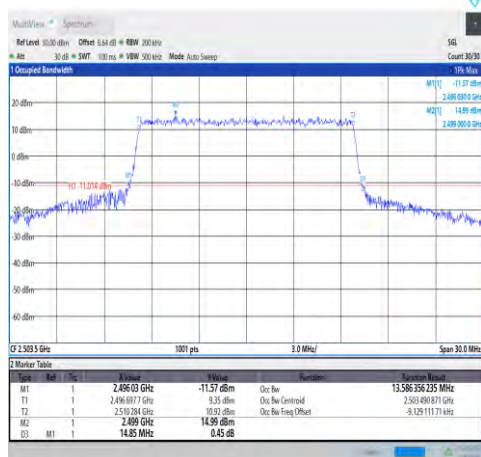
1-N41-30-15-L-6-CP-QPSK-Outer_Full-38@ 0-Ant1-13.586-14.850-≤15-PASS
