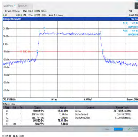
1-N41-30-30-H-4-DFT-64QAM-Outer_Full-75 @0-Ant1-26.725-28.680-≤30-PASS
