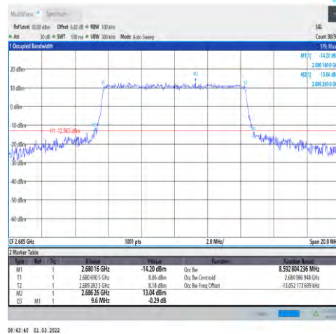
1-N41-30-10-H-6-CP-QPSK-Outer_Full-24@ 0-Ant1-8.593-9.600-≤10-PASS
