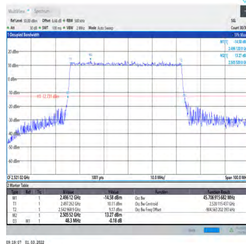
1-N41-30-50-L-5-DFT-256QAM-Outer_Full-1 28@0-Ant1-45.707-48.300-≤50-PASS
