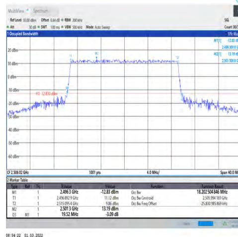
1-N41-30-20-L-6-CP-QPSK-Outer_Full-51@ 0-Ant1-18.203-19.520-≤20-PASS
