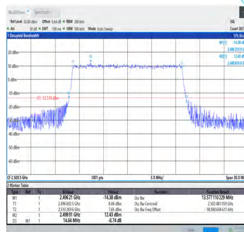
1-N41-30-15-L-9-CP-256QAM-Outer_Full-38 @0-Ant1-13.577-14.640-≤15-PASS
