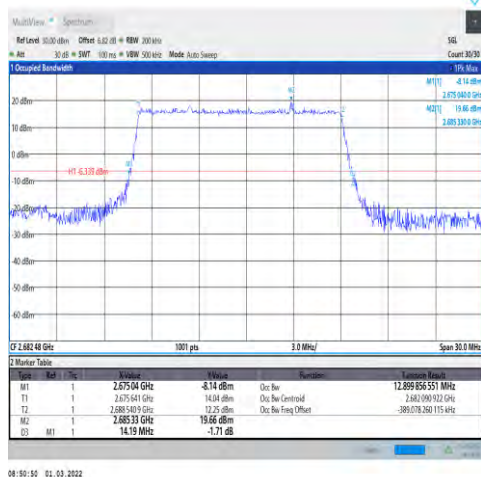
1-N41-30-15-H-2-DFT-PI2BPSK-Outer_Full-3 6@0-Ant1-12.9-14.190-≤15-PASS
