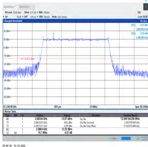
1-N41-30-15-M-9-CP-256QAM-Outer_Full-38 @0-Ant1-13.549-14.700-≤15-PASS
