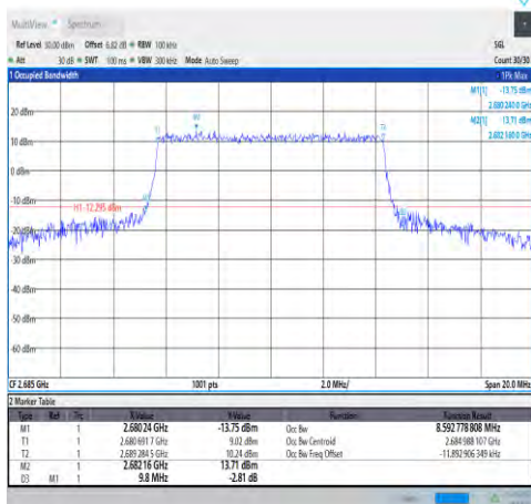
1-N41-30-10-H-7-CP-16QAM-Outer_Full-24 @0-Ant1-8.593-9.800-≤10-PASS
