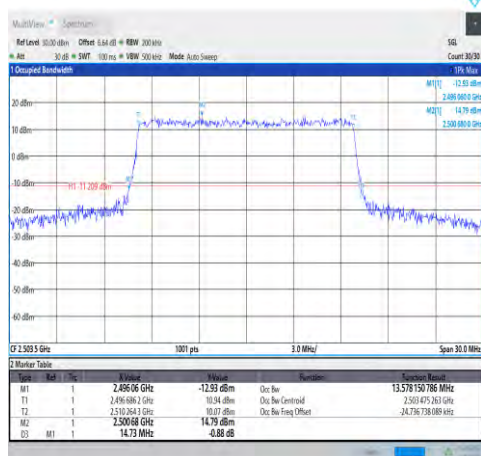
1-N41-30-15-L-8-CP-64QAM-Outer_Full-38 @0-Ant1-13.578-14.730-≤15-PASS
