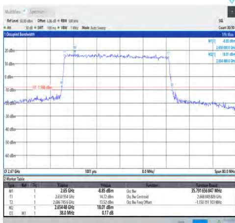
1-N41-30-40-H-1-DFT-QPSK-Outet_Full-100 @0-Ant1-35.792-38.000-≤40-PASS
