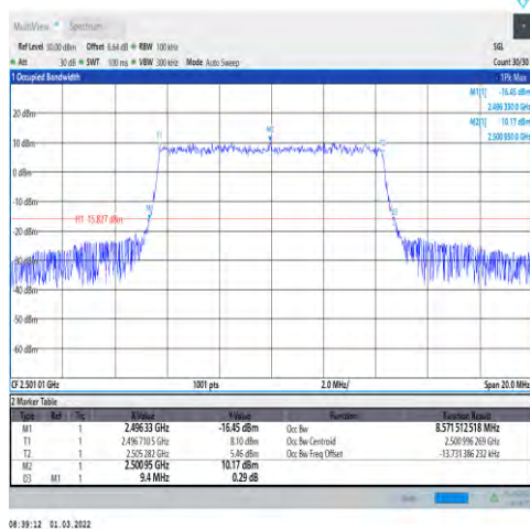
1-N41-30-10-L-9-CP-256QAM-Outer_Full-24 @0-Ant1-8.572-9.400-≤10-PASS
