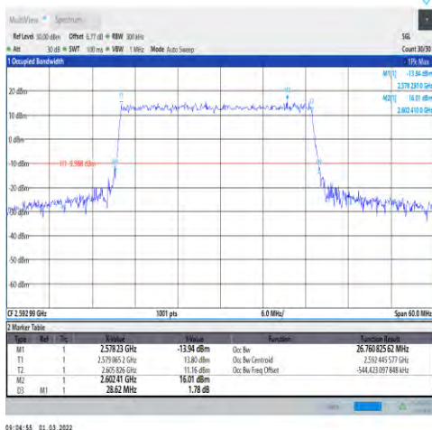
1-N41-30-30-M-3-DFT-16QAM-Outer_Full-75 @0-Ant1-26.761-28.620-≤30-PASS
