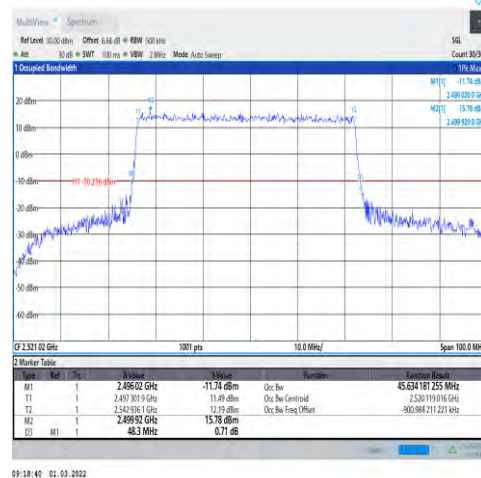
1-N41-30-50-L-3-DFT-16QAM-Outer_Full-12 8@0-Ant1-45.634-48.300-≤50-PASS
