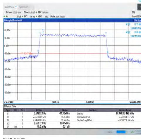
1-N41-30-40-H-6-CP-QPSK-Outer_Full-106@0-Ant1-37.895-40.000-≤40-PASS
