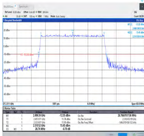
1-N41-30-30-L-4-DFT-64QAM-Outer_Full-75 @0-Ant1-26.766-28.740-≤30-PASS
