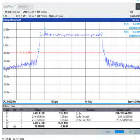
1-N41-30-20-L-3-DFT-16QAM-Outer_Full-50 @0-Ant1-17.863-19.080-≤20-PASS
