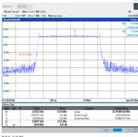
1-N41-30-30-M-5-DFT-256QAM-Outer_Full-7 5@0-Ant1-26.798-28.560-≤30-PASS
