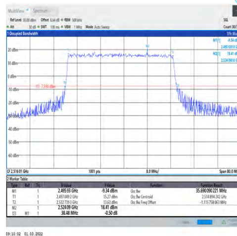
1-N41-30-40-L-2-DFT-PI2BPSK-Outer_Full-1 00@0-Ant1-35.69-38.480-≤40-PASS
