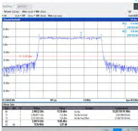
1-N41-30-20-L-9-CP-256QAM-Outer_Full-51 @0-Ant1-18.203-19.560-≤20-PASS
