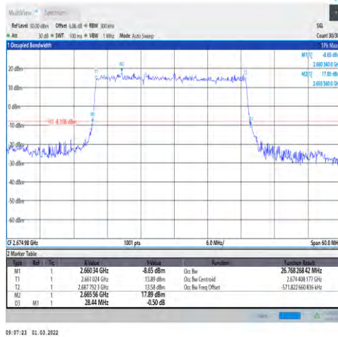
1-N41-30-30-H-2-DFT-PI2BPSK-Outer_Full-75 5@0-Ant1-26.768-28.440-≤30-PASS
