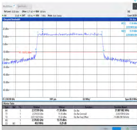
1-N41-30-40-M-8-CP-64QAM-Outet_Full-106 @0-Ant1-37.888-40.000-≤40-PASS
