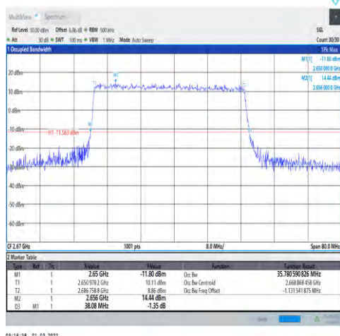
1-N41-30-40-H-5-DFT-256QAM-Outer_Full-100@0-Ant1-35.781-38.080-≤40-PASS
