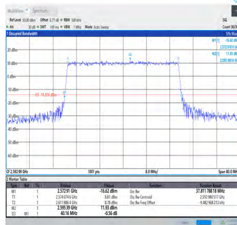
1-N41-30-40-M-9-CP-256QAM-Outet_Full-106 @0-Ant1-37.812-40.160-≤40-PASS
