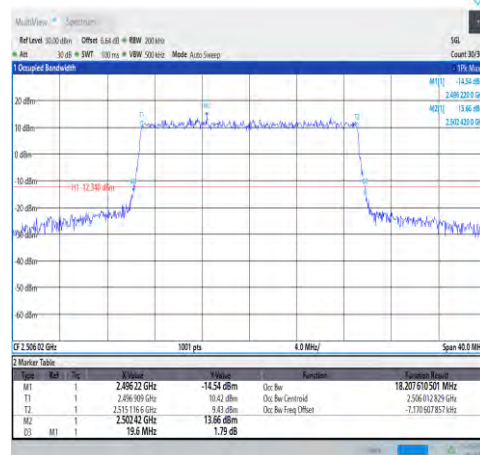
1-N41-30-20-L-8-CP-64QAM-Outer_Full-51 @0-Ant1-18.208-19.600-≤20-PASS
