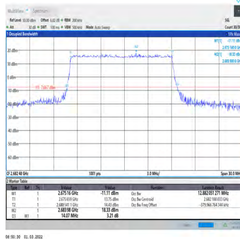
1-N41-30-15-H-1-DFT-QPSK-Outer_Full-36 @0-Ant1-12.882-14.070-≤15-PASS
