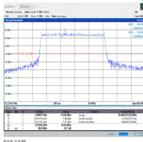
1-N41-30-40-L-4-DFT-64QAM-Outer_Full-10 0@0-Ant1-35.695-38.000-≤40-PASS
