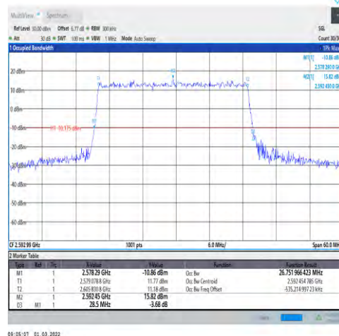
1-N41-30-30-M-4-DFT-64QAM-Outer_Full-75 @0-Ant1-26.752-28.500-≤30-PASS
