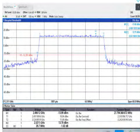
1-N41-30-30-L-6-CP-QPSK-Outer_Full-78@ 0-Ant1-27.794-29.700-≤30-PASS
