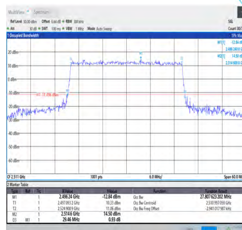
1-N41-30-30-L-7-CP-16QAM-Outer_Full-78 @0-Ant1-27.808-29.460-≤30-PASS
