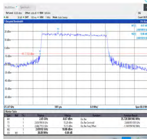
1-N41-30-40-H-2-DFT-PI2BPSK-Outet_Full-100 @0-Ant1-35.728-38.080-≤40-PASS
