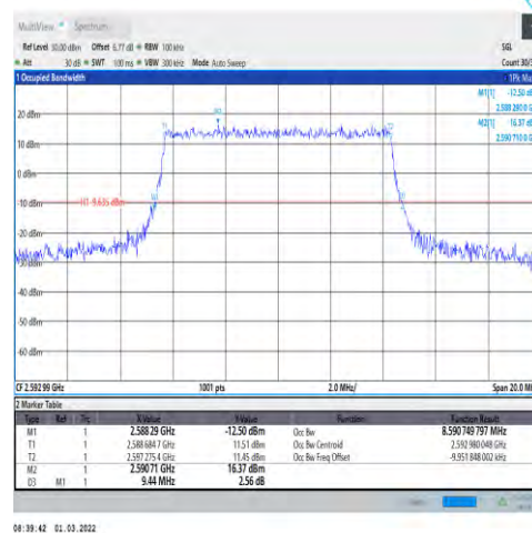
1-N41-30-10-M-1-DFT-QPSK-Outer_Full-24 @0-Ant1-8.591-9.440-≤10-PASS
