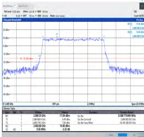
1-N41-30-10-H-9-CP-256QAM-Outer_Full-24 @0-Ant1-8.589-9.560-≤10-PASS
