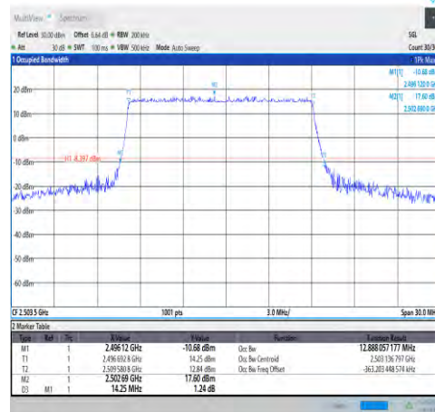
1-N41-30-15-L-1-DFT-QPSK-Outer_Full-36@ 0-Ant1-12.888-14.250-≤15-PASS
