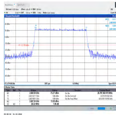
1-N41-30-30-H-5-DFT-256QAM-Outer_Full-75 5@0-Ant1-26.781-28.320-≤30-PASS
