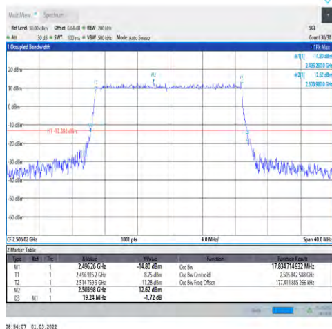
1-N41-30-20-L-5-DFT-256QAM-Outer_Full-5 0@0-Ant1-17.835-19.240-≤20-PASS
