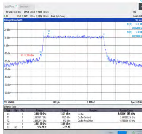
1-N41-30-10-H-8-CP-64QAM-Outer_Full-24 @0-Ant1-8.603-9.540-≤10-PASS
