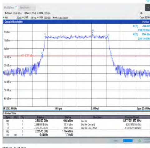
1-N41-30-10-M-2-DFT-PI2BPSK-Outer_Full-24 @0-Ant1-8.577-9.400-≤10-PASS
