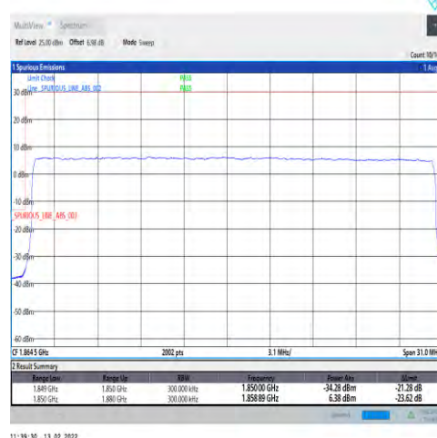
1-N25-15-30-L-3-DFT-PI2BPSK-Outer_Full-160@0-Ant1-seegraph-PASS-see graph
