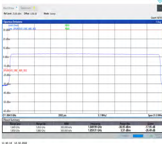
1-N25-15-30-L-6-CP-QPSK-Outer_Full-160@0-Ant1-seegraph-PASS-see graph
