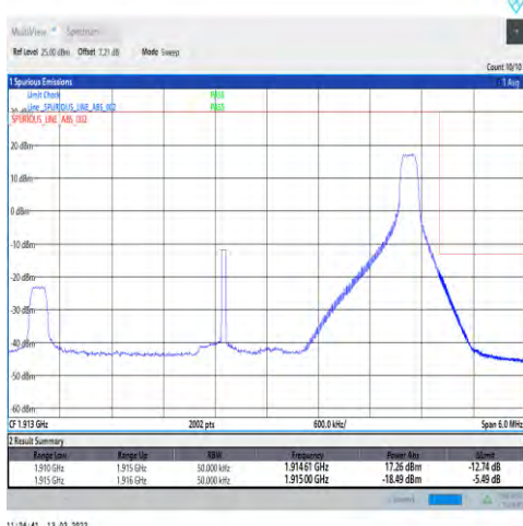
1-N25-15-5-H-5-CP-QPSK-Edge_1RB_Right-1@24-Ant1-seegraph-PASS-see graph
