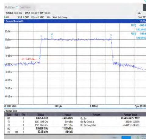
1-N25-PC3-15-40-M-7-CP-16QAM-Outer_Full I-216@0-Ant1-38.643-40.480-≤40-PASS
