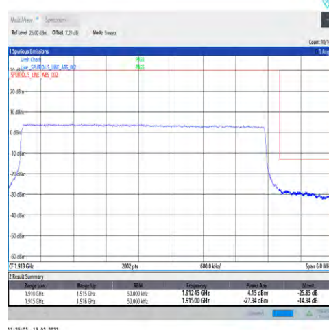
1-N25-15-5-H-6-CP-QPSK-Outer_Full-25@0-Ant1-seegraph-PASS-see graph
