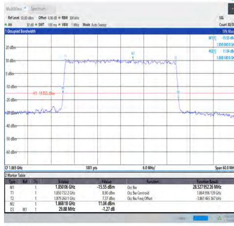
1-N25-PC3-15-30-L-4-DFT-64QAM-Outer_Fu II-160@0-Ant1-28.528-29.880-≤30-PASS
