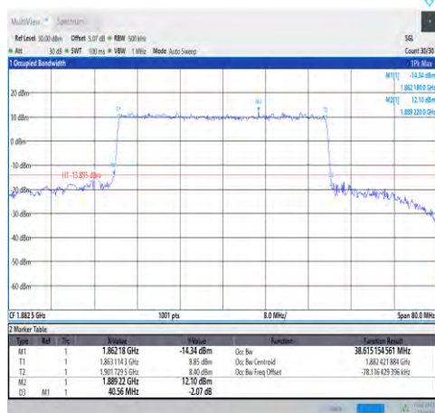
1-N25-PC3-15-40-M-6-CP-QPSK-Outer_Full- 216@0-Ant1-38.615-40.560-≤40-PASS
