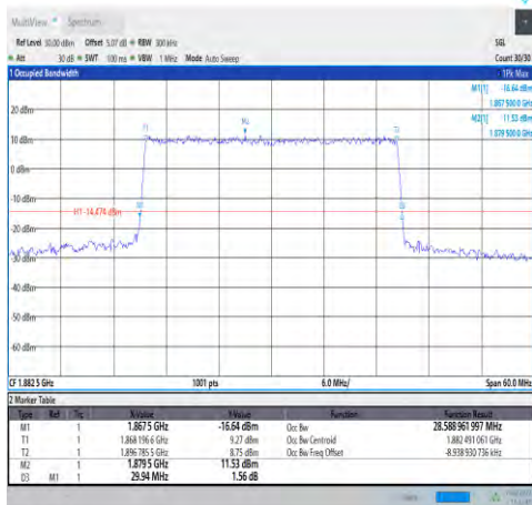
1-N25-PC3-15-30-M-3-DFT-16QAM-Outter_Full-160@0-Ant1-28.589-29.940-≤30-PASS
