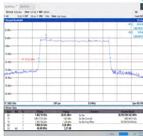
1-N25-PC3-15-40-M-9-CP-256QAM-Outer_F ull-216@0-Ant1-38.593-40.480-≤40-PASS
