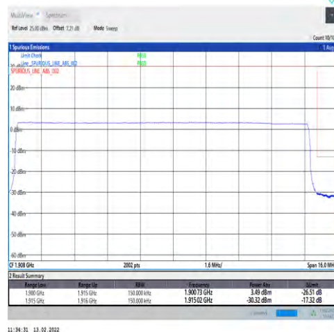
1-N25-15-15-H-6-CP-QPSK-Outer_Full-79@0-Ant1-seegraph-PASS-see graph
