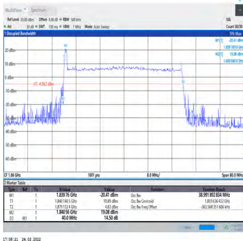
1-N25-PC3-15-40-L-9-CP-256QAM-Outer_F ull-216@0-Ant1-39.028-40.000-≤40-PASS
