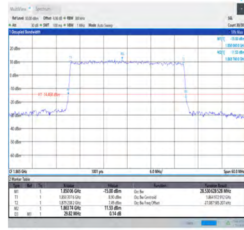
1-N25-PC3-15-30-L-3-DFT-16QAM-Outer_Fu II-160@0-Ant1-28.531-29.820-≤30-PASS
