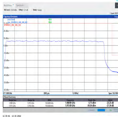
1-N25-15-15-H-3-DFT-PI2BPSK-Outer_Full-75@0-Ant1-seegraph-PASS-see graph
