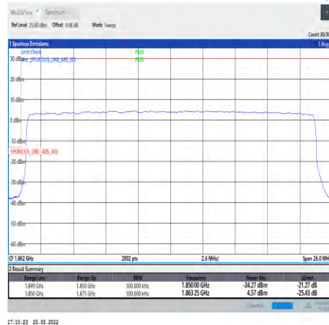
1-N25-PC3-15-25-L-3-DFT-PI2BPSK-Outer_Full-128@0-Ant1-seegraph-PASS-see graph
