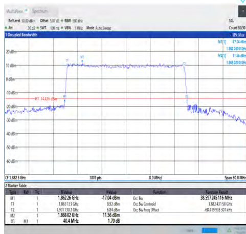
1-N25-PC3-15-40-M-8-CP-64QAM-Outer_Full I-216@0-Ant1-38.597-40.400-≤40-PASS
