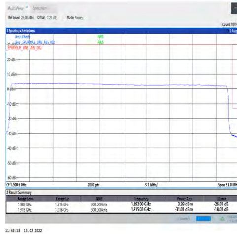
1-N25-15-30-H-6-CP-QPSK-Outer_Full-160@0-Ant1-seegraph-PASS-see graph
