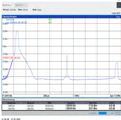
1-N25-15-10-L-4-CP-QPSK-Edge_1RB_Left-1@0-Ant1-seegraph-PASS-see graph
