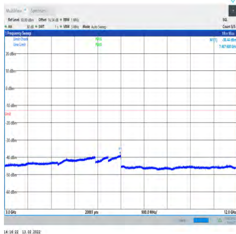
1-N25-15-40-L-1-DFT-PI2BPSK-Inner_1RB_ Left-1@1-3000-12000-Ant1--38.44--13-PASS
