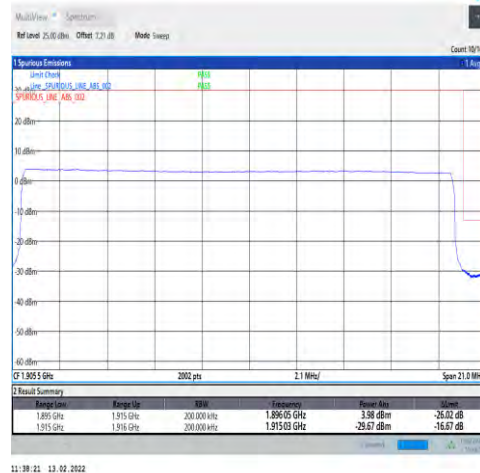
1-N25-15-20-H-6-CP-QPSK-Outer_Full-106@0-Ant1-seegraph-PASS-see graph
