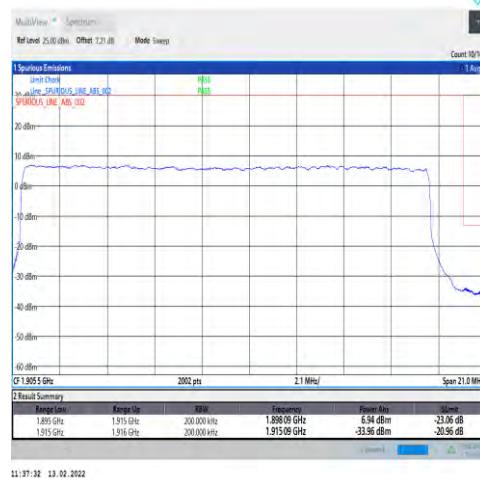
1-N25-15-20-H-3-DFT-PI2BPSK-Outer_Full-100@0-Ant1-seegraph-PASS-see graph
