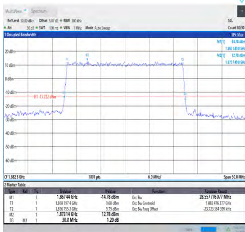
1-N25-PC3-15-30-M-1-DFT-QPSK-Outter_Ful I-160@0-Ant1-28.558-30.000-≤30-PASS
