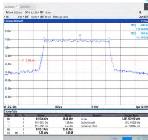
1-N25-PC3-15-5-H-4-DFT-64QAM-Outer_Ful I-25@0-Ant1-4.463-4.820-≤5-PASS
