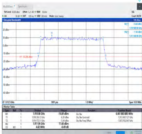
1-N25-PC3-15-5-H-3-DFT-16QAM-Outer_Ful I-25@0-Ant1-4.462-4.820-≤5-PASS
