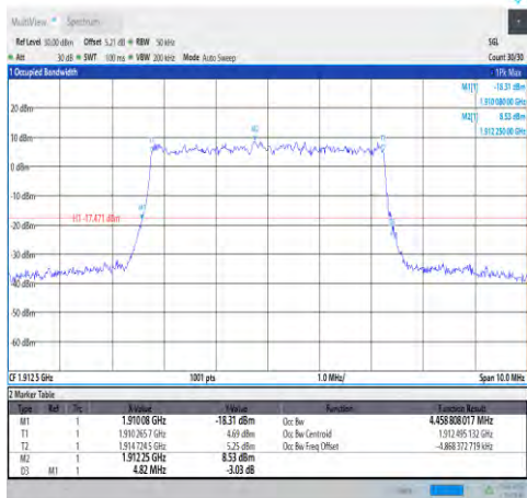
1-N25-PC3-15-5-H-5-DFT-256QAM-Outer_F ull-25@0-Ant1-4.459-4.820-≤5-PASS
