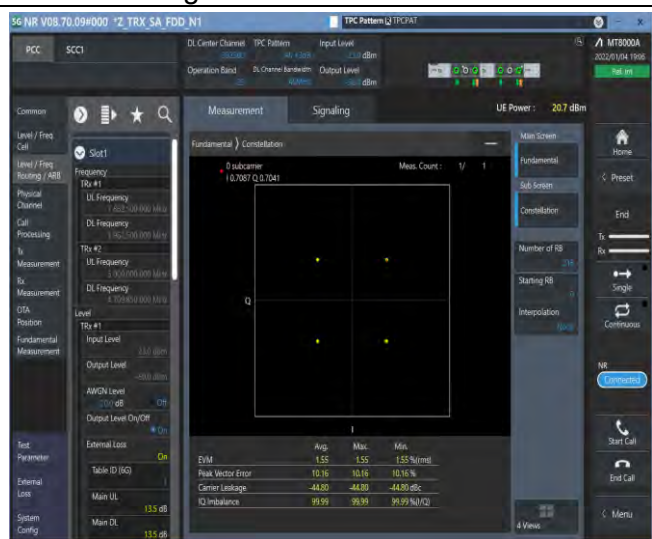
1-N25-15-40-M-6-CP-QPSK-Outer_Full-216@0-see graph-PASS
