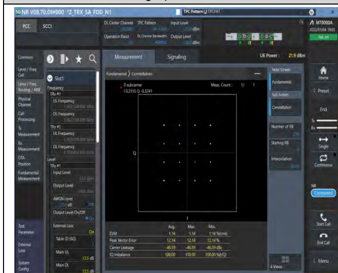
1-N25-15-40-M-3-DFT-16QAM-Out_Full-216@0-see graph-PASS
