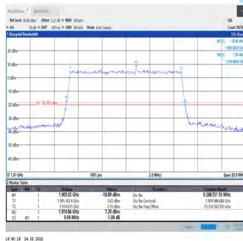
1-N25-PC3-15-10-H-9-CP-256QAM-Outer_Full ull-52@0-Ant1-9.289-9.940-≤10-PASS
