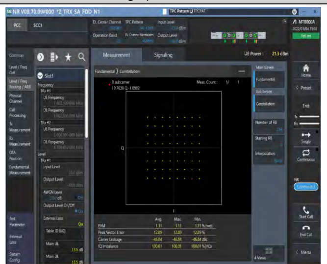
1-N25-15-40-M-4-DFT-64QAM-Out_Full-216@0-see graph-PASS
