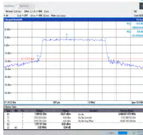
1-N25-PC3-15-5-H-6-CP-QPSK-Outer_Full-2 5@0-Ant1-4.469-5.030-≤5-PASS
