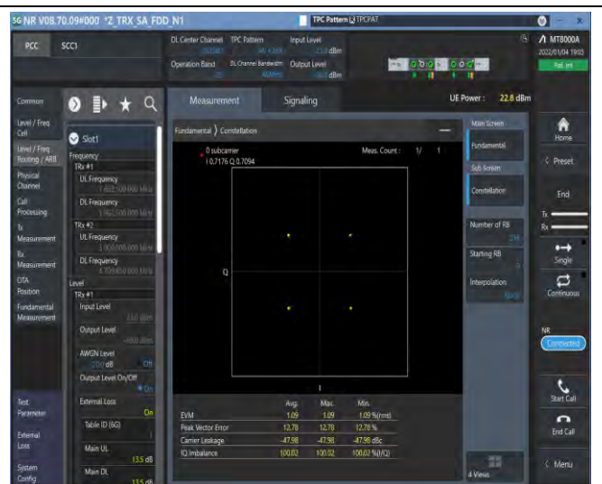
1-N25-15-40-M-2-DFT-QPSK-Out_Full-216@0-see graph-PASS
