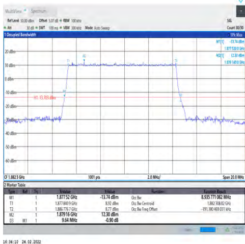
1-N25-PC3-15-10-M-1-DFT-QPSK-Outter_Ful I-50@0-Ant1-8.936-9.640-≤10-PASS
