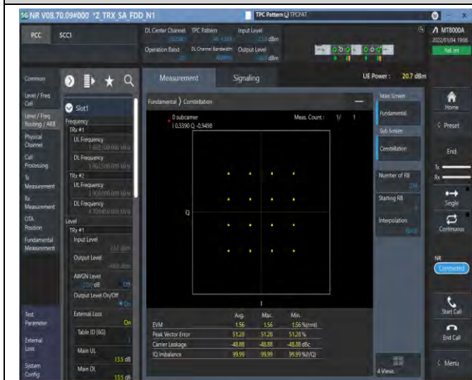
1-N25-15-40-M-7-CP-16QAM-Outer_Full-216@0-see graph-PASS
