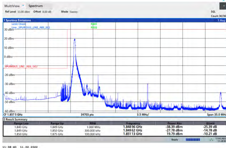
2-2-5MHz-20MHz-16QAM-16QAM-18633-18750-1RB#0-0RB#0
