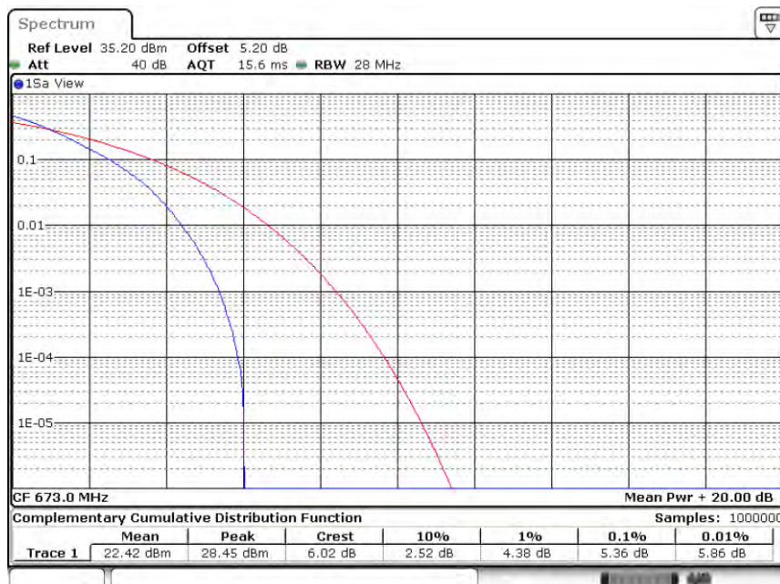
Band71-20MHz-QPSK-133222-100RB#0
