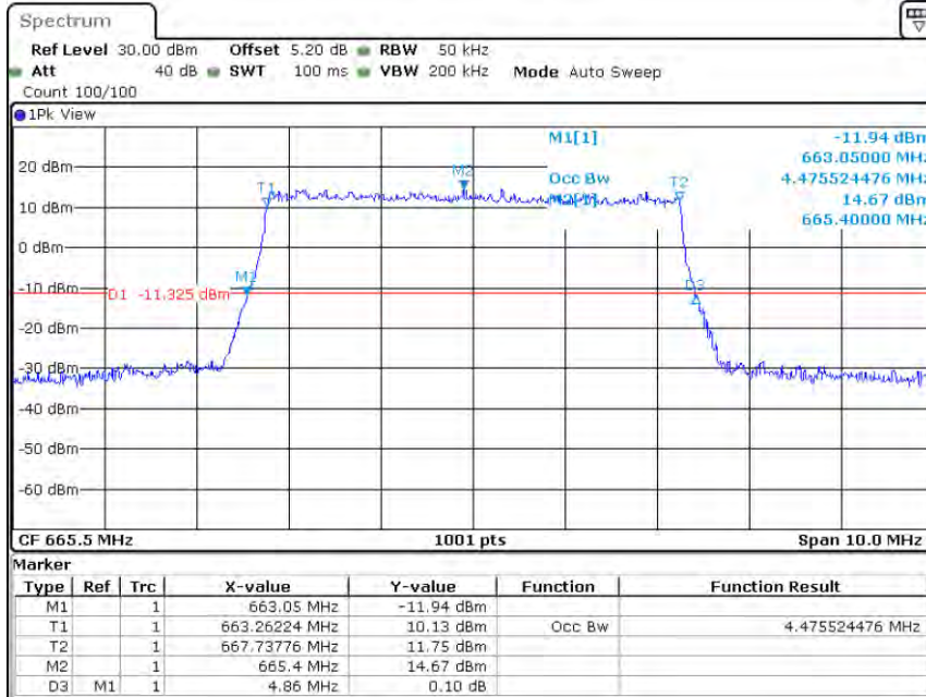
Band71-5MHz-QPSK-133147-25RB#0-4.476
