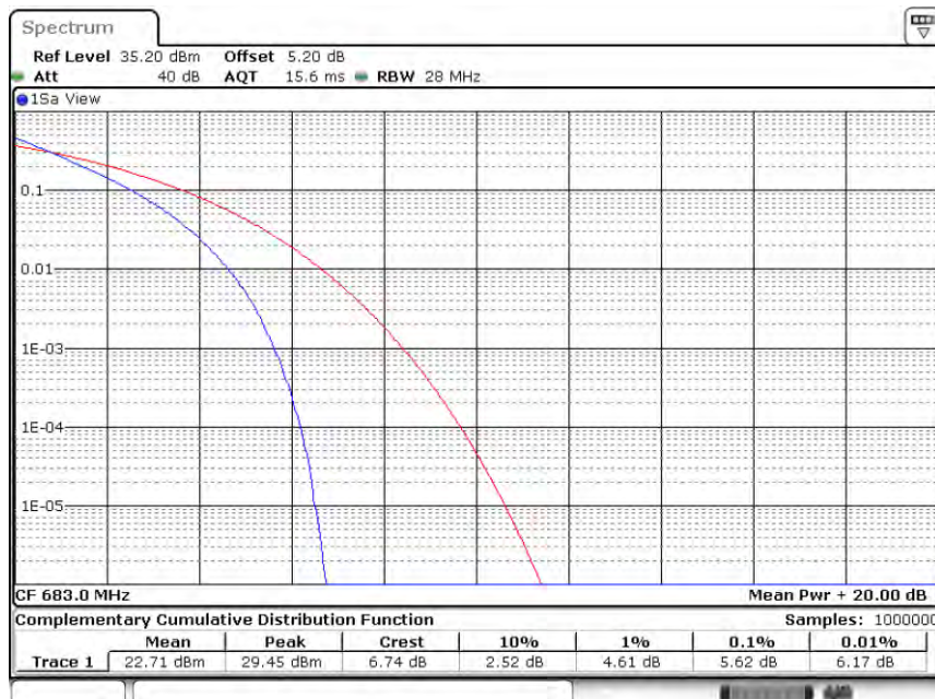
Band71-20MHz-QPSK-133322-100RB#0
