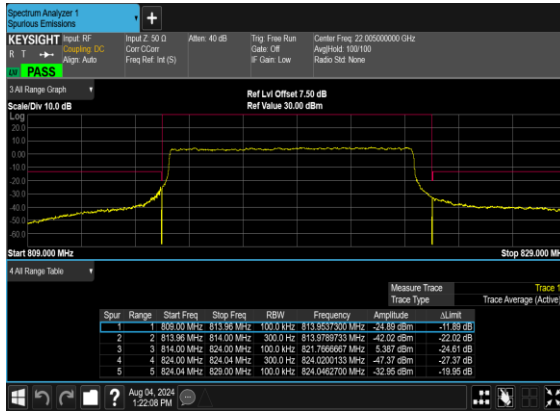
N26(10M)_DFT-s- OFDM_QPSK_Outer_Full_Mid_CH
