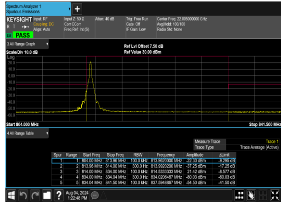
N26(20M)_DFT-s- OFDM_BPSK_Edge_1RB_Left_Mid_CH
