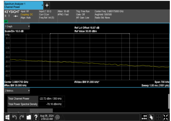
N77(100M)_DFT-s- OFDM_BPSK_Edge_1RB_Right_High_CH_CHP_PASS
