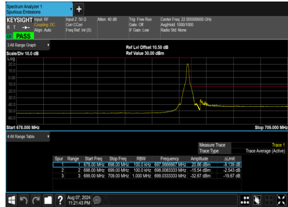
N71(10M)_DFT-s- OFDM_BPSK_Edge_1RB_Right_High_CH
