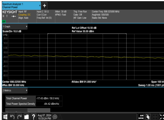
N71(5M)_DFT-s- OFDM_BPSK_Edge_1RB_Right_High_CH_ch P_PASS
