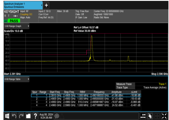
N41(50M)_DFT-s- OFDM_BPSK_Edge_1RB_Left_Low_CH
