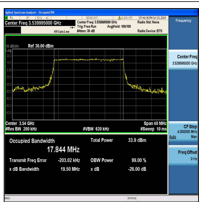
NTNV_N77-3450-3550_PC2_30_20_H_TID2_Ant1#1
