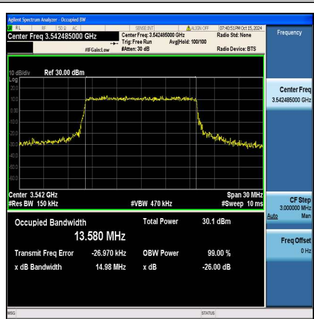
NTNV_N77-3450-3550_PC2_30_15_H_TID6_Ant1#1
