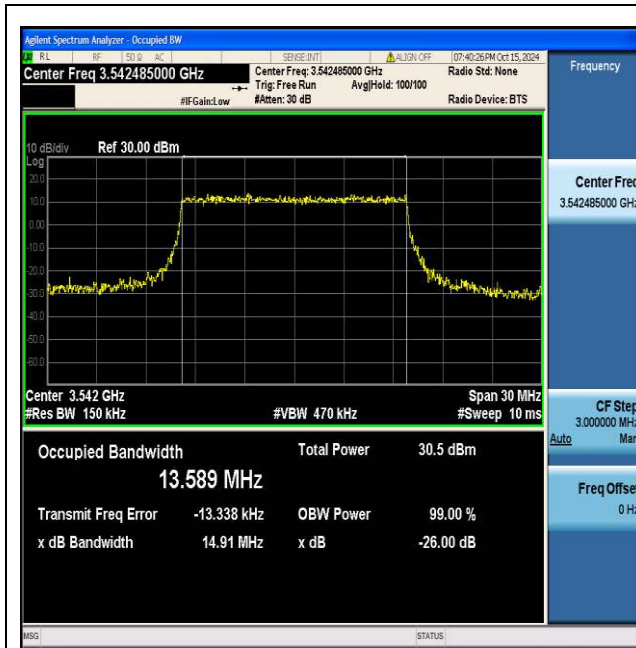
NTNV_N77-3450-3550_PC2_30_15_H_TID5_Ant1#1
