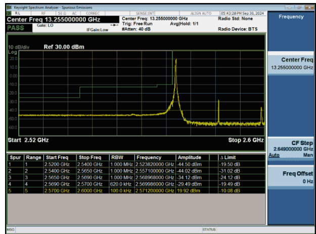
NTNV-n38-PC3-30-30-L-DFT-BPSK-Edge_1RB_Left-PASS
