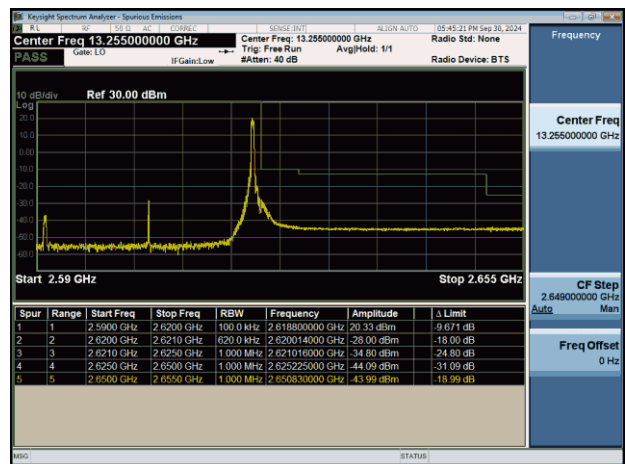
NTNV-n38-PC3-30-30-H-DFT-BPSK-Edge_1RB_Right-PASS
