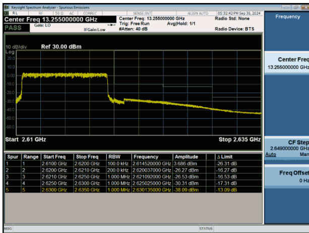
NTNV-n38-PC3-30-10-H-CP-QPSK-Outet_Full-PASS
