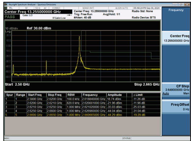
NTNV-n38-PC3-30-40-H-DFT-BPSK-Edge_1RB_Right-PASS
