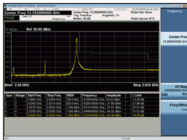
NTNV-n38-PC3-30-30-H-CP-QPSK-Edge_1RB_Right-PASS
