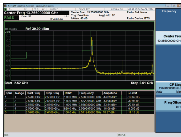
NTNV-n38-PC3-30-40-L-DFT-BPSK-Edge_1RB_Left-PASS
