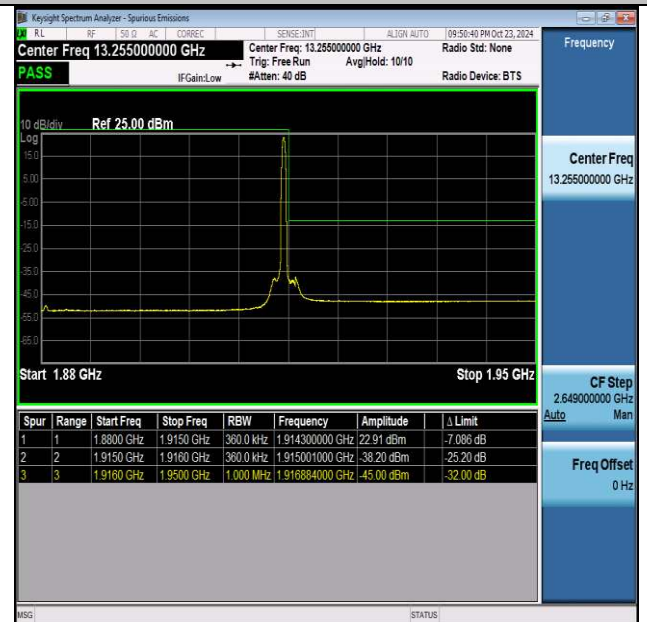
NTNV-n25-PC3-15-35-H-DFT-PI2BPSK-Edge_1RB_Right-PASS
