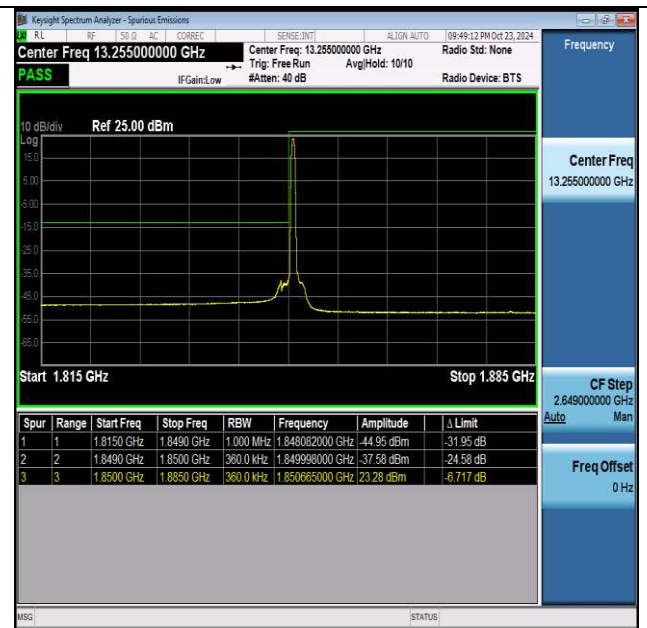
NTNV-n25-PC3-15-35-L-DFT-PI2BPSK-Edge_1RB_Left-PASS
