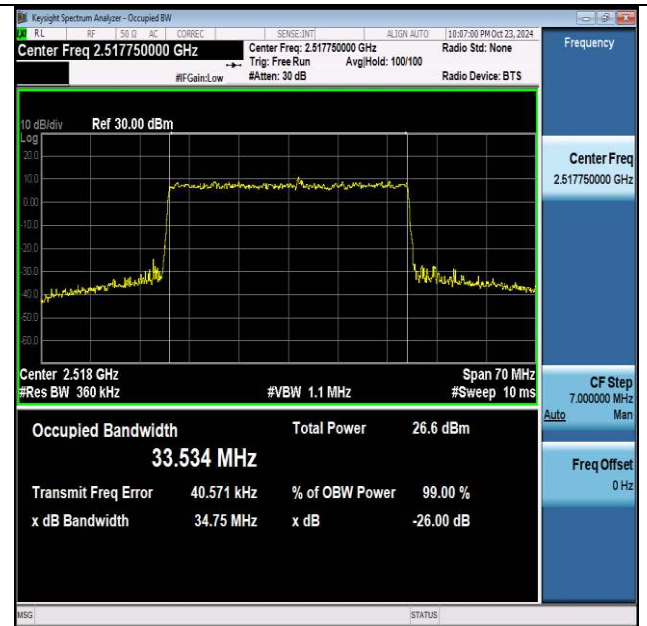
NTNV-n7-PC3-15-35-L-CP-256QAM-Outer_Full-Ant1-PASS
