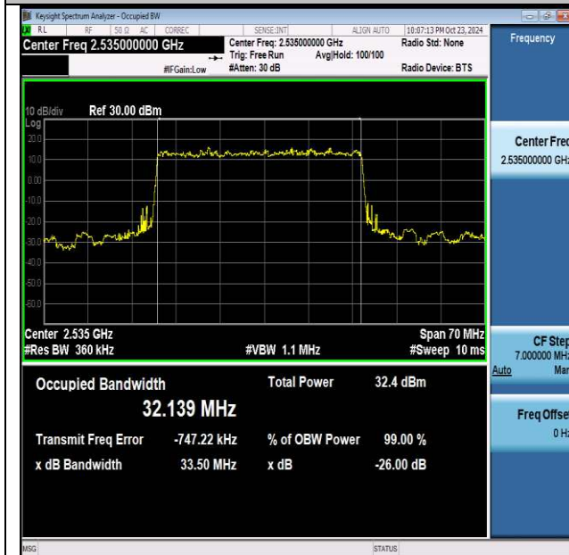
NTNV-n7-PC3-15-35-M-DFT-PI2BPSK-Outer_Full-Ant1-PASS
