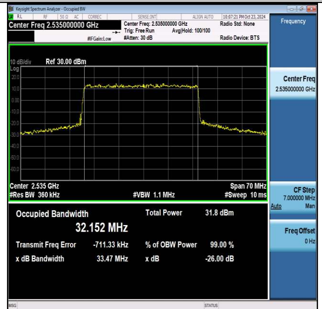
NTNV-n7-PC3-15-35-L-CP-256QAM-Outer_Full-Ant1-PASS
