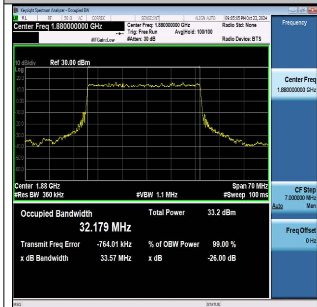
NTNV-n2-PC3-15-35-M-DFT-PI2BPSK-Outer_Full-Ant1-PASS
