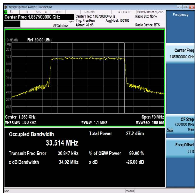
NTNV-n2-PC3-15-35-L-CP-256QAM-Outer_Full-Ant1-PASS
