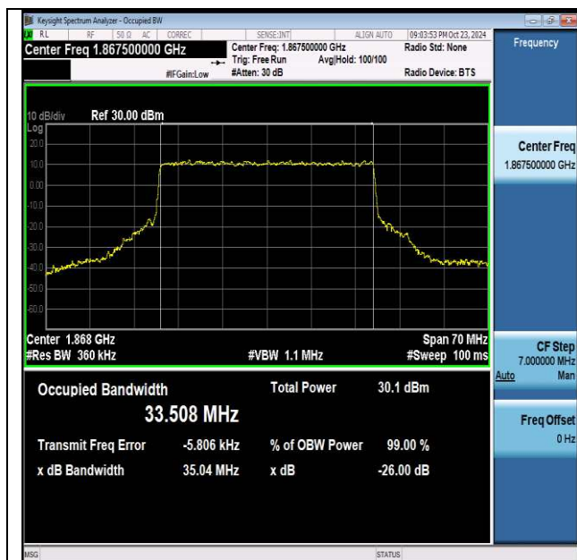
NTNV-n2-PC3-15-35-L-CP-64QAM-Outer_Full-Ant1-PASS
