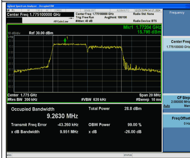
66-66-5MHz-5MHz-64QAM-64QAM-132599-132647-25RB#0-25RB#0-PASS
