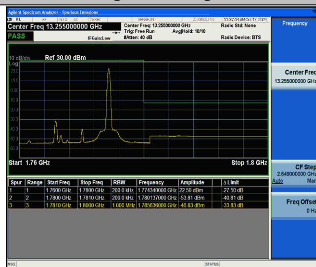
66-66-15MHz-5MHz-QPSK@QPSK-QPSK@QPSK-132549- 132642-1RB#74@75RB#0-0RB#0@25RB#0-PASS
