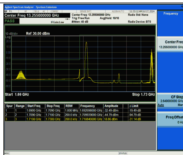
66-66-15MHz-5MHz-QPSK@QPSK-QPSK@QPSK-132047- 132140-1RB#0@75RB#0-1RB#24@25RB#0-PASS
