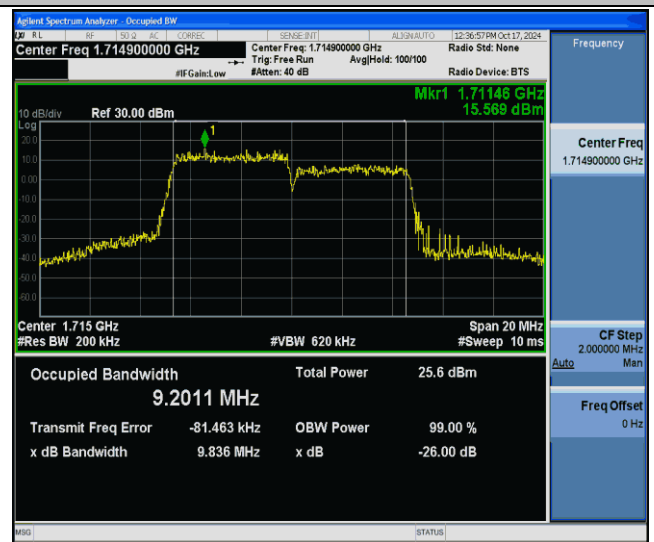
66-66-5MHz-5MHz-256QAM-256QAM-131997-132045-25RB#0-25RB#0-PASS
