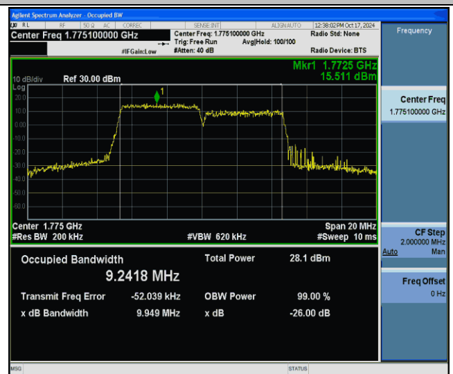
66-66-5MHz-5MHz-256QAM-256QAM-132599-132647-25RB#0-25RB#0-PASS
