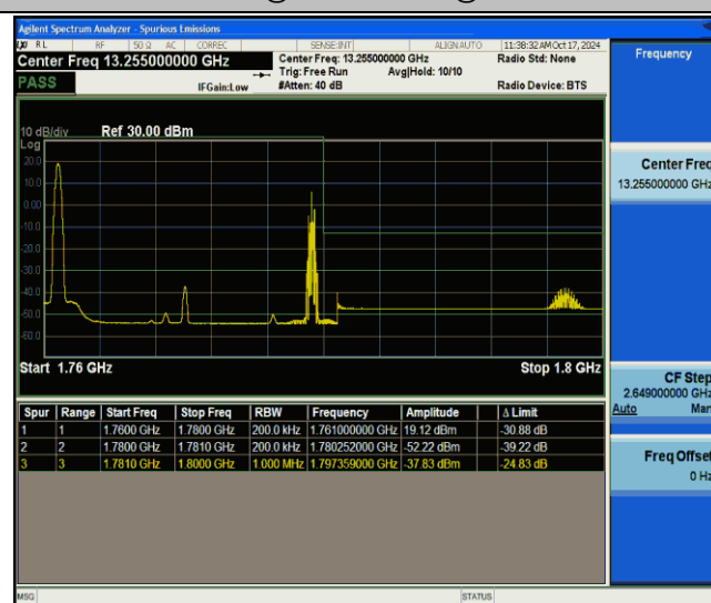
66-66-15MHz-5MHz-QPSK@QPSK-QPSK@QPSK-132549- 132642-1RB#0@75RB#0-1RB#24@25RB#0-PASS
