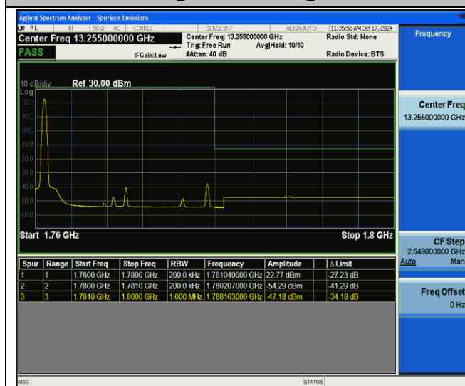
66-66-15MHz-5MHz-QPSK@QPSK-QPSK@QPSK-132549- 132642-1RB#0@75RB#0-0RB#0@25RB#0-PASS
