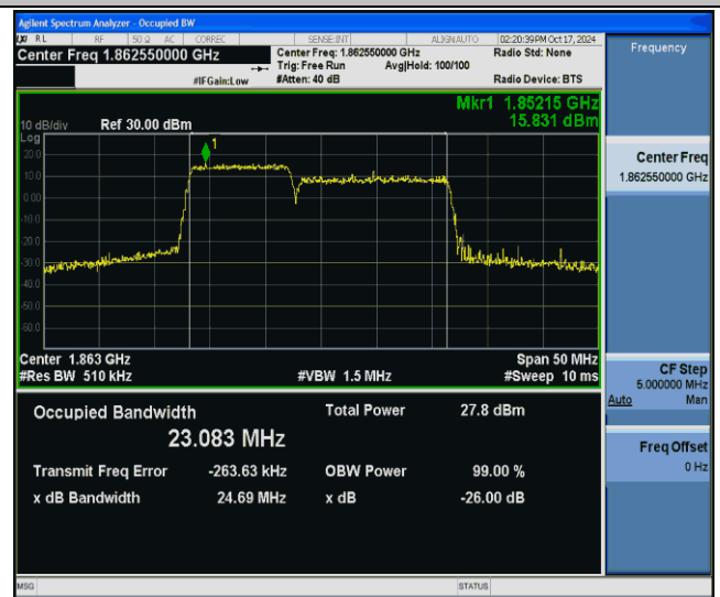
2-2-10MHz-15MHz-256QAM-256QAM-18653-18773-50RB#0- 75RB#0-PASS
