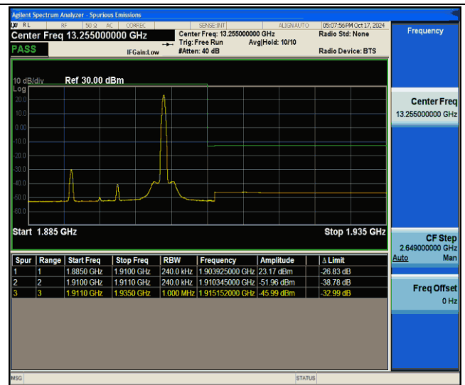
2-2-20MHz-5MHz-QPSK@QPSK-QPSK-19050-19167-1RB#99@100RB#0-0RB#0@25RB#0-PASS
