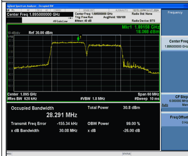
2-2-15MHz-15MHz-64QAM-64QAM-18975-19125-75RB#0-75RB#0-PASS
