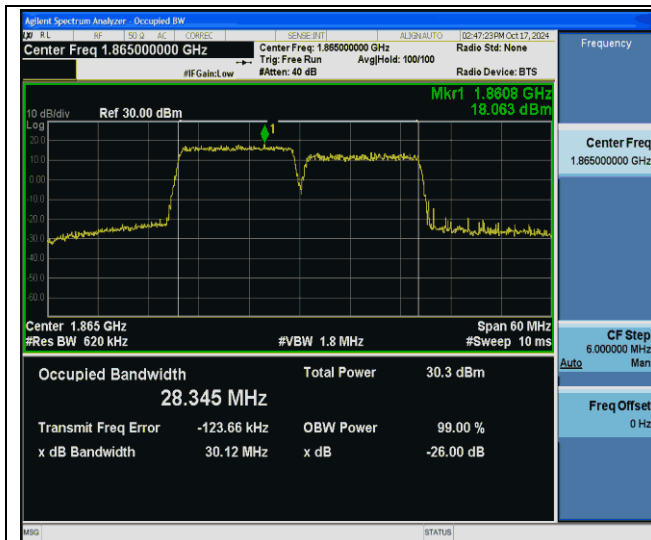
2-2-15MHz-15MHz-64QAM-64QAM-18675-18825-75RB#0-75RB#0-PASS
