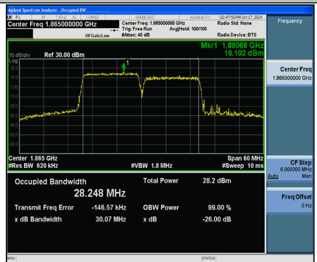
2-2-15MHz-15MHz-256QAM-256QAM-18675-18825-75RB#0-75RB#0-PASS
