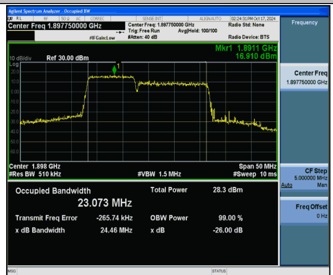
2-2-10MHz-15MHz-256QAM-256QAM-19005-19125-50RB#0- 75RB#0-PASS
