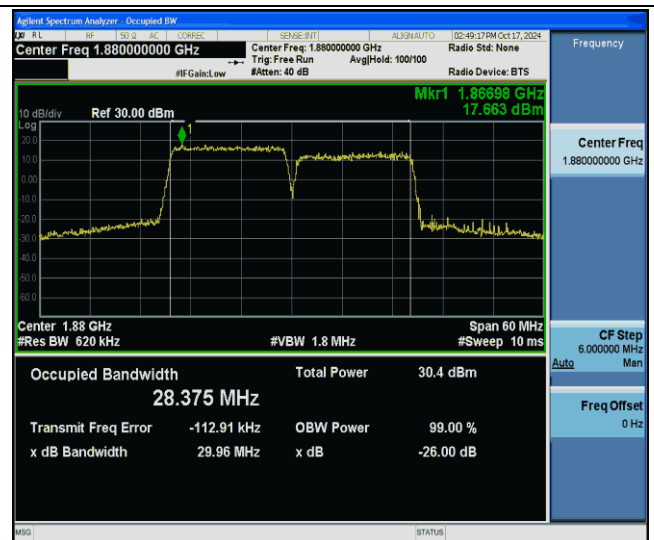
2-2-15MHz-15MHz-64QAM-64QAM-18825-18975-75RB#0-75RB#0-PASS
