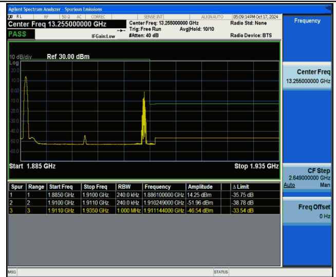
2-2-20MHz-5MHz-QPSK@QPSK-QPSK-19050-19167-1RB#0@100RB#0-1RB#24@25RB#0-PASS
