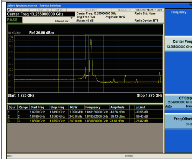
2-2-15MHz-10MHz-QPSK@QPSK-QPSK-18675-18795-1RB#0@75RB#0-0RB#0@50RB#0-PASS
