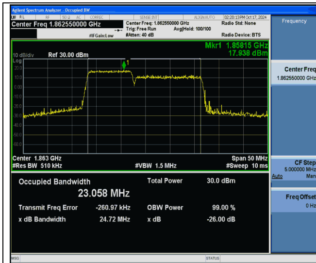
2-2-10MHz-15MHz-64QAM-64QAM-18653-18773-50RB#0- 75RB#0-PASS
