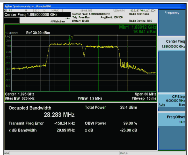
2-2-15MHz-15MHz-256QAM-256QAM-18975-19125-75RB#0-75RB#0-PASS
