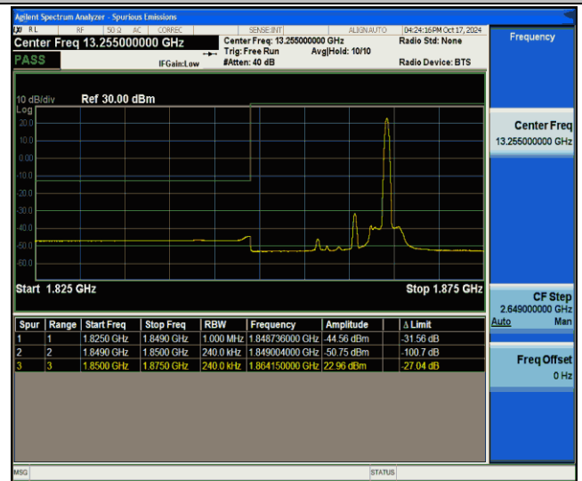
2-2-15MHz-10MHz-QPSK@QPSK-QPSK-18675-18795-1RB#74@75RB#0-0RB#0@50RB#0-PASS
