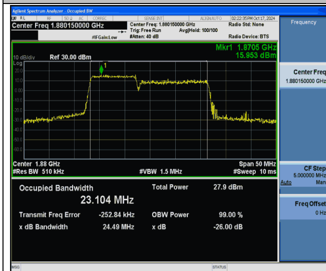
2-2-10MHz-15MHz-256QAM-256QAM-18829-18949-50RB#0- 75RB#0-PASS
