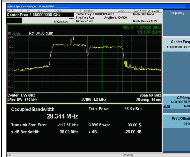
2-2-15MHz-15MHz-256QAM-256QAM-18825-18975-75RB#0-75RB#0-PASS
