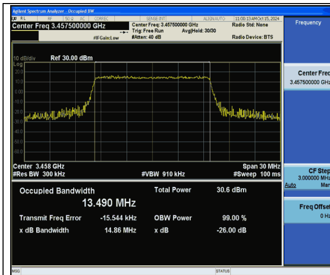
Band42(3450-3550)-15MHz-64QAM-42165-75RB#0-PASS
