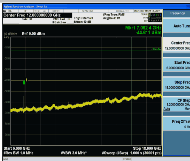
Band42(3450-3550)-20MHz-QPSK-42990-1RB#0-6000~18000-PASS
