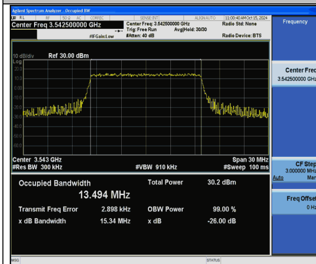
Band42(3450-3550)-15MHz-64QAM-43015-75RB#0-PASS
