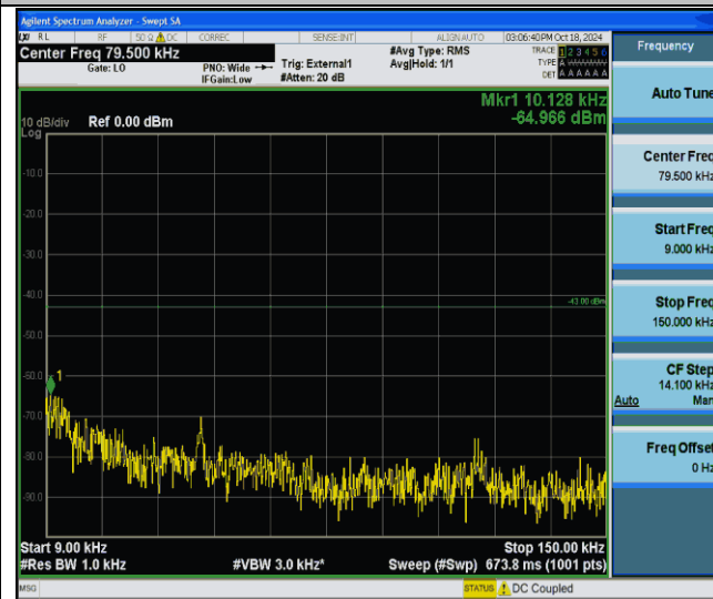
Band42(3450-3550)-20MHz-QPSK-42590-1RB#0-0.009~0.15-
