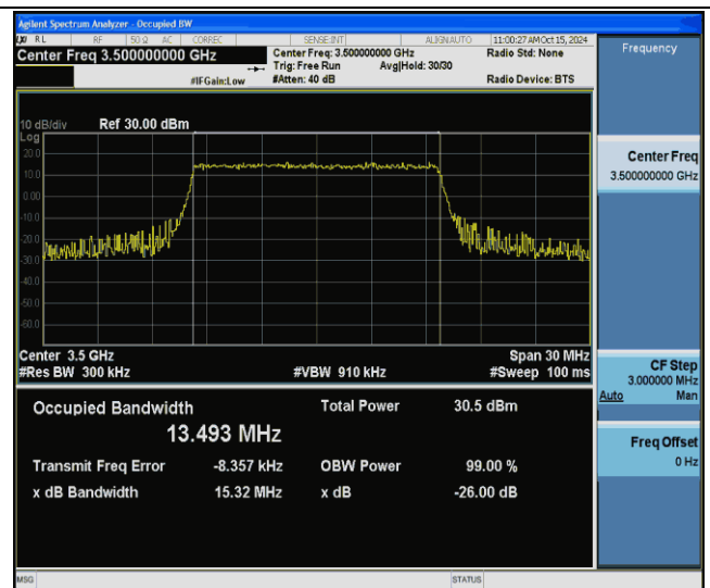
Band42(3450-3550)-15MHz-64QAM-42590-75RB#0-PASS
