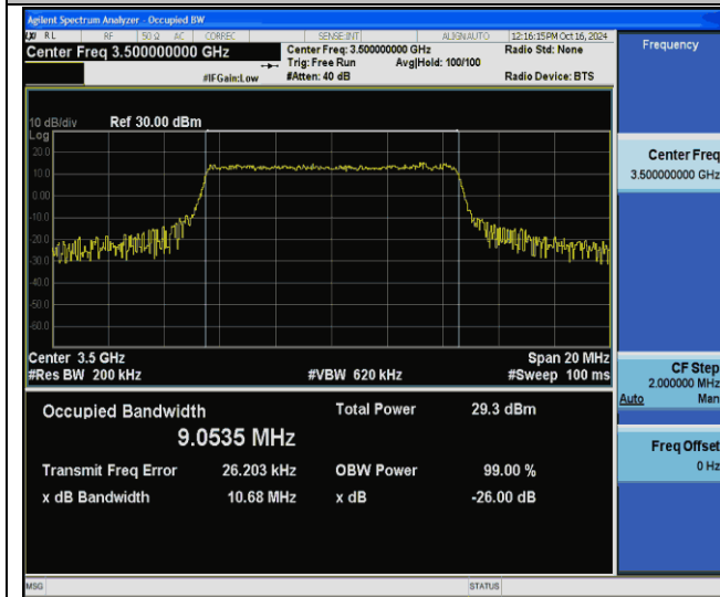
Band42(3450-3550)-10MHz-256QAM-42590-50RB#0-PASS
