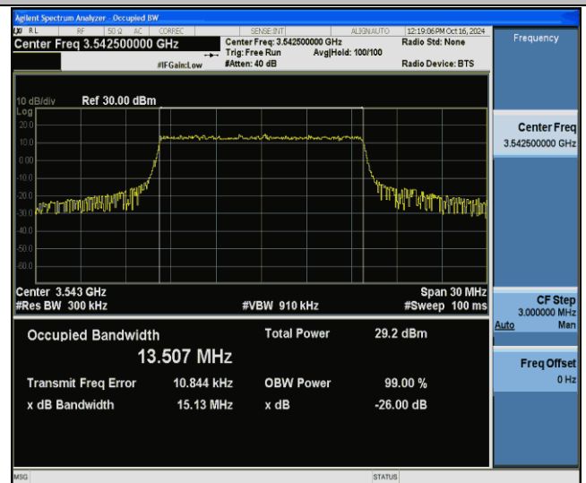
Band42(3450-3550)-15MHz-256QAM-43015-75RB#0-PASS
