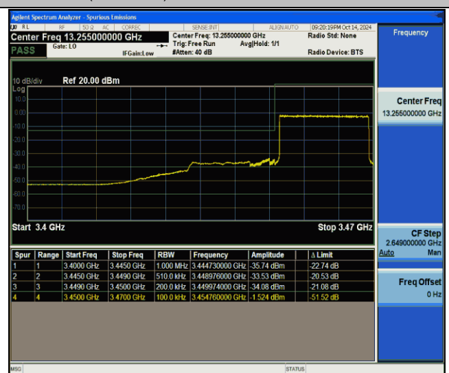
Band42(3450-3550)-20MHz-QPSK-42190-100RB#0-PASS
