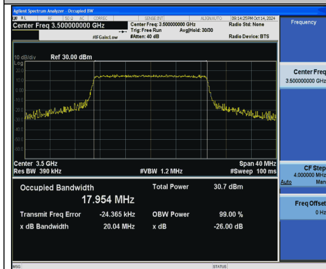
Band42(3450-3550)-20MHz-16QAM-42590-100RB#0-PASS
