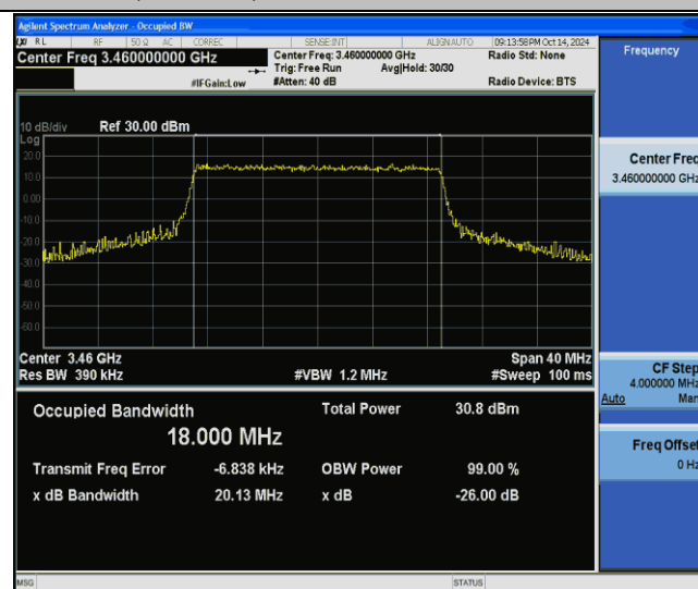
Band42(3450-3550)-20MHz-16QAM-42190-100RB#0-PASS
