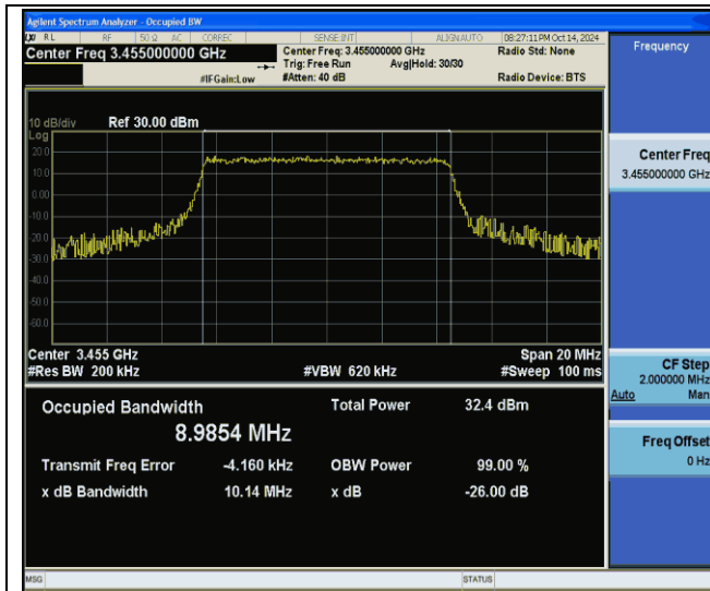
Band42(3450-3550)-10MHz-QPSK-42140-50RB#0-PASS
