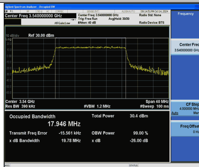
Band42(3450-3550)-20MHz-16QAM-42990-100RB#0-PASS
