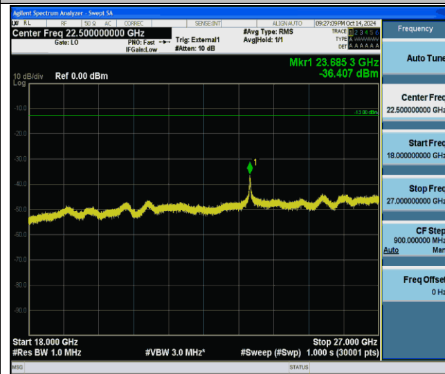
Band42(3450-3550)-20MHz-QPSK-42190-1RB#0-18000~27000-
