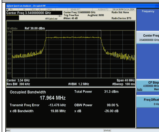
Band42(3450-3550)-20MHz-QPSK-42990-100RB#0-PASS
