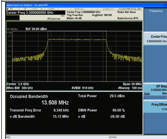
Band42(3450-3550)-15MHz-256QAM-42590-75RB#0-PASS
