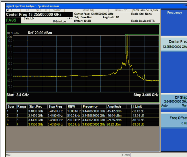
Band42(3450-3550)-15MHz-QPSK-42165-1RB#0-PASS
