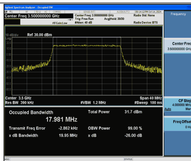
Band42(3450-3550)-20MHz-QPSK-42590-100RB#0-PASS
