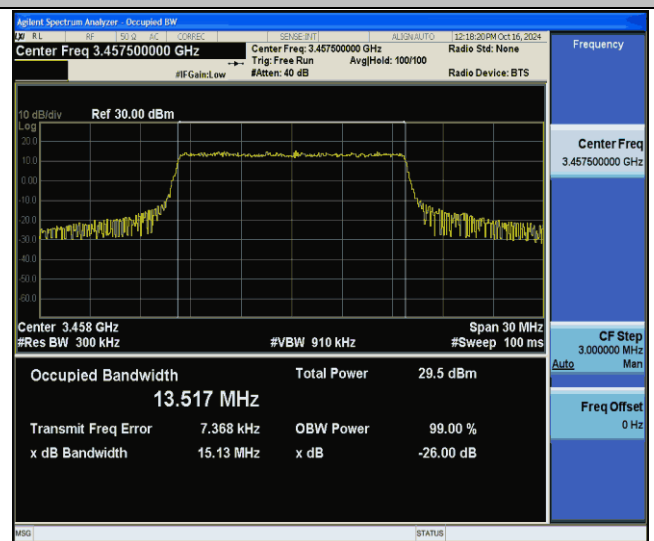
Band42(3450-3550)-15MHz-256QAM-42165-75RB#0-PASS
