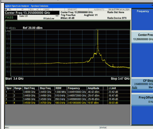
Band42(3450-3550)-20MHz-QPSK-42190-1RB#0-PASS
