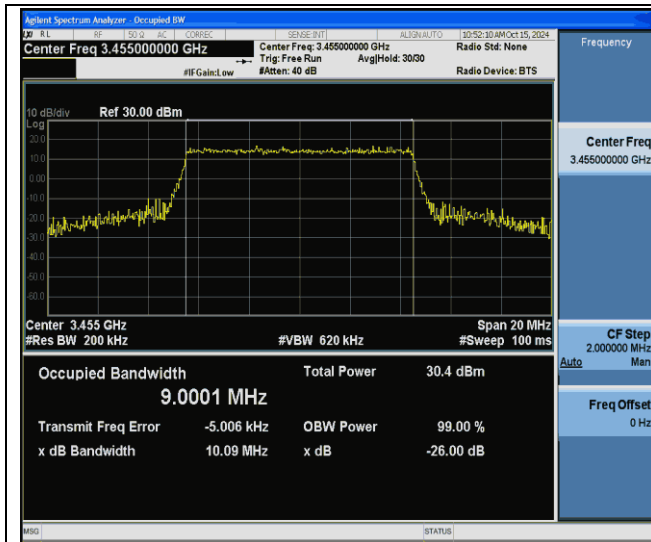
Band42(3450-3550)-10MHz-64QAM-42140-50RB#0-PASS
