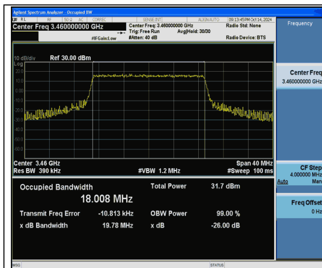
Band42(3450-3550)-20MHz-QPSK-42190-100RB#0-PASS
