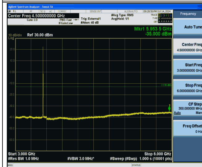
Band42(3450-3550)-20MHz-QPSK-42990-1RB#0-3000~6000-PASS
