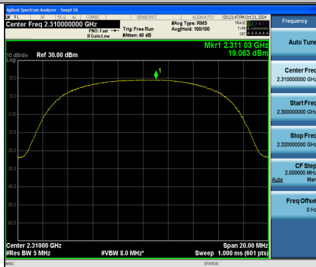
Band30-10MHz-QPSK-27710-50RB#0-PASS
