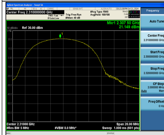
Band30-10MHz-QPSK-27710-25RB#0-PASS
