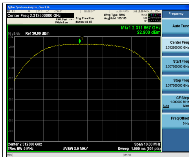
Band30-5MHz-QPSK-27735-1RB#12-PASS
